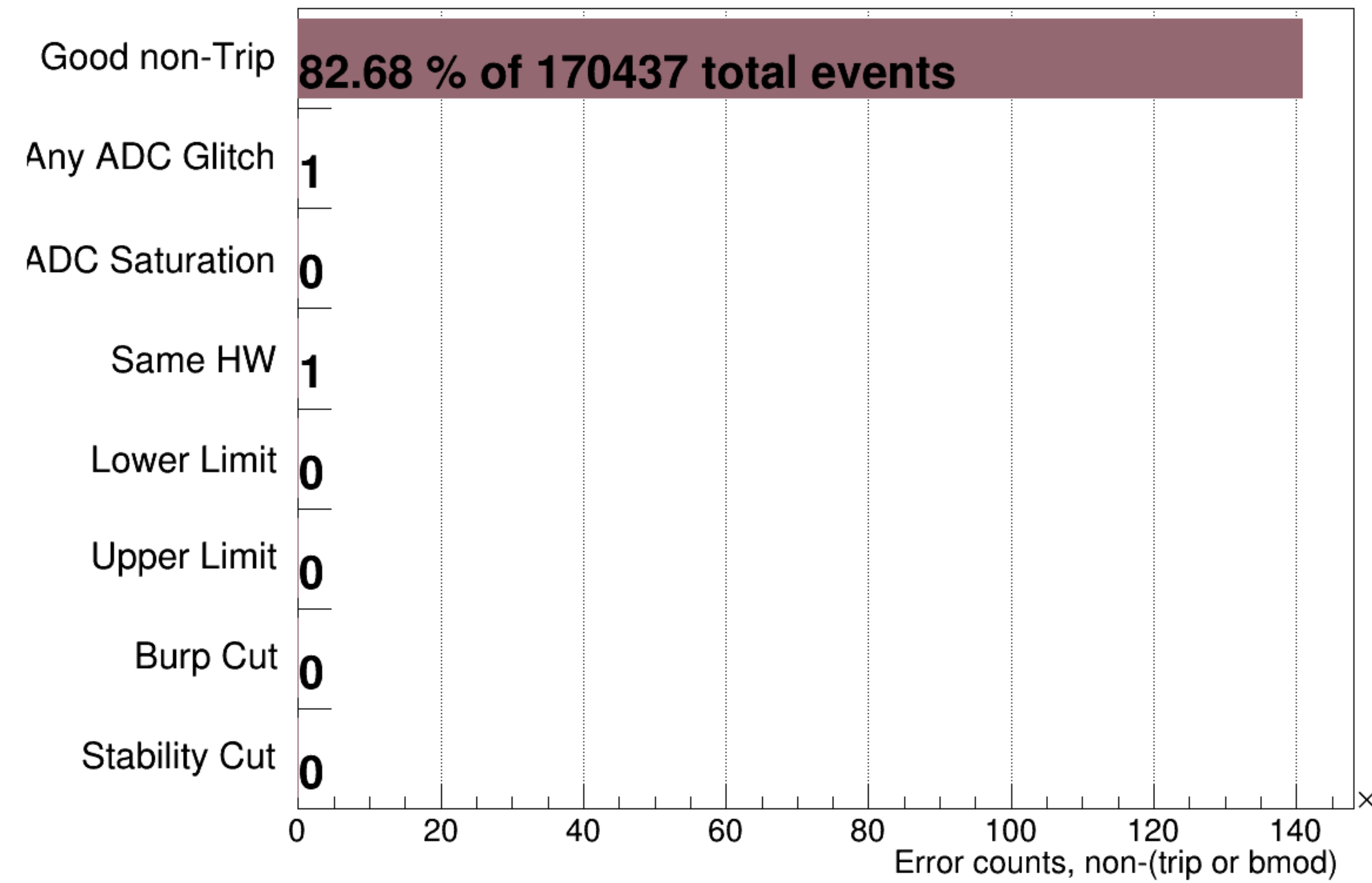
atl1's Device Error Counter &amp;&amp; Not (Trip || BMOD)
