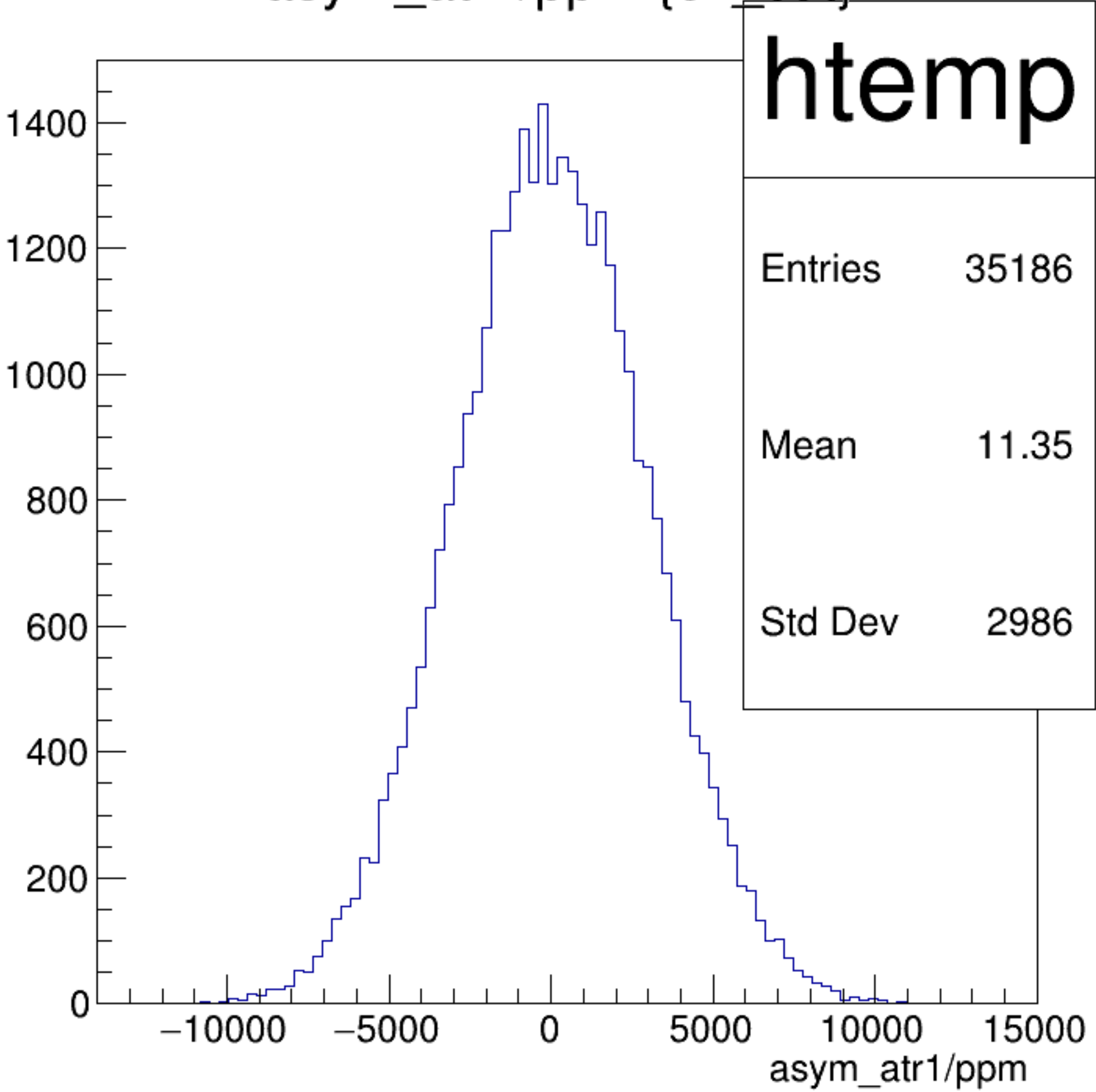
asym_atr1/ppm {ok_cut}
