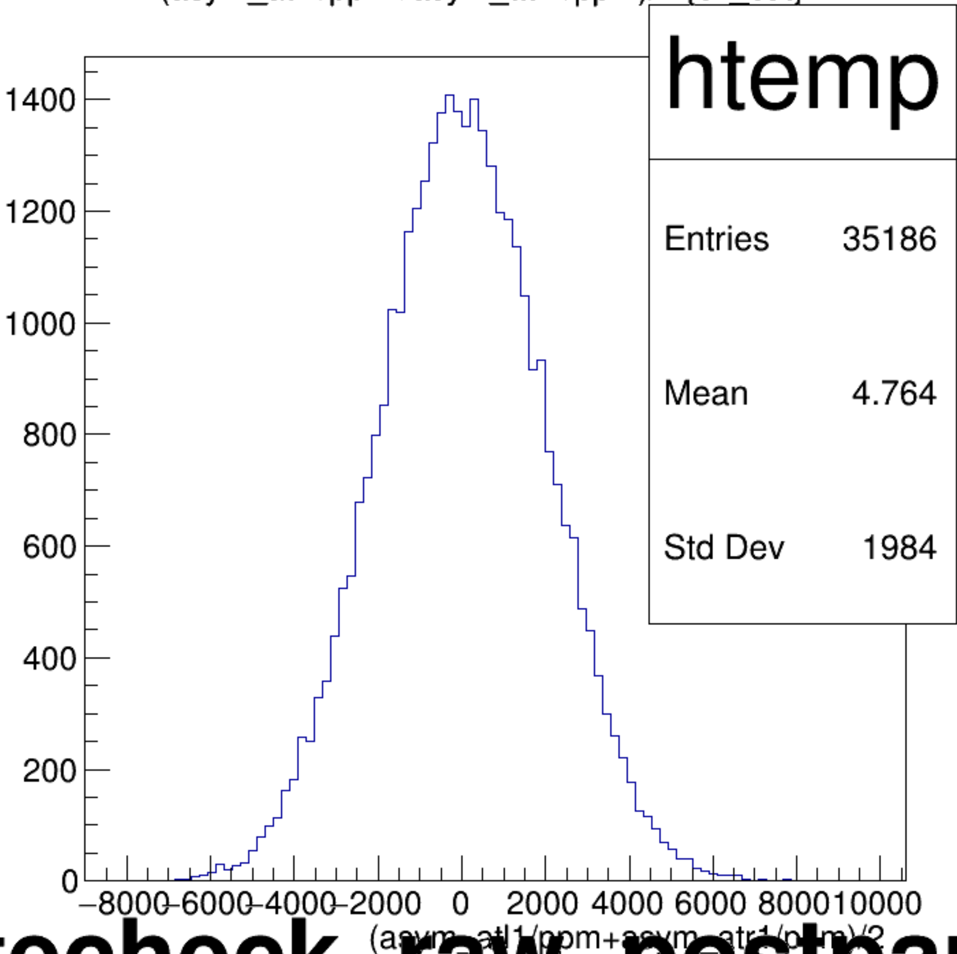
(asym_atl1/ppm+asym_atr1/ppm)/2 {ok_cut}
