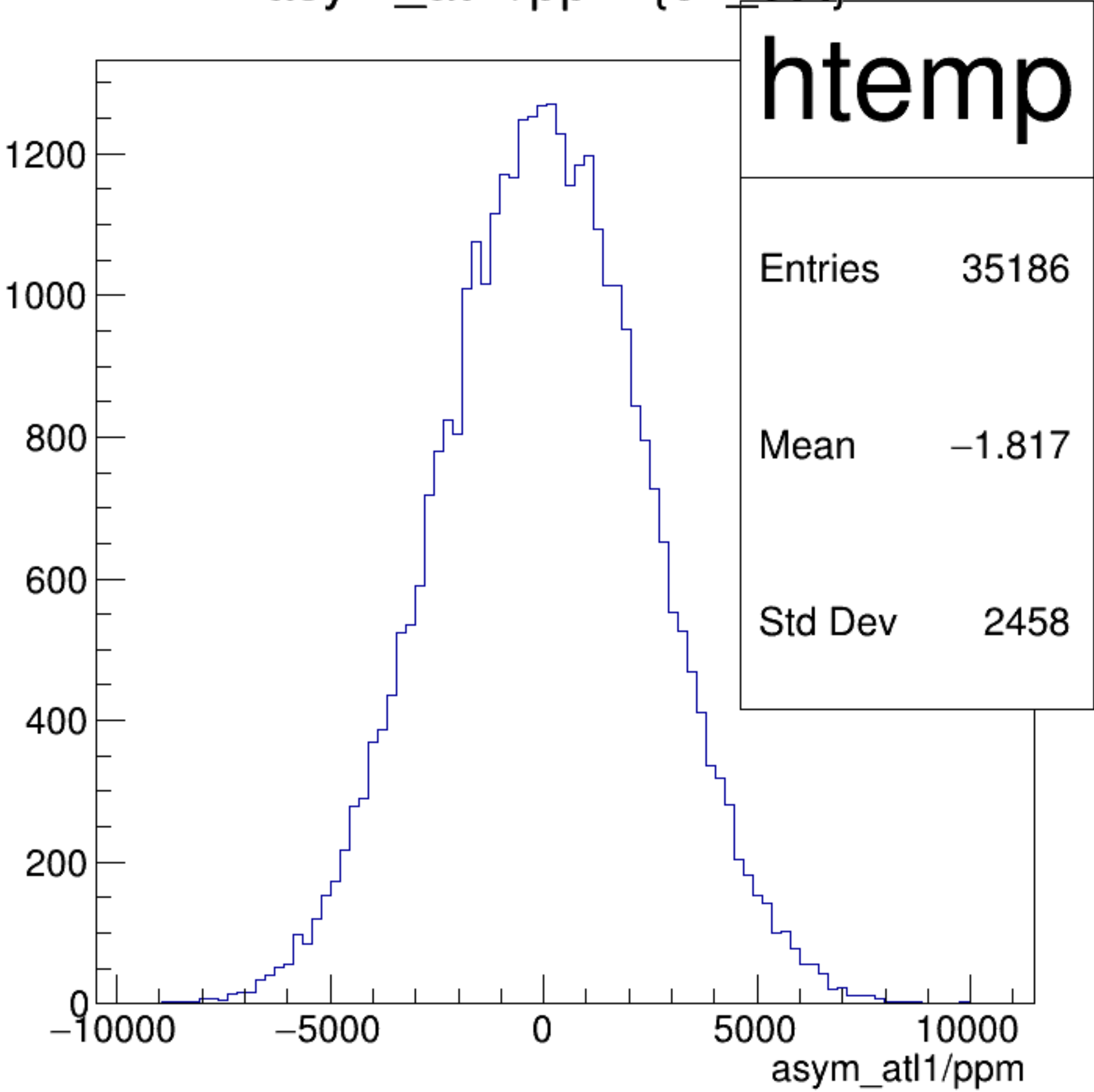
asym_atl1/ppm {ok_cut}
