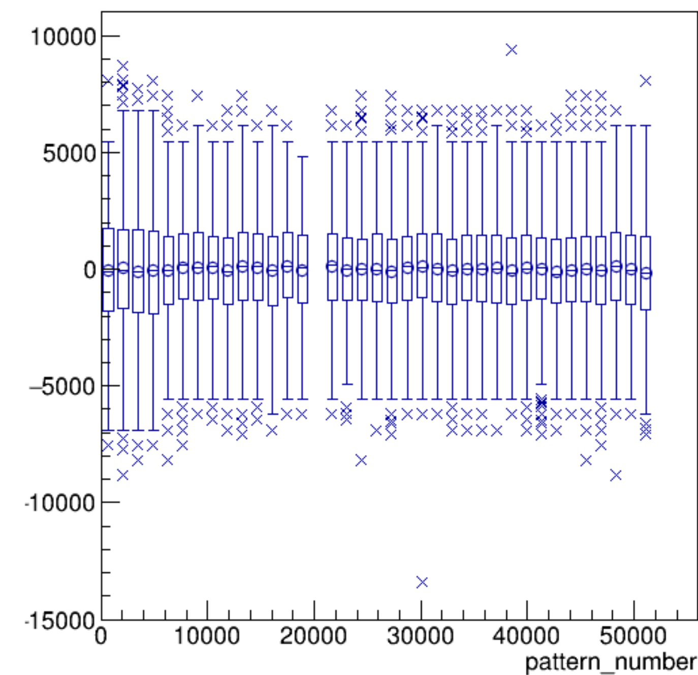
asym_atl1/ppm:pattern_number {ErrorFlag==0}
