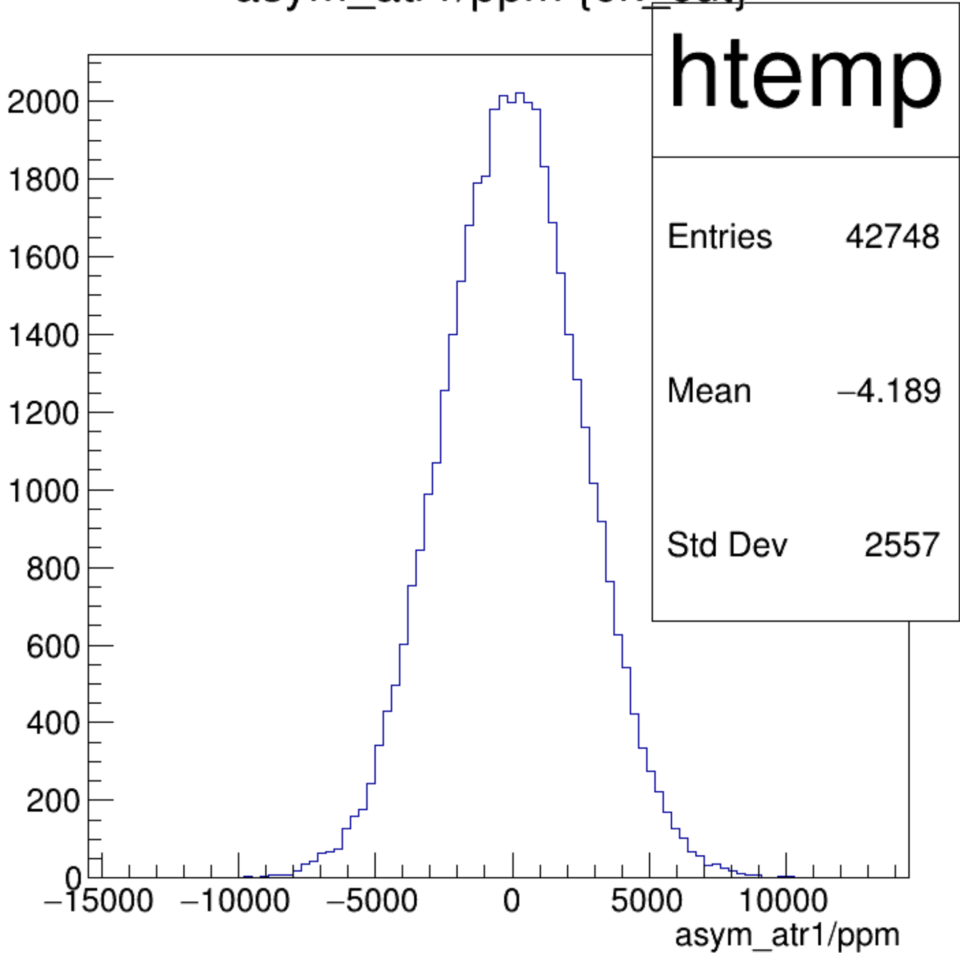
asym_atr1/ppm {ok_cut}
