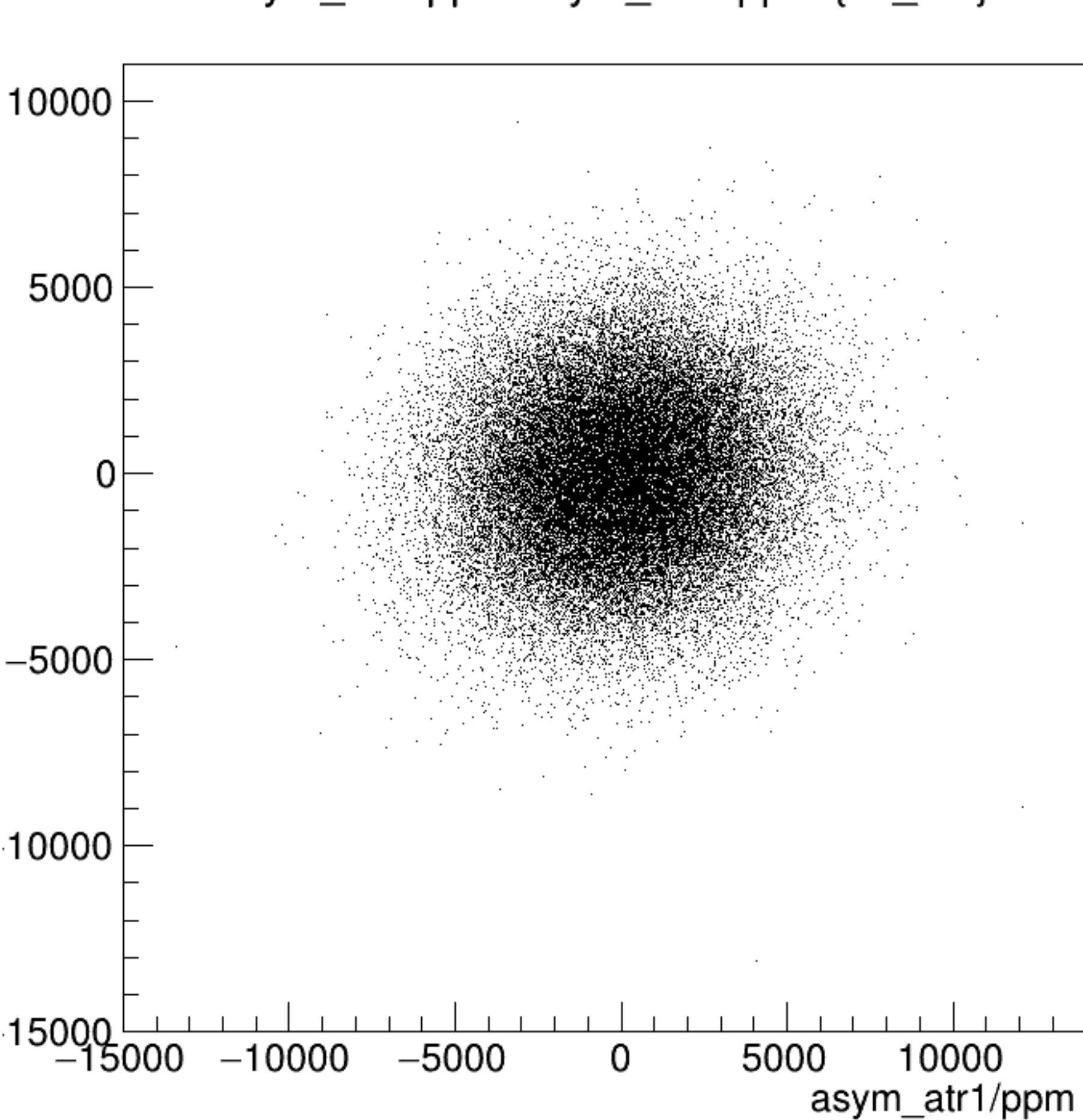
asym_atl1/ppm:asym_atr1/ppm {ok_cut}
