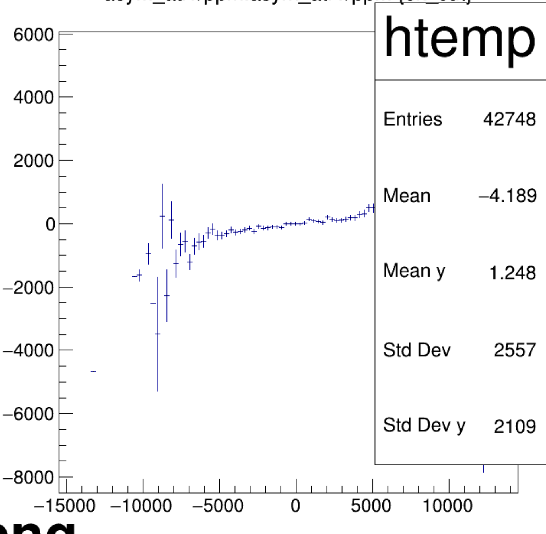
asym_atl1/ppm:asym_atr1/ppm {ok_cut}
