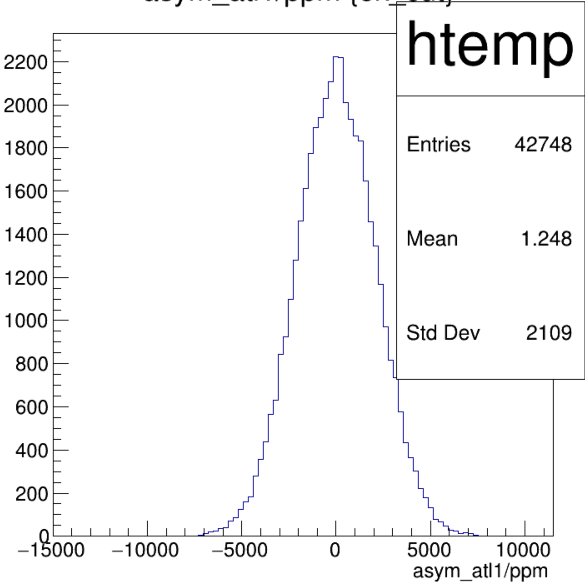
asym_atl1/ppm {ok_cut}
