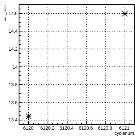
usr_4eY:cyclenum {run == 6387}
