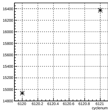
usr_coil7:cyclenum {run == 6387}
