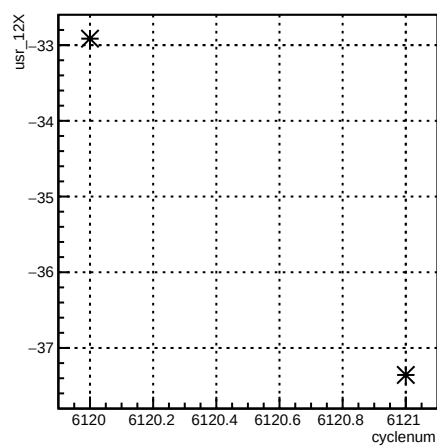
usr_12X:cyclenum {run == 6387}
