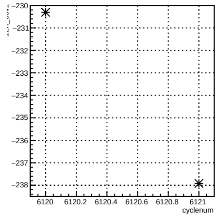
12X_coil1:cyclenum {run == 6387}
