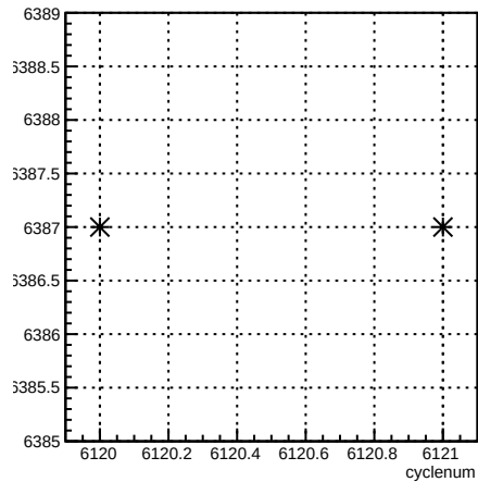
run:cyclenum {run == 6387}
