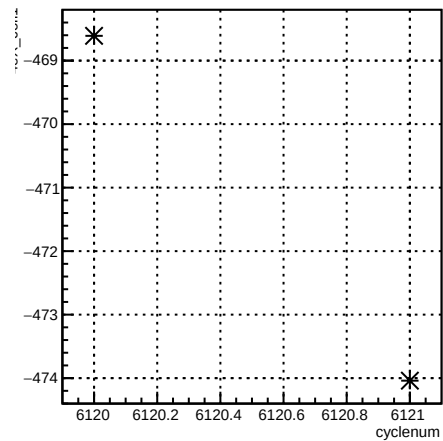
4eX_coil1:cyclenum {run == 6387}
