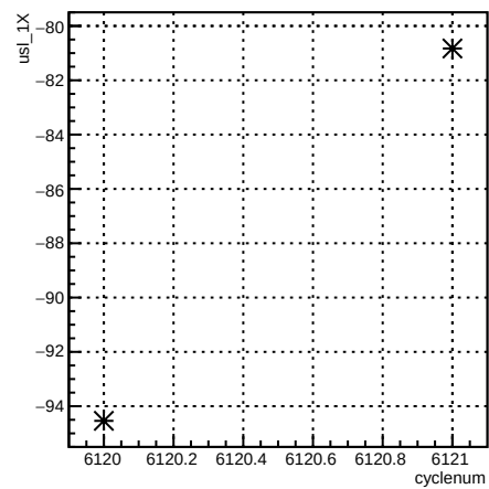
usl_1X:cyclenum {run == 6387}
