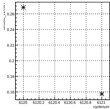
delta46_12X4eY:cyclenum {run == 6387}
