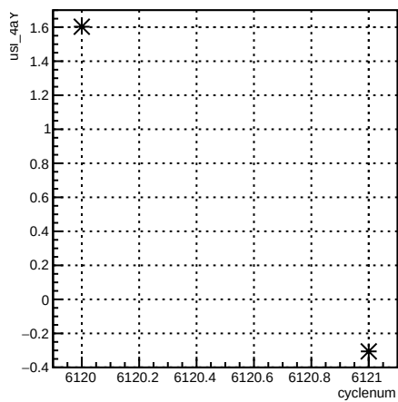
usl_4aY:cyclenum {run == 6387}
