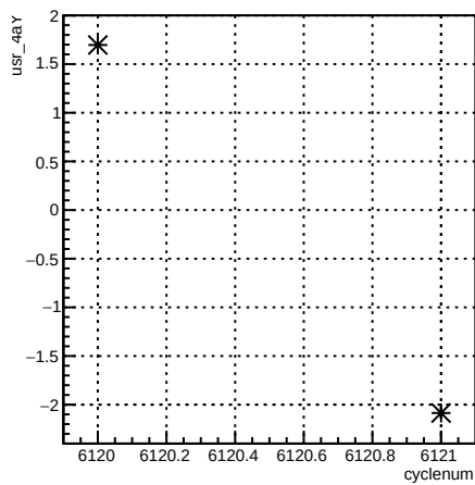
usr_4aY:cyclenum {run == 6387}
