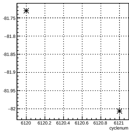
12X_coil3:cyclenum {run == 6387}
