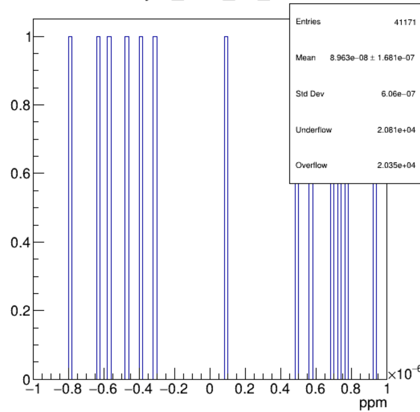
asym_bcm_an_diff
