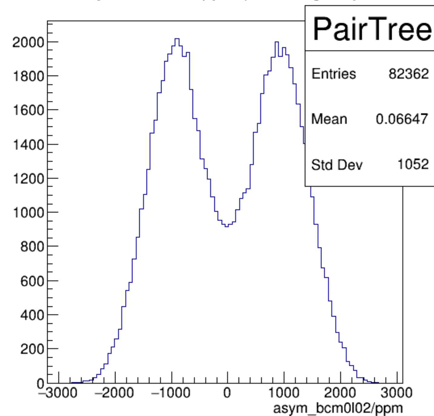
asym_bcm0l02/ppm {ErrorFlag==0}
