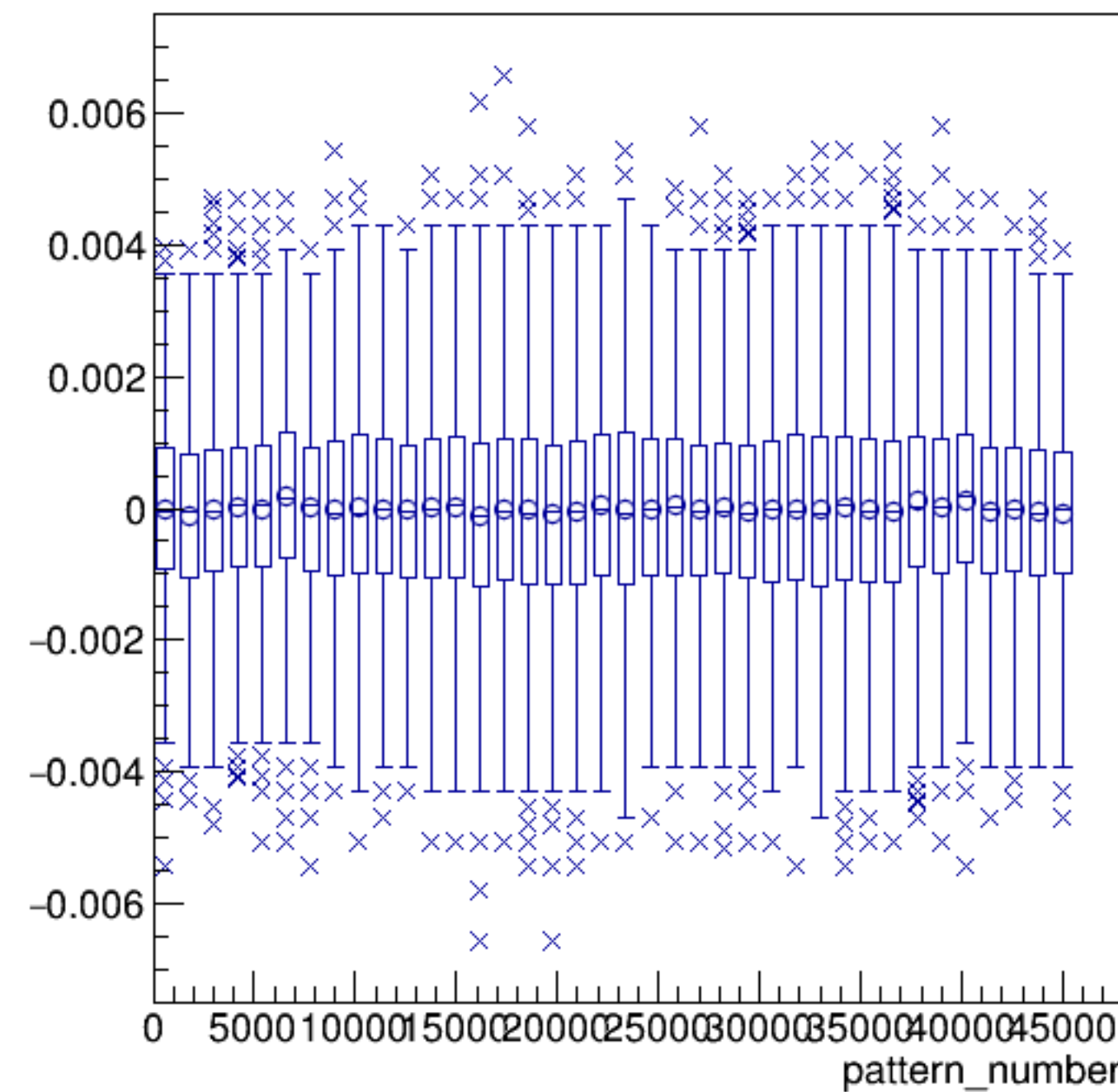
asym_bcm_an_diff*yield_bcm_an_diff:pattern_number {ErrorFlag==0}
