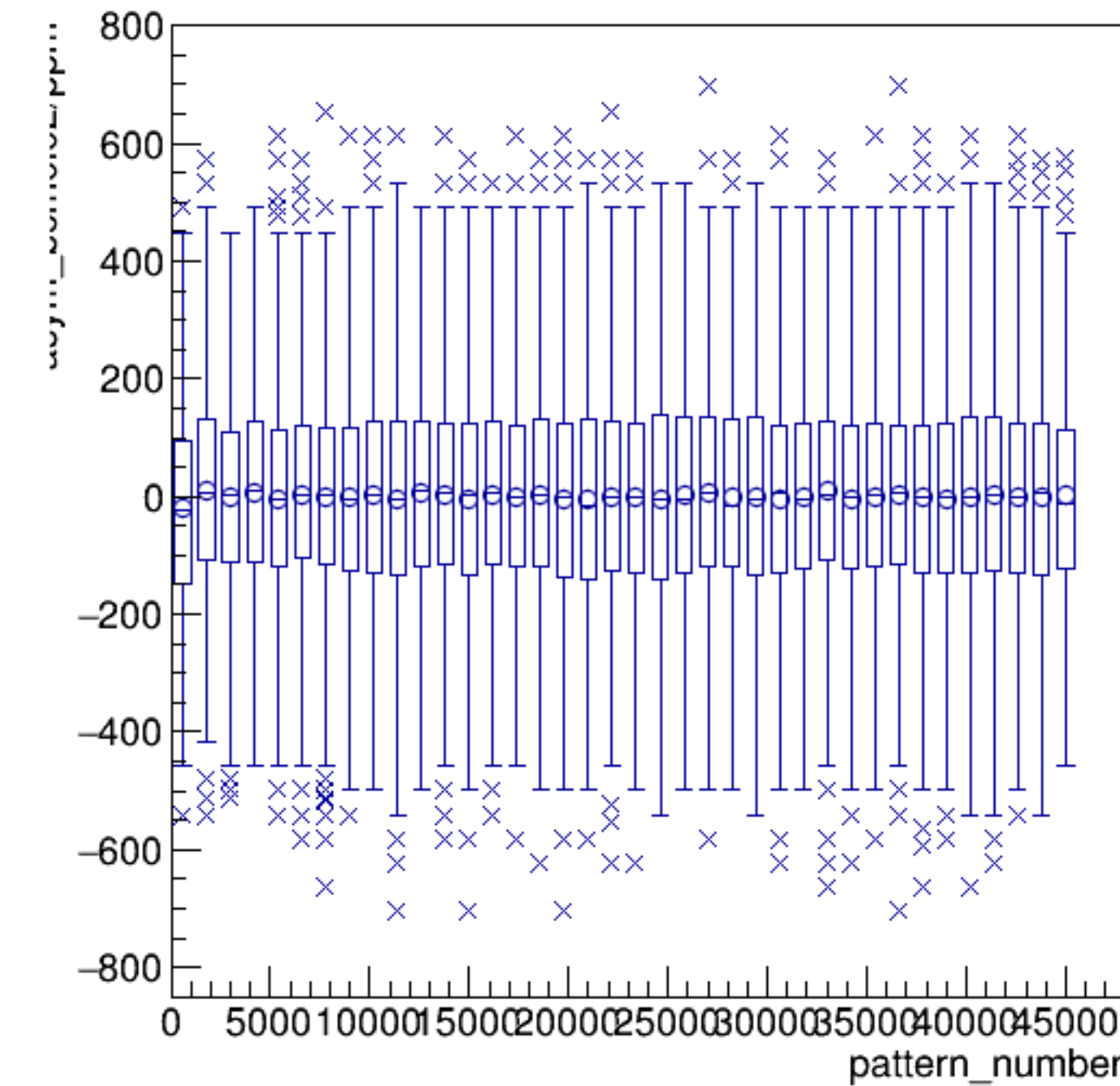
asym_bcm0l02/ppm:pattern_number {ErrorFlag==0}
