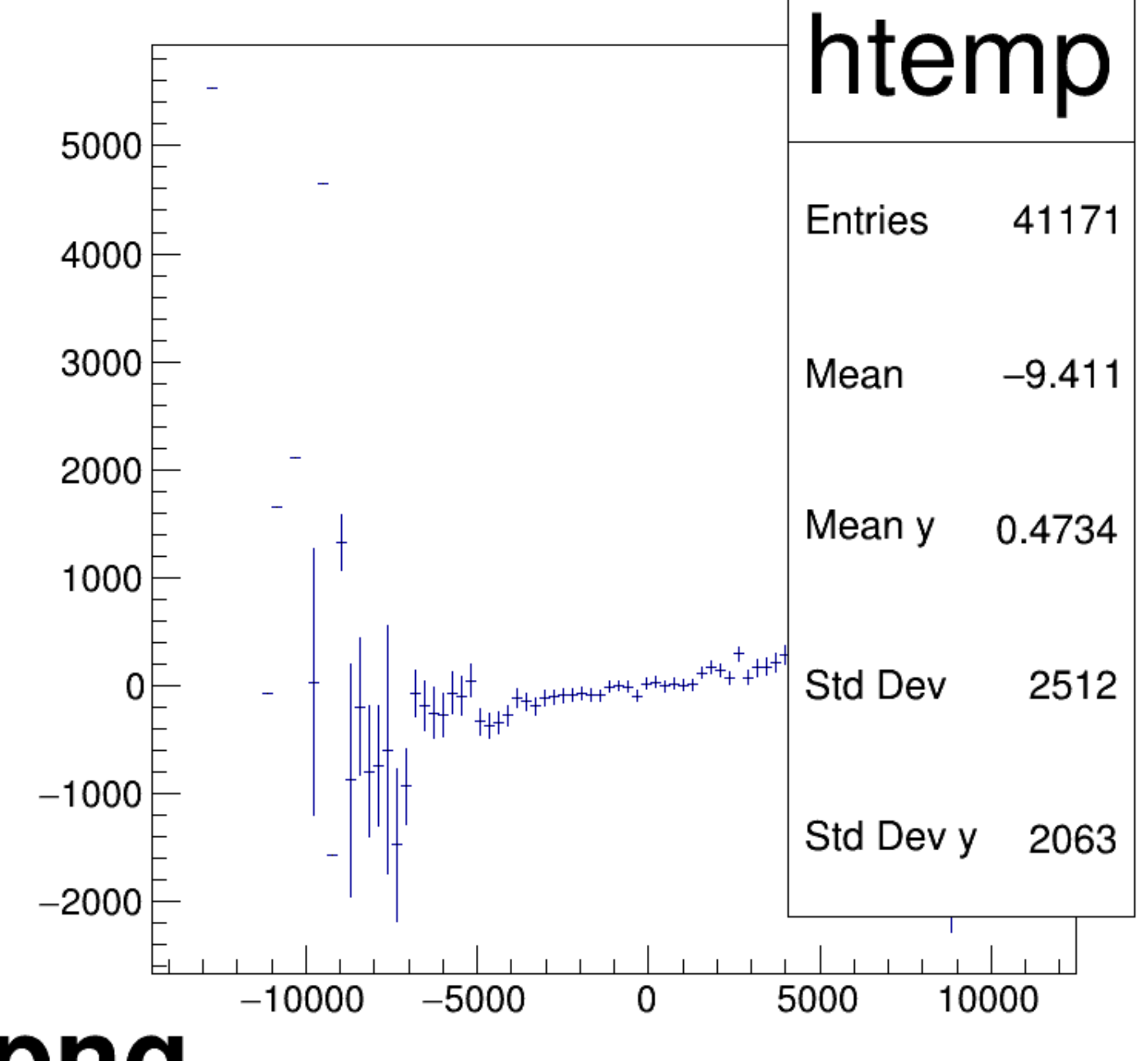
asym_atl1/ppm:asym_atr1/ppm {ok_cut}
