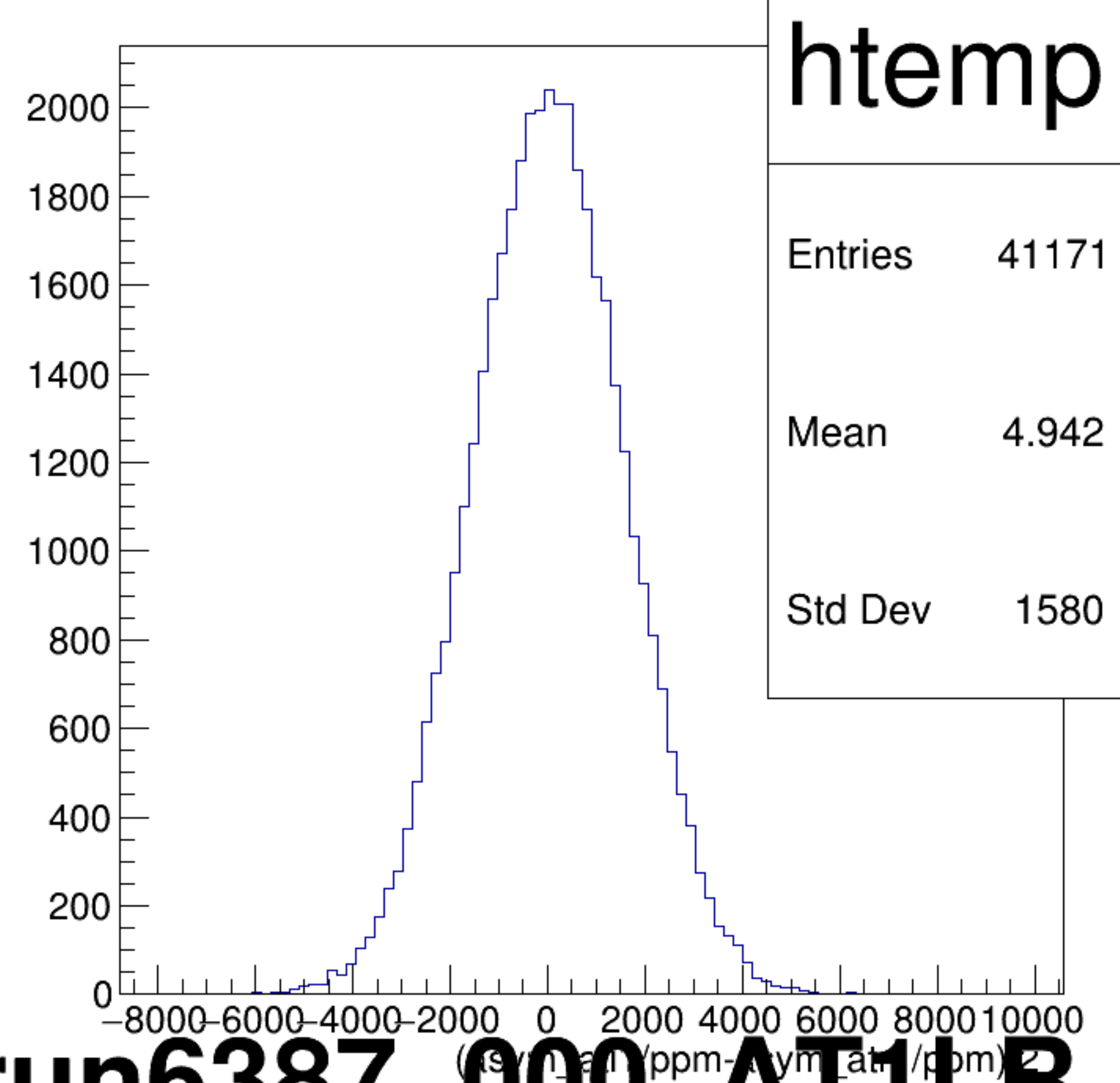
(asym_atl1/ppm-asym_atr1/ppm)/2 {ok_cut}
