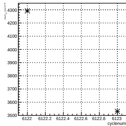
usl_coil4:cyclenum {run == 6388}
