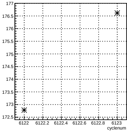
4aY_coil4:cyclenum {run == 6388}
