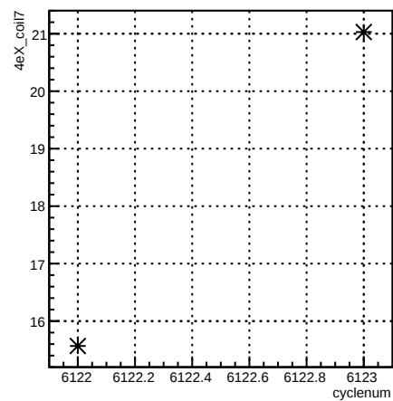
4eX_coil7:cyclenum {run == 6388}
