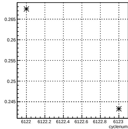
delta46_12X4eY:cyclenum {run == 6388}
