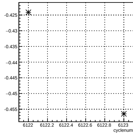
delta13_12X4eX:cyclenum {run == 6388}
