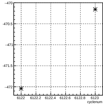
4eX_coil1:cyclenum {run == 6388}
