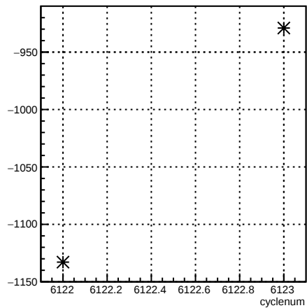
usl_coil6:cyclenum {run == 6388}
