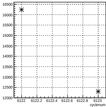
usl_coil7:cyclenum {run == 6388}
