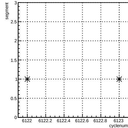
segment:cyclenum {run == 6388}
