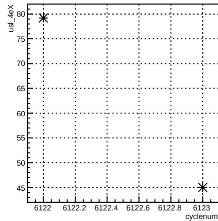
run:cyclenum {run == 6388}
