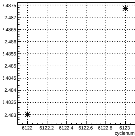
alpha46_4eY4aY:cyclenum {run == 6388}
