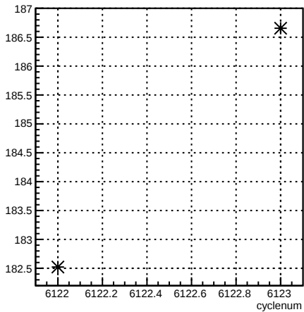
4eY_coil4:cyclenum {run == 6388}
