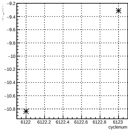
4aY_coil7:cyclenum {run == 6388}
