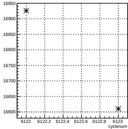
usl_coil1:cyclenum {run == 6388}
