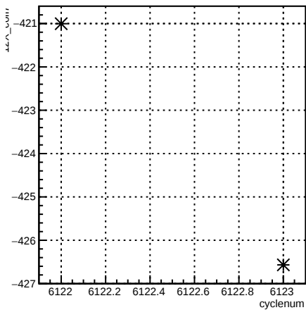
12X_coil7:cyclenum {run == 6388}
