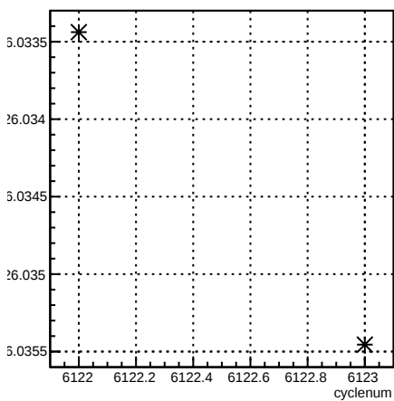
4eY_coil6:cyclenum {run == 6388}
