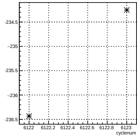
12X_coil6:cyclenum {run == 6388}
