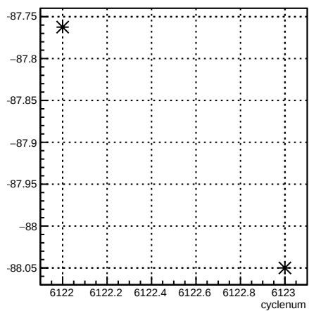
4eX_coil3:cyclenum {run == 6388}
