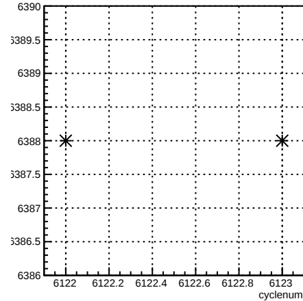
run:cyclenum {run == 6388}
