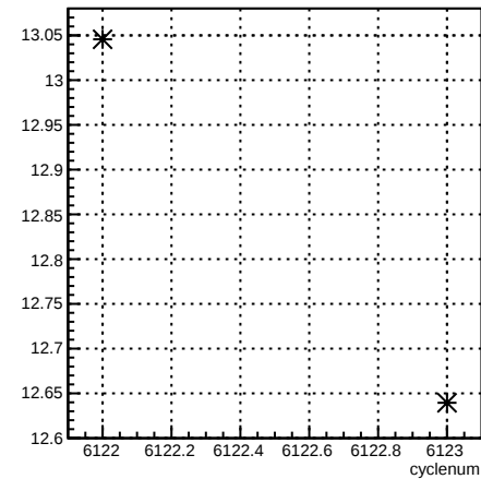
usr_4eY:cyclenum {run == 6388}
