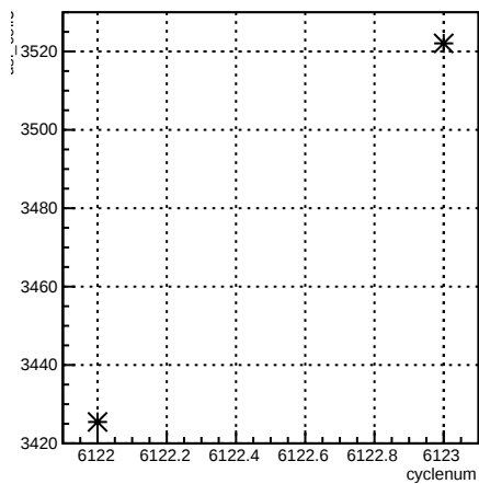
usl_coil3:cyclenum {run == 6388}
