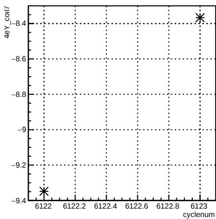
4eY_coil7:cyclenum {run == 6388}
