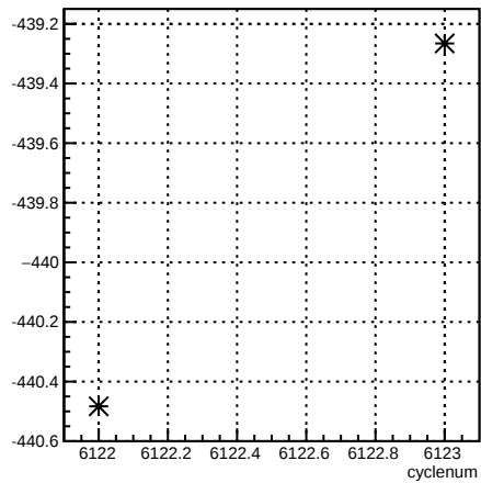
4eX_coil1:cyclenum {run == 6388}
