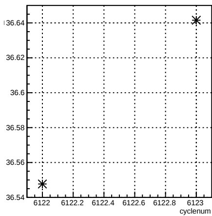
4aY_coil6:cyclenum {run == 6388}
