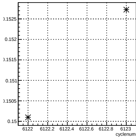
alpha13_4eX1X:cyclenum {run == 6388}
