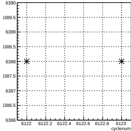
run:cyclenum {run == 6388}
