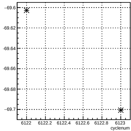
4eX_coil3:cyclenum {run == 6388}
