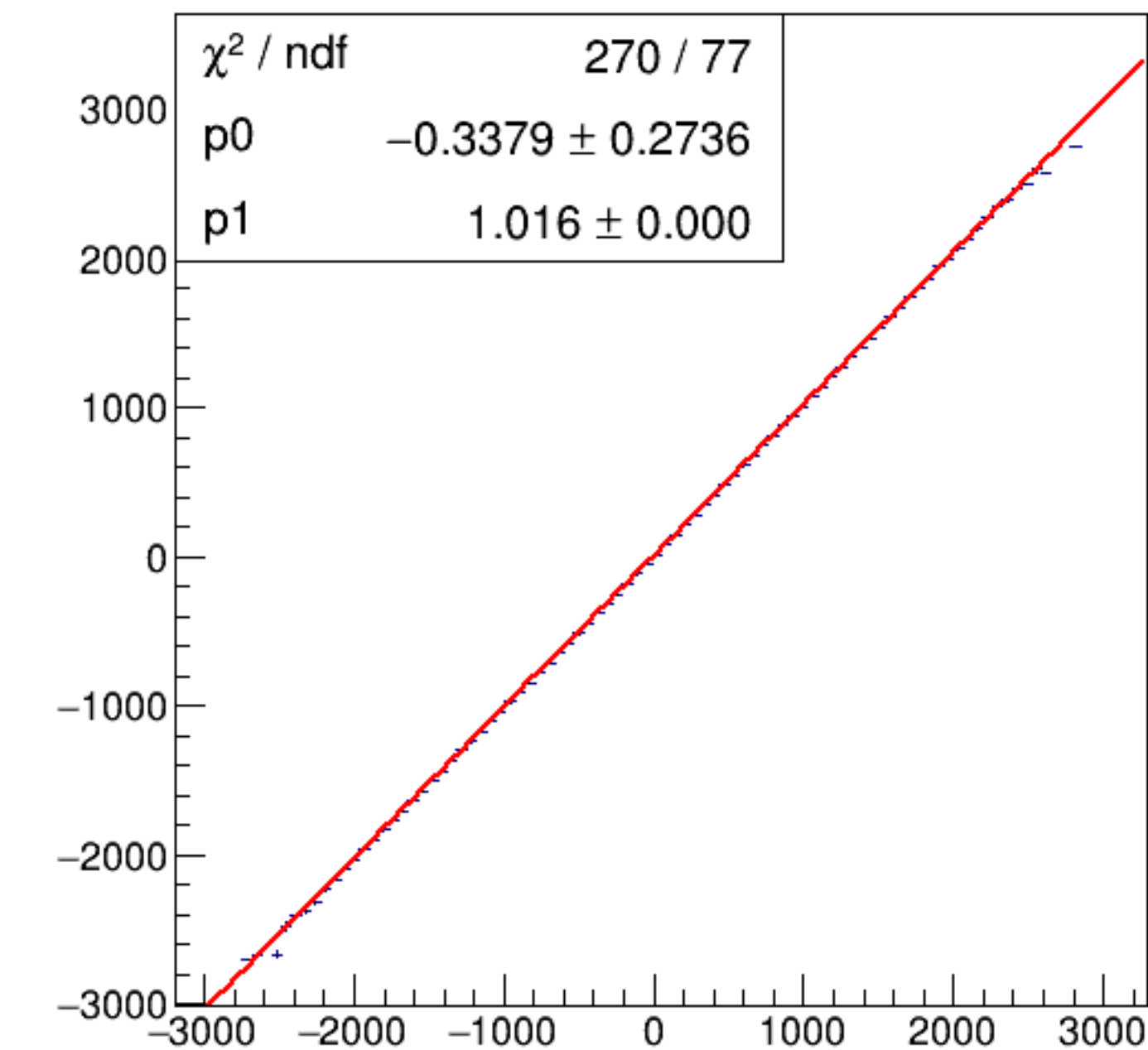
run6388_000_asym_bcm_dg_us_vs_asym_bcm_an_ds3_pr.png
