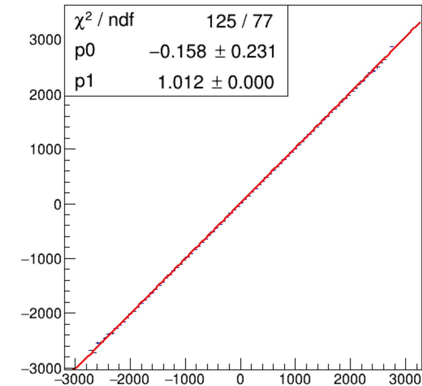
run6388_000_asym_bcm_dg_ds_vs_asym_bcm_an_us_pr.png
