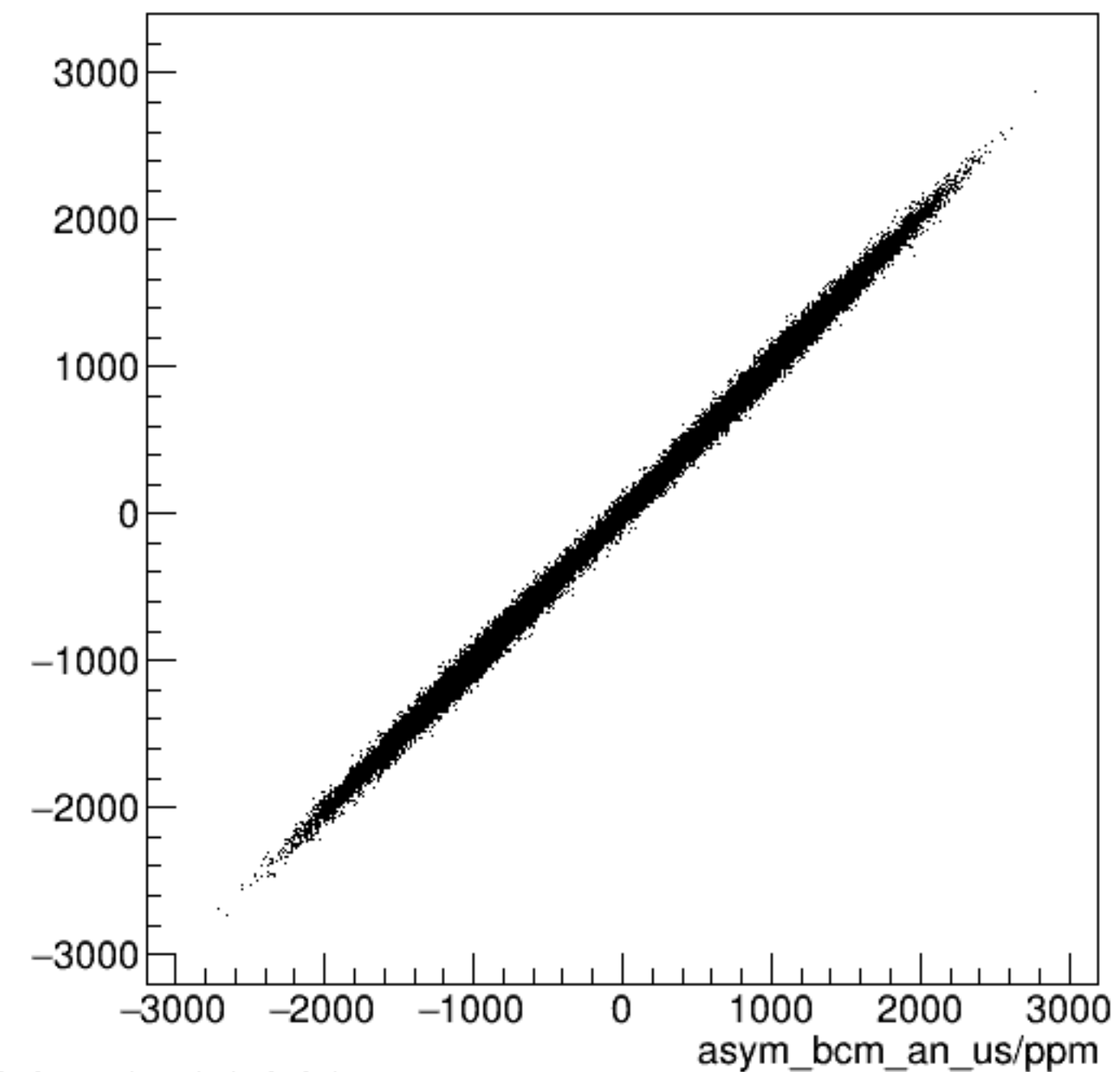
run6388_000_asym_bcm_dg_ds_vs_asym_bcm_an_us_pr.png
