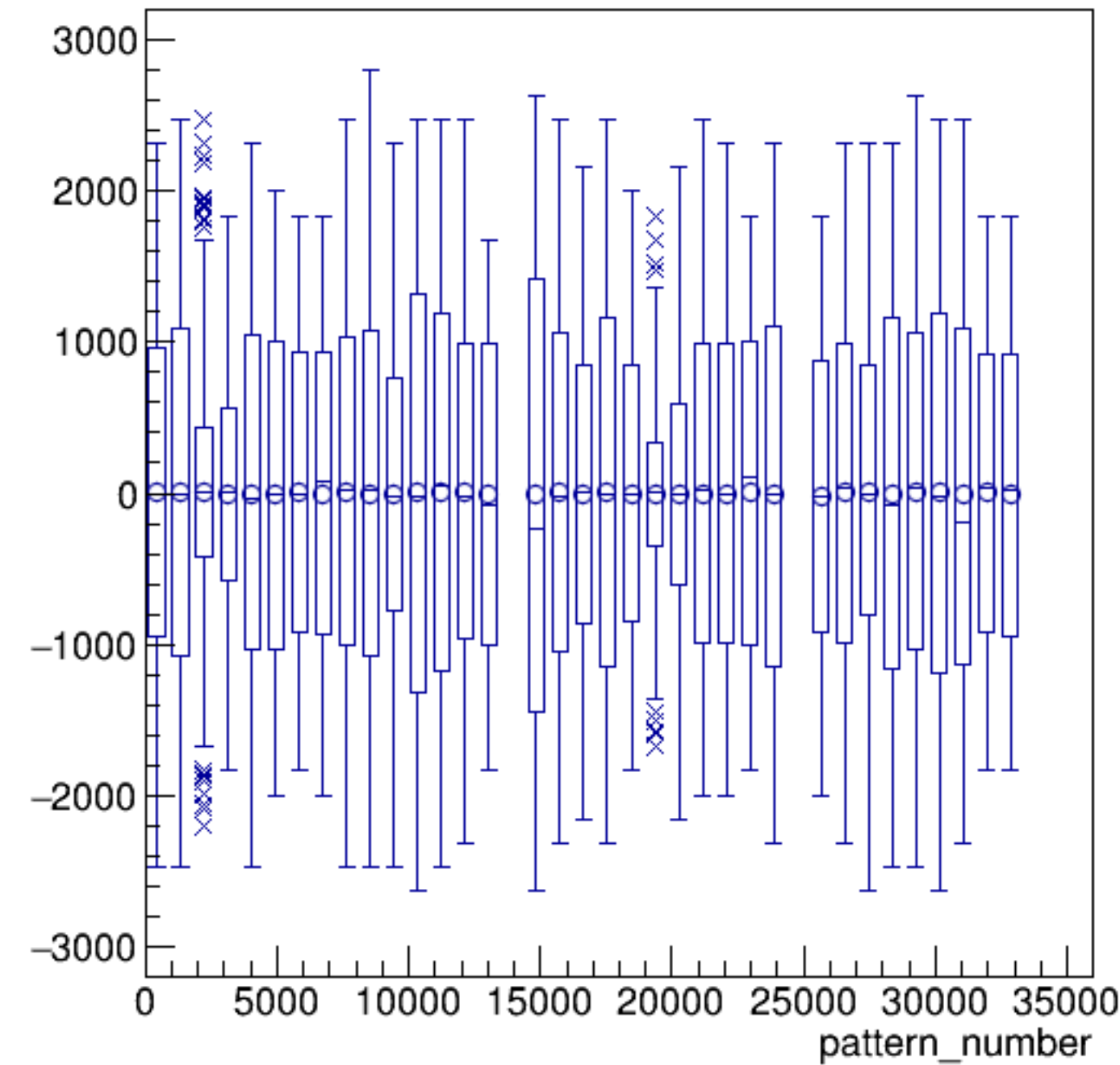
asym_bcm_dg_us/ppm:pattern_number {ErrorFlag==0}
