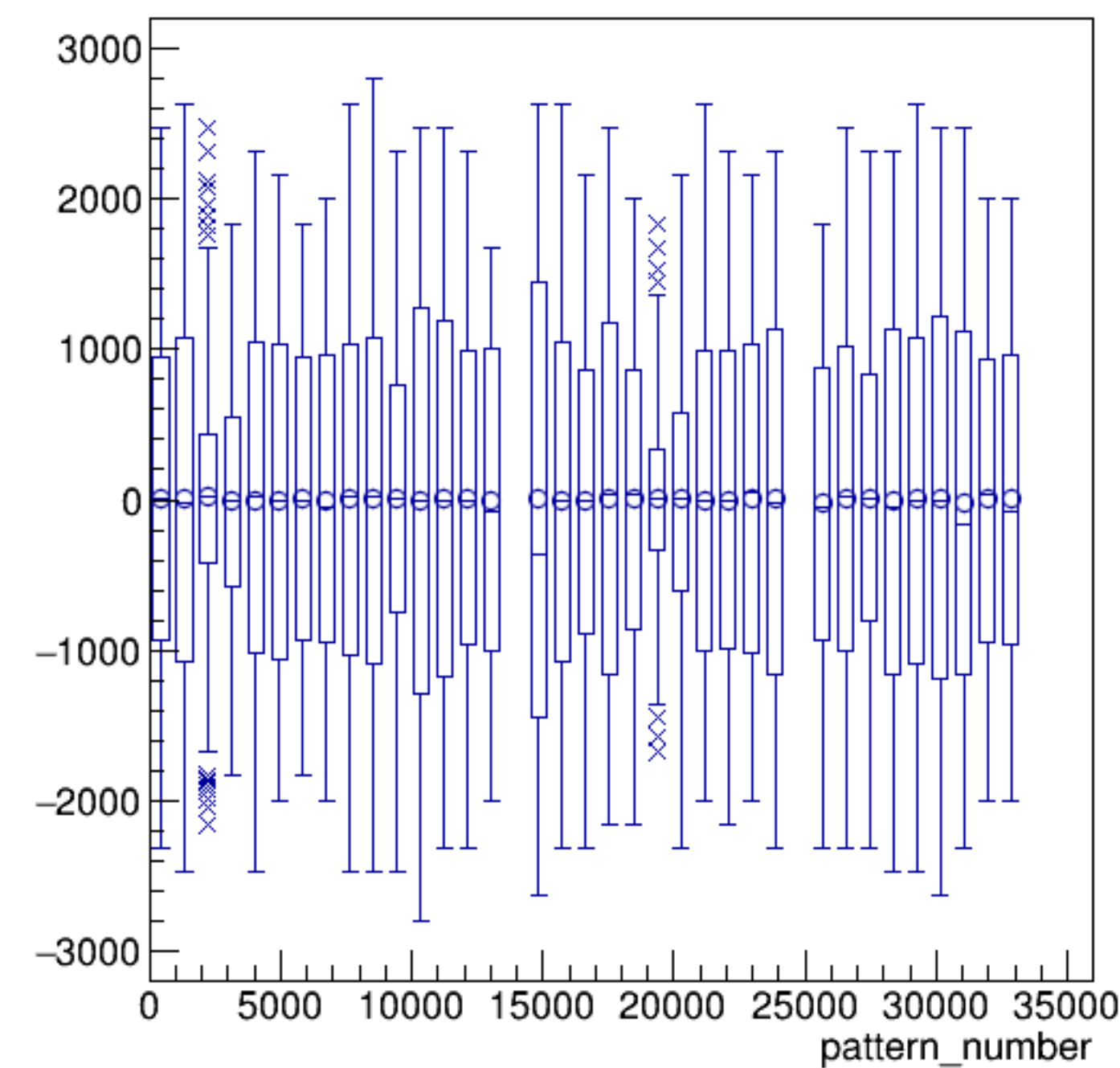
asym_bcm0l02/ppm:pattern_number {ErrorFlag==0}
