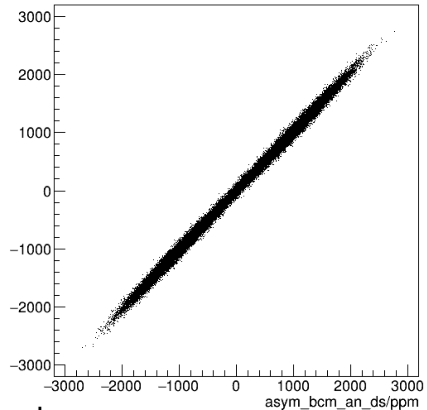
run6388_000_asym_bcm_dg_us_vs_asym_bcm_an_ds_pr.png
