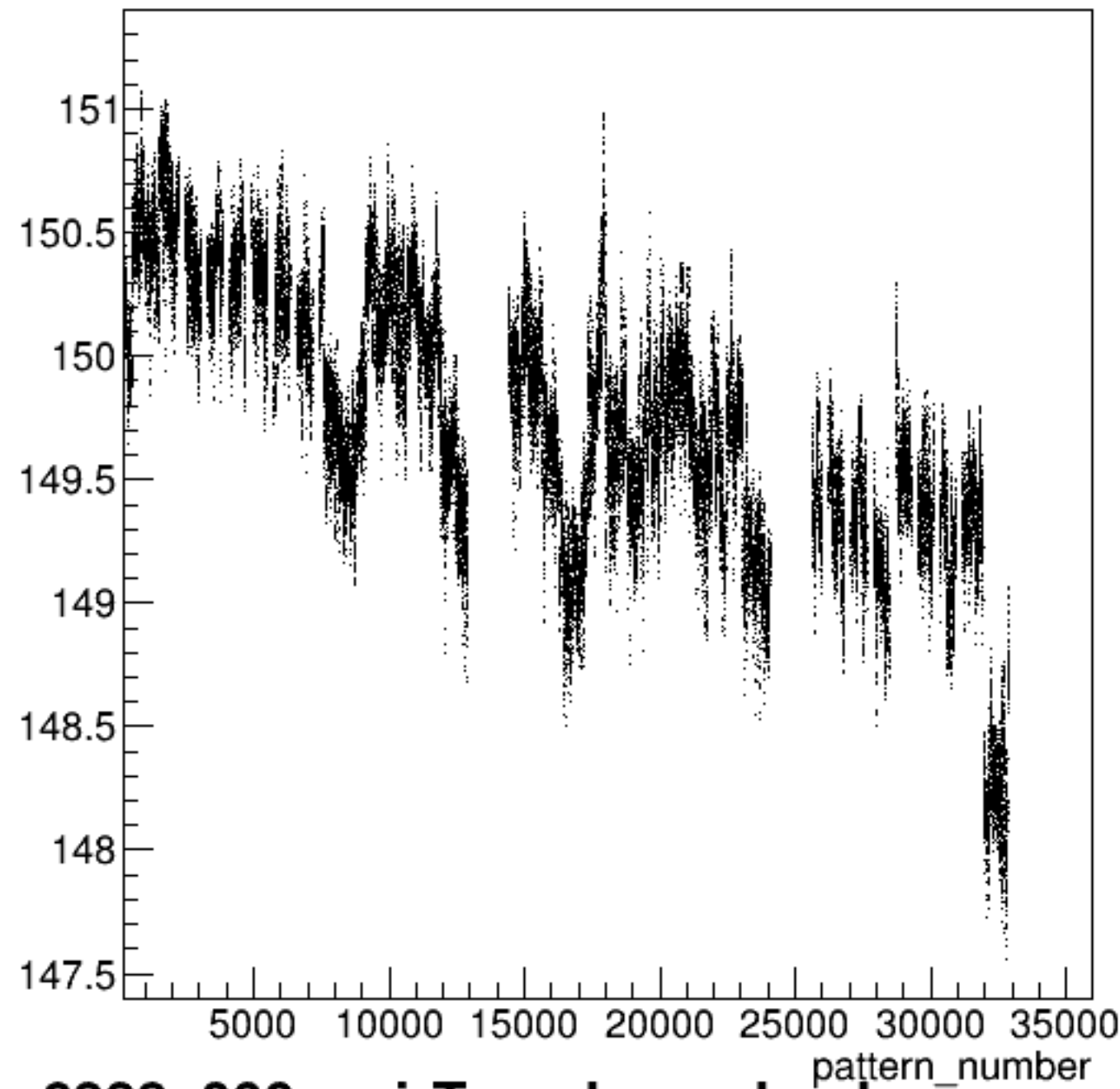
yield_bcm_dg_ds:pattern_number {ErrorFlag==0}
