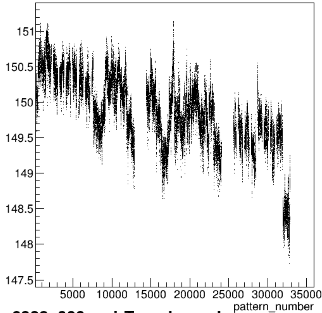
yield_bcm_dg_us:pattern_number {ErrorFlag==0}
