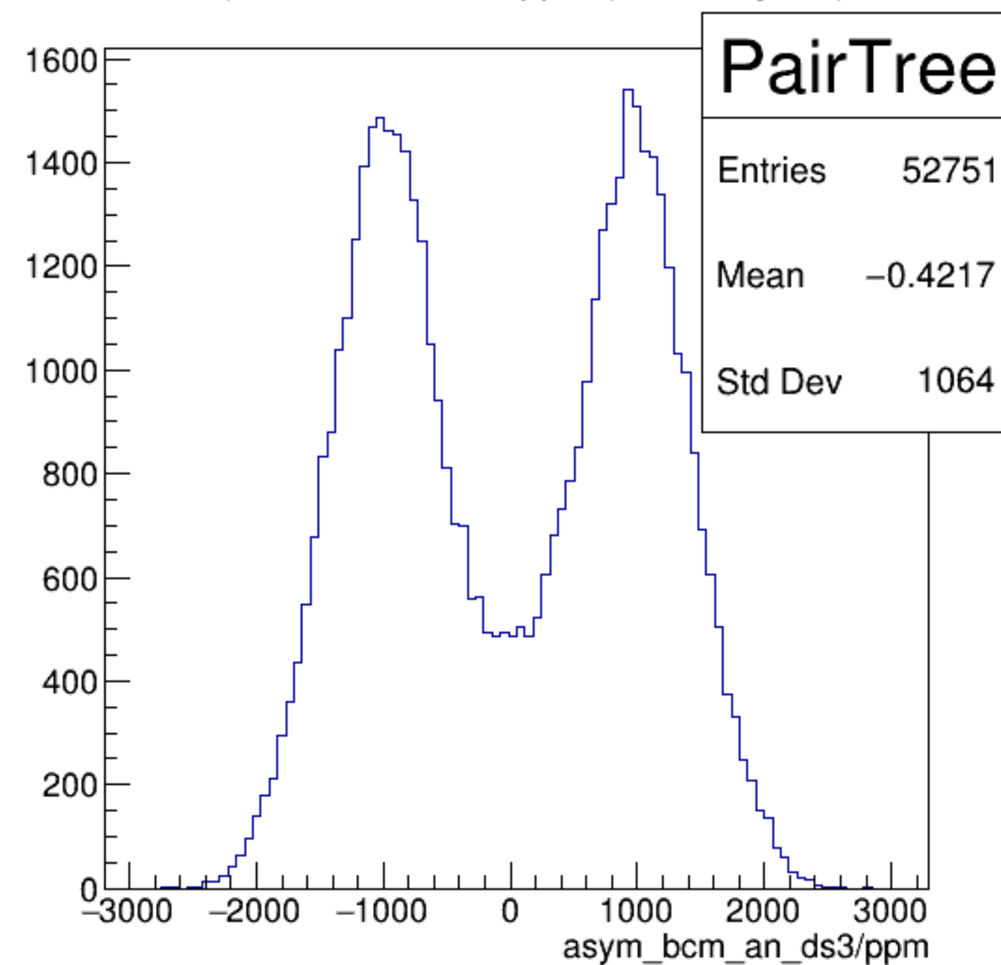
asym_bcm_an_ds3/ppm {ErrorFlag==0}
