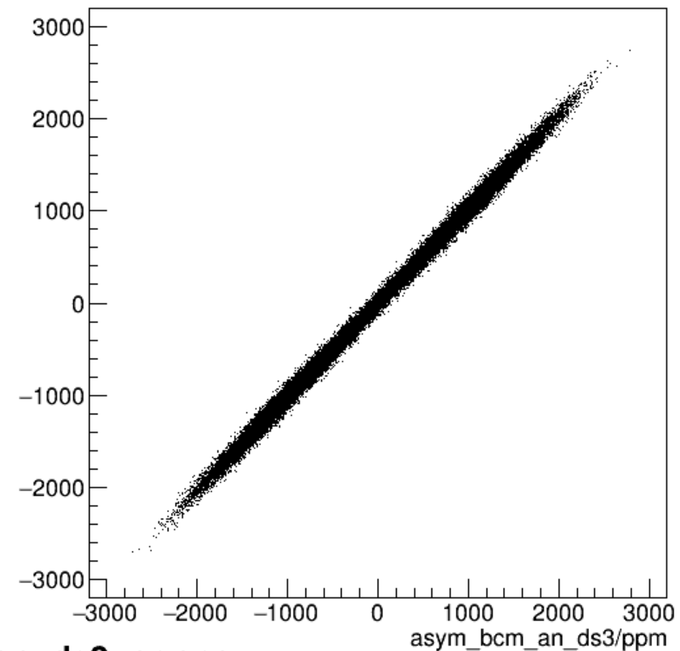
run6388_000_asym_bcm_dg_us_vs_asym_bcm_an_ds3_pr.png
