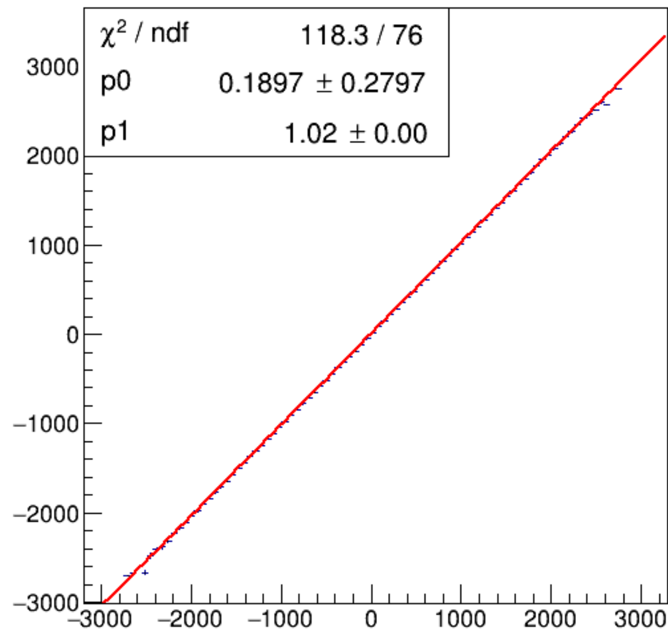
run6388_000_asym_bcm_dg_us_vs_asym_bcm_an_ds_pr.png
