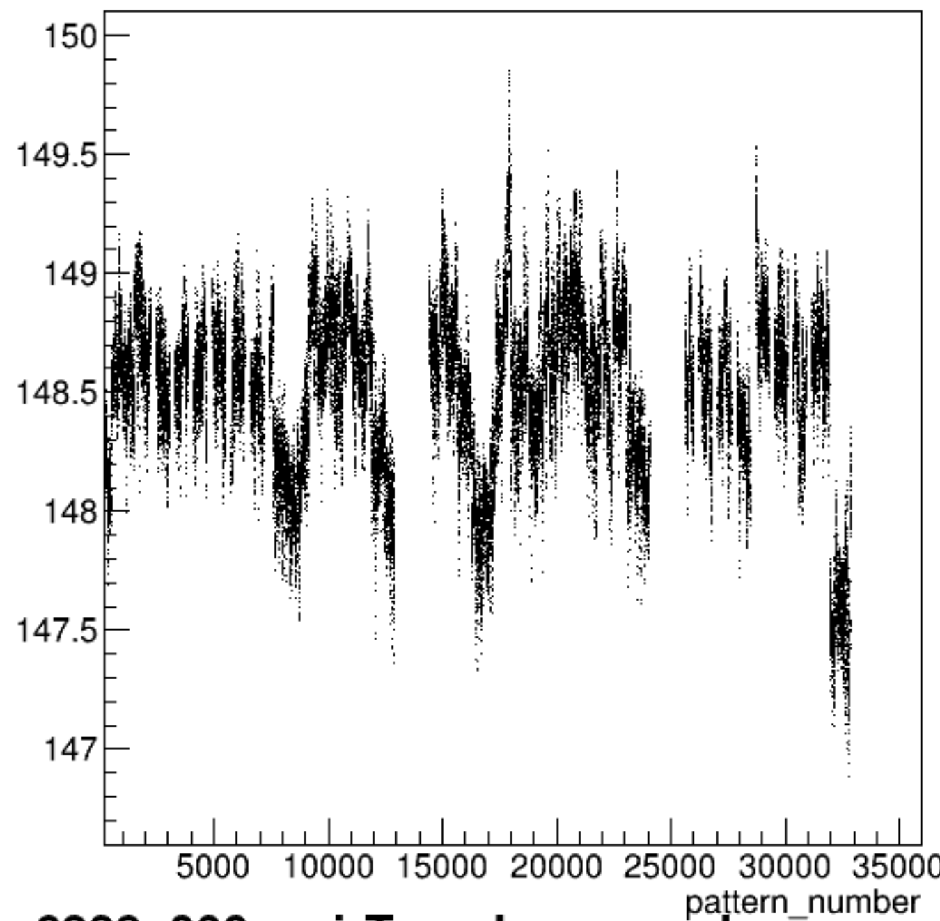
yield_bcm_an_ds:pattern_number {ErrorFlag==0}
