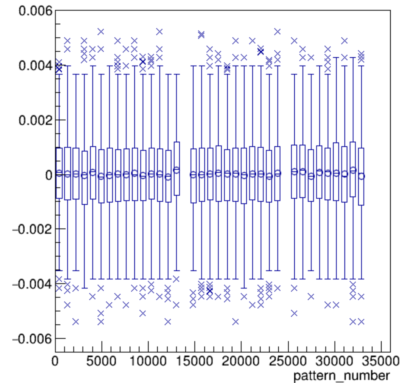
asym_bcm_an_diff*yield_bcm_an_diff:pattern_number {ErrorFlag==0}
