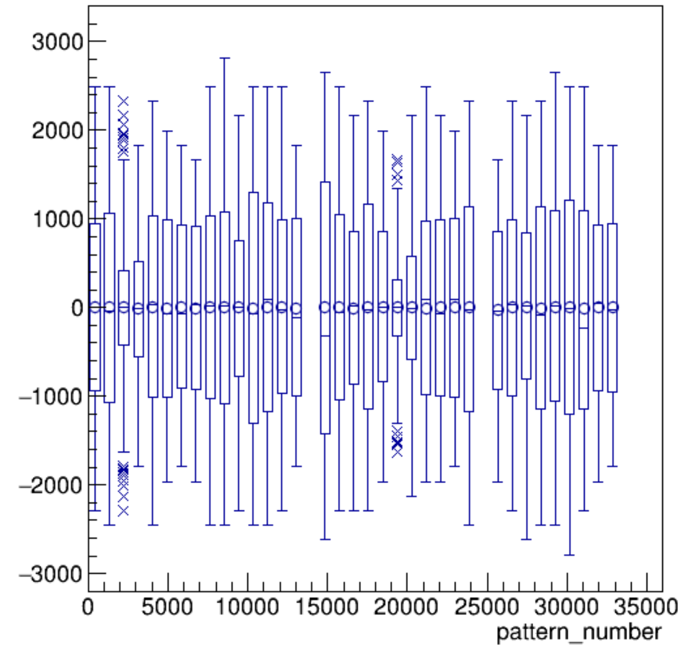
asym_bcm_dg_ds/ppm:pattern_number {ErrorFlag==0}
