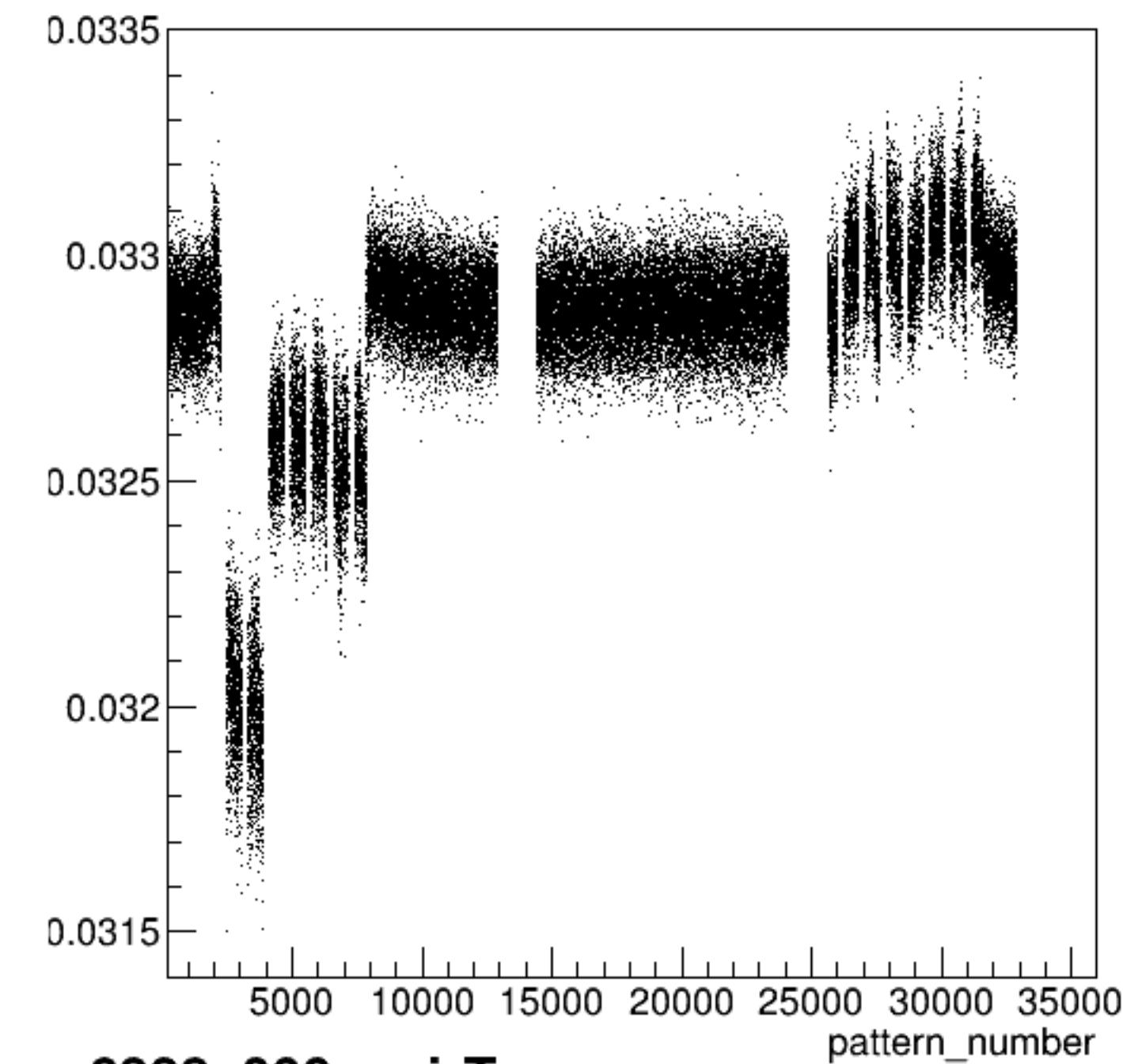
yield_usr:pattern_number {ErrorFlag==0}
