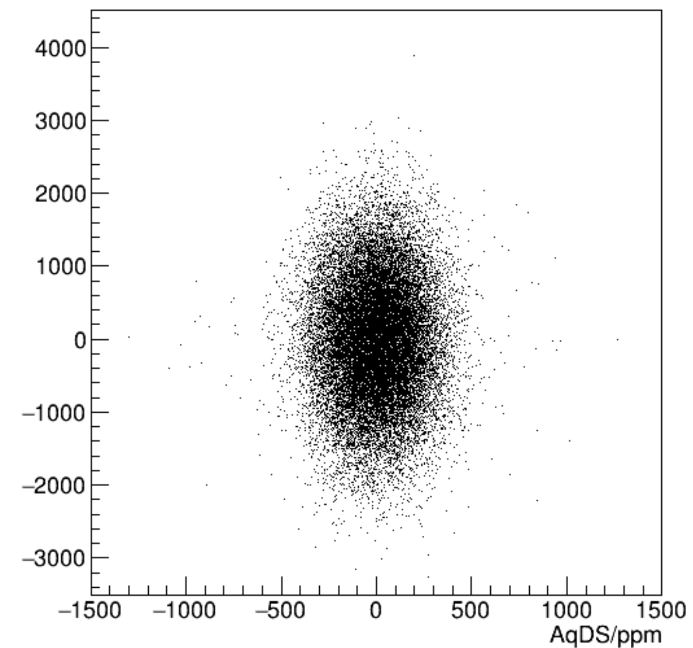
reg_asym_usr/ppm:AqDS/ppm {ok_cut}
