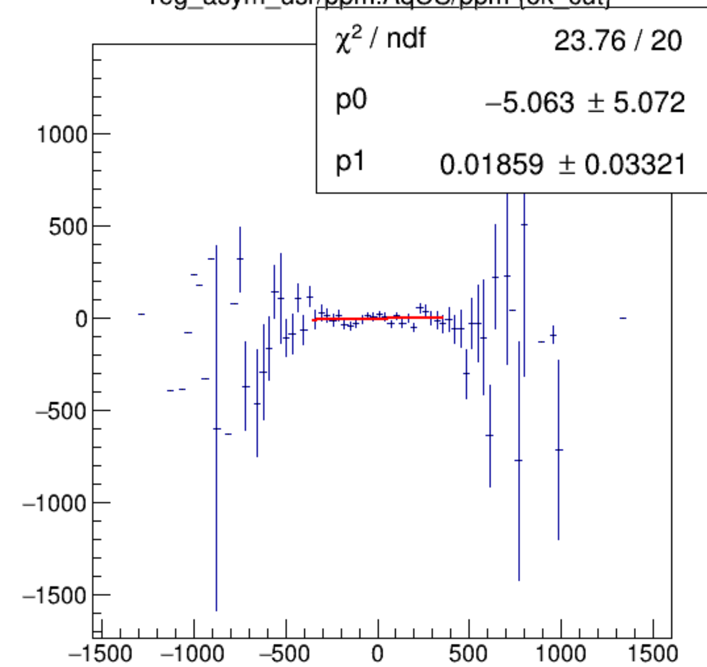
reg_asym_usr/ppm:AqUS/ppm {ok_cut}
