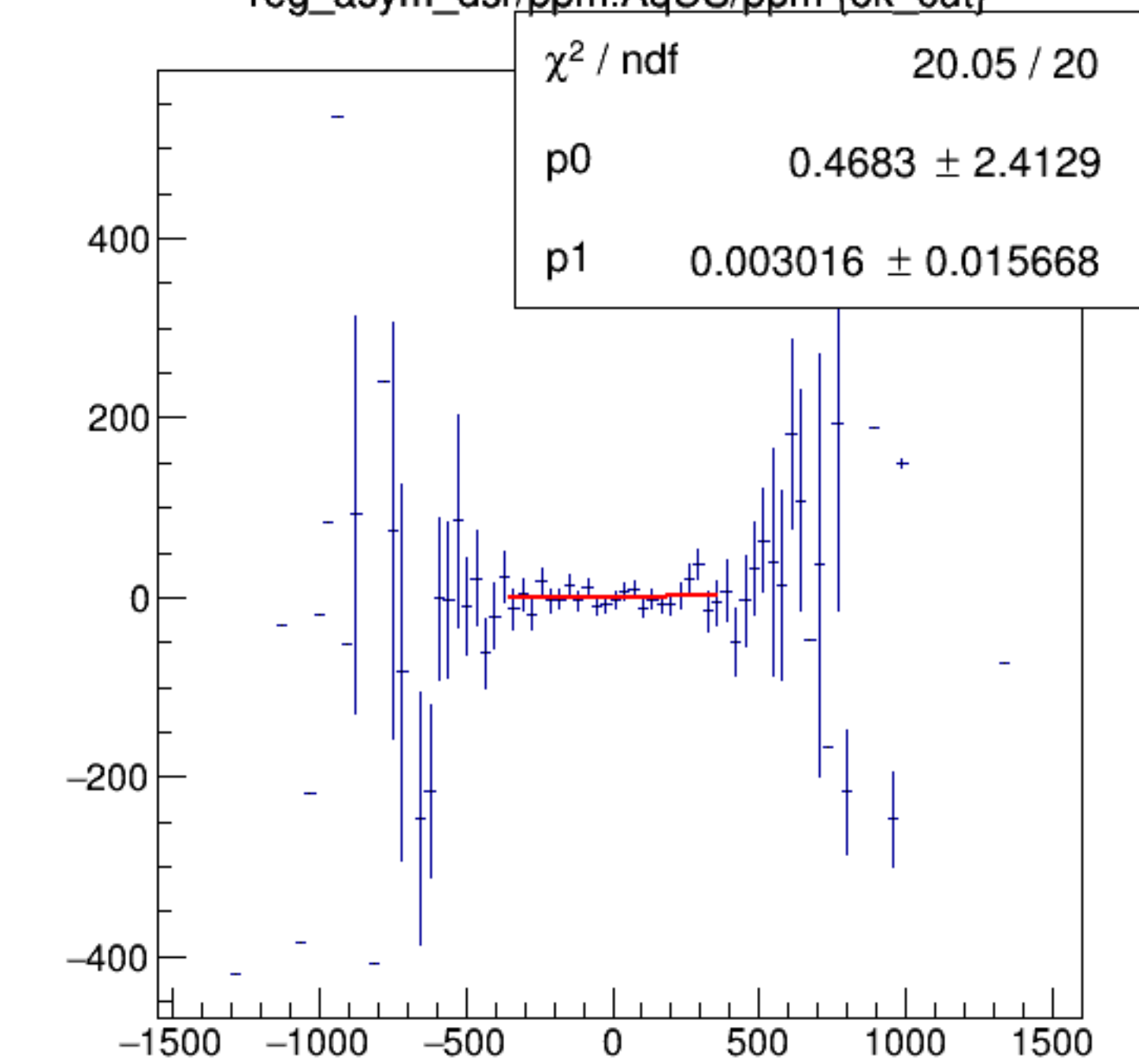
reg_asym_dsr/ppm:AqUS/ppm {ok_cut}
