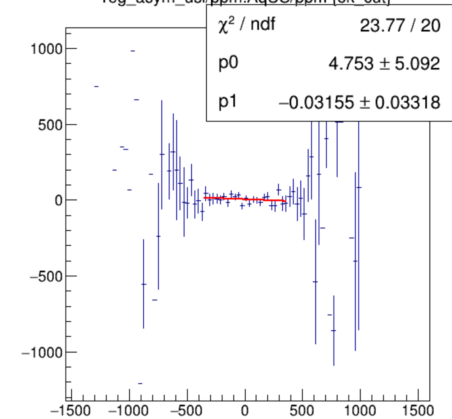
reg_asym_usl/ppm:AqUS/ppm {ok_cut}
