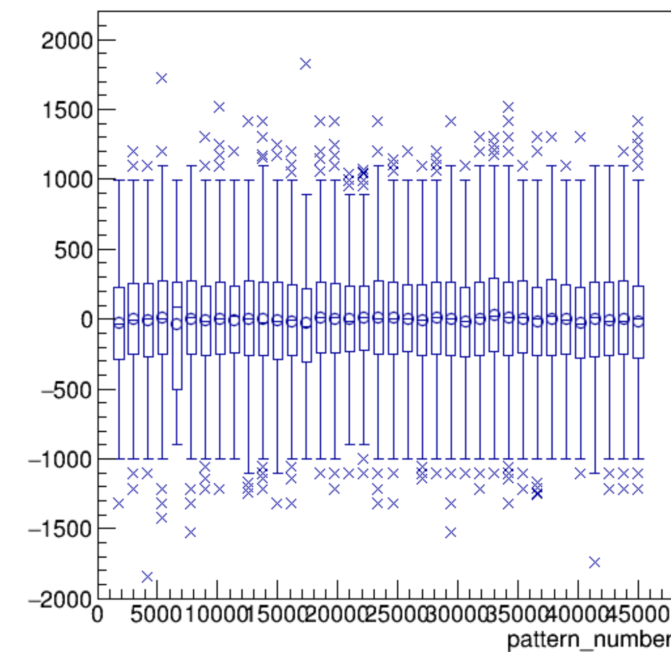
asym_dsr/ppm:pattern_number {ErrorFlag==0}
