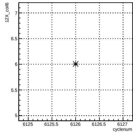
12X_coil6:cyclenum {run == 6390}
