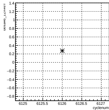
delta46_12X4eY:cyclenum {run == 6390}
