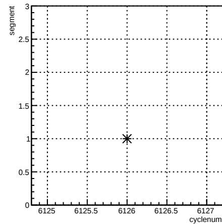
segment:cyclenum {run == 6390}
