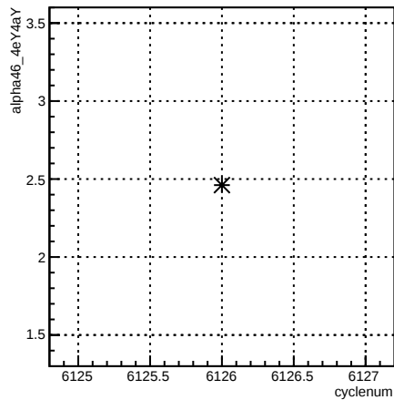
run:cyclenum {run == 6390}
