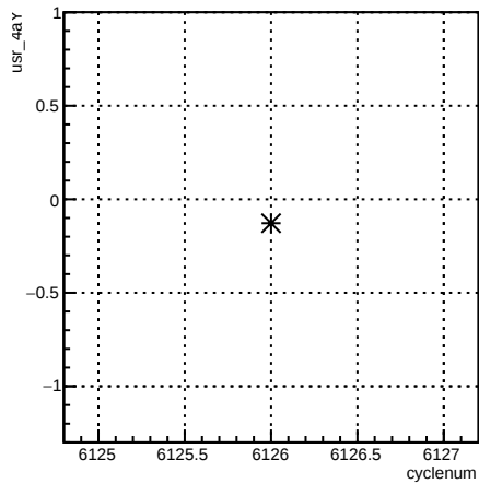
usr_4aY:cyclenum {run == 6390}
