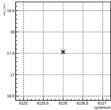
usl_4eY:cyclenum {run == 6390}
