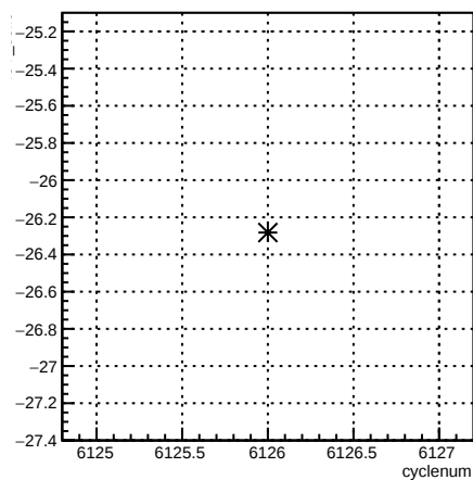
4eY_coil6:cyclenum {run == 6390}
