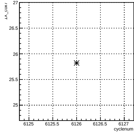
4eX_coil7:cyclenum {run == 6390}
