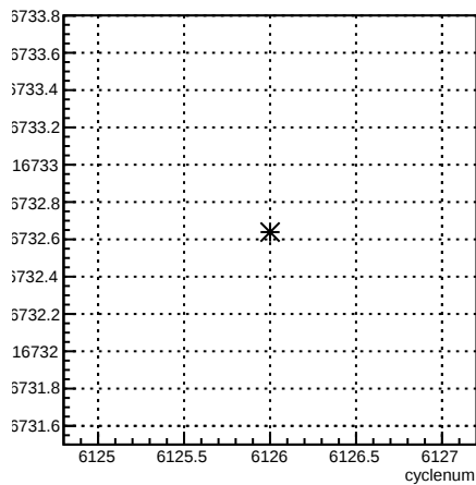
usl_coil1:cyclenum {run == 6390}
