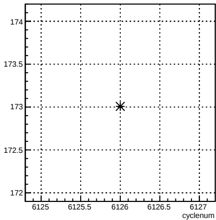
4eY_coil4:cyclenum {run == 6390}
