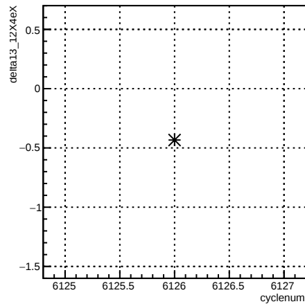
segment:cyclenum {run == 6390}
