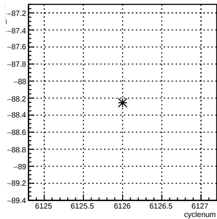
4eX_coil3:cyclenum {run == 6390}
