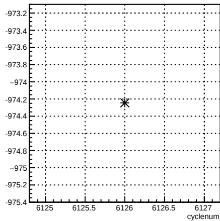
usl_coil6:cyclenum {run == 6390}
