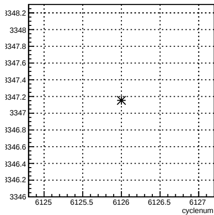
usl_coil7:cyclenum {run == 6390}
