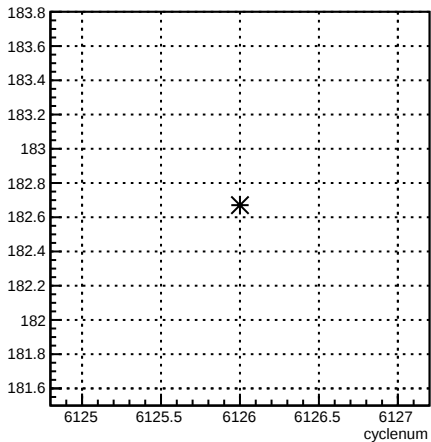
4eY_coil4:cyclenum {run == 6390}
