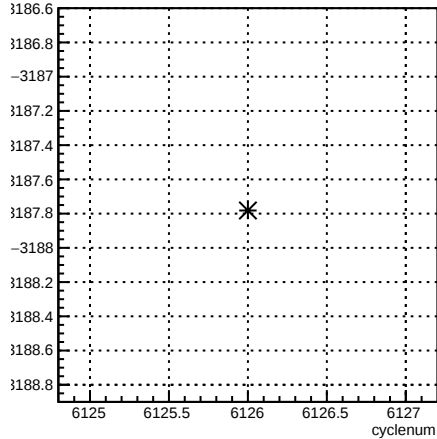
usr_coil7:cyclenum {run == 6390}
