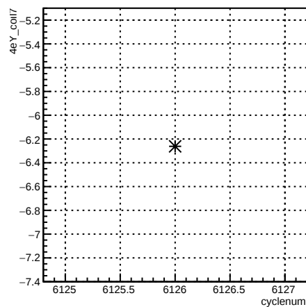
4eY_coil7:cyclenum {run == 6390}
