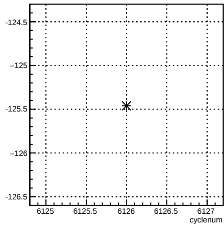
usr_4eY:cyclenum {run == 6390}
