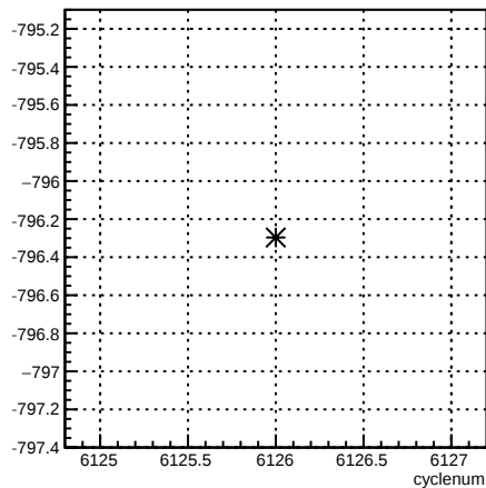
usr_coil6:cyclenum {run == 6390}
