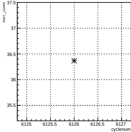
4eY_coil6:cyclenum {run == 6390}
