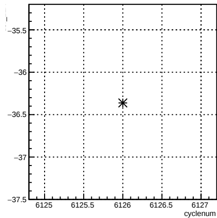
usr_12X:cyclenum {run == 6390}
