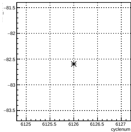
12X_coil7:cyclenum {run == 6390}
