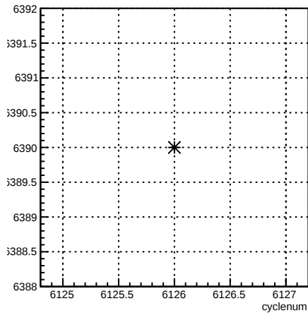
run:cyclenum {run == 6390}
