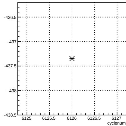
4eX_coil1:cyclenum {run == 6390}
