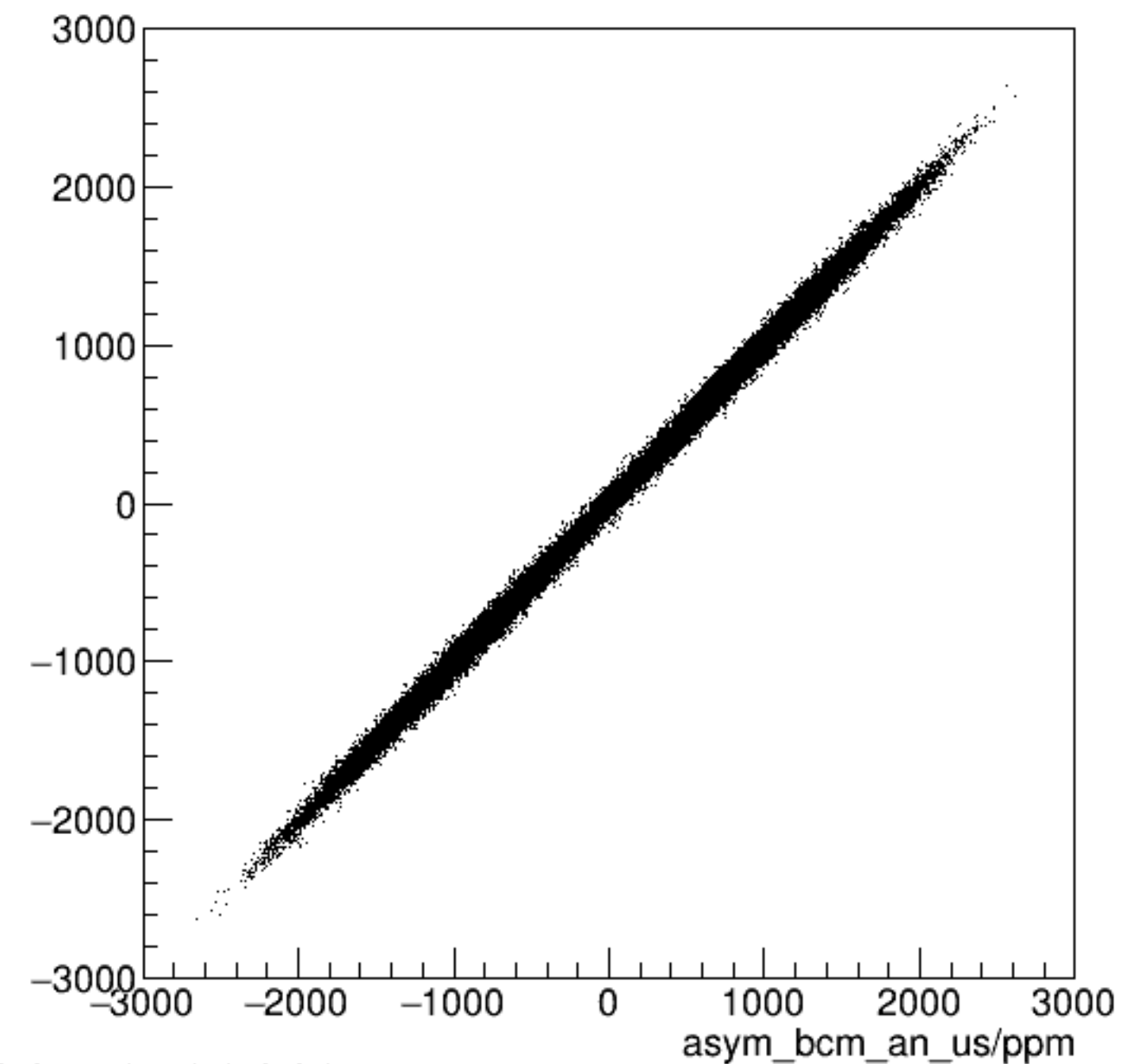
run6391_000_asym_bcm_dg_ds_vs_asym_bcm_an_us_pr.png
