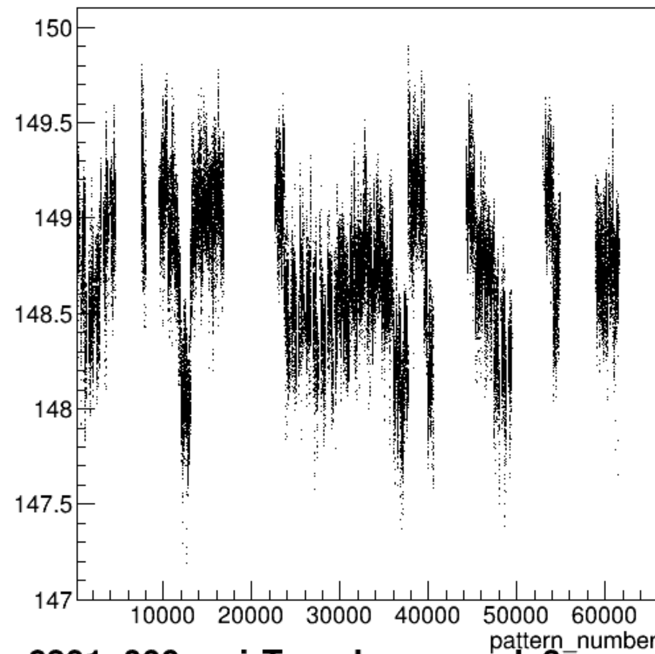
yield_bcm_an_ds3:pattern_number {ErrorFlag==0}
