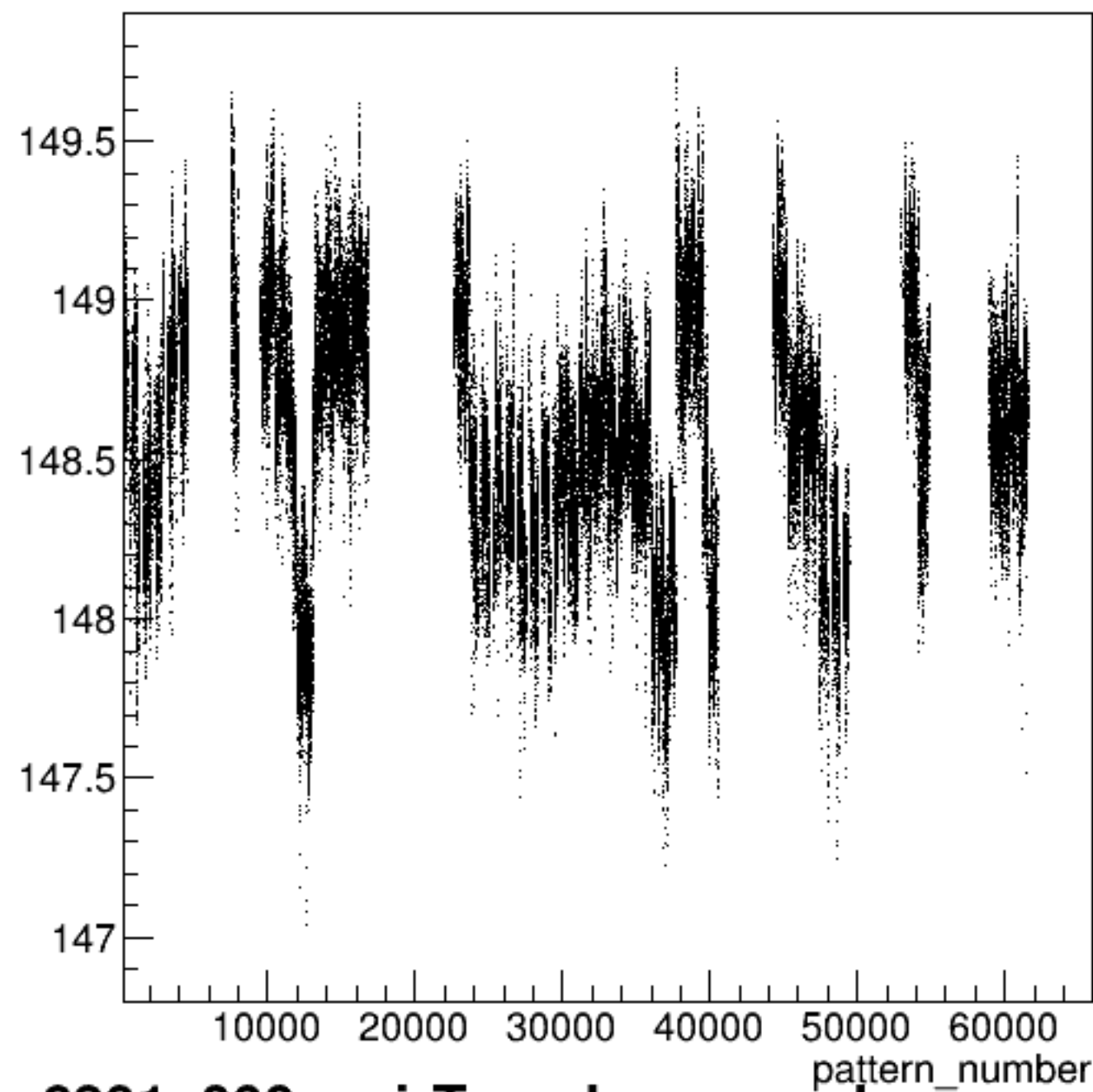
yield_bcm_an_ds:pattern_number {ErrorFlag==0}
