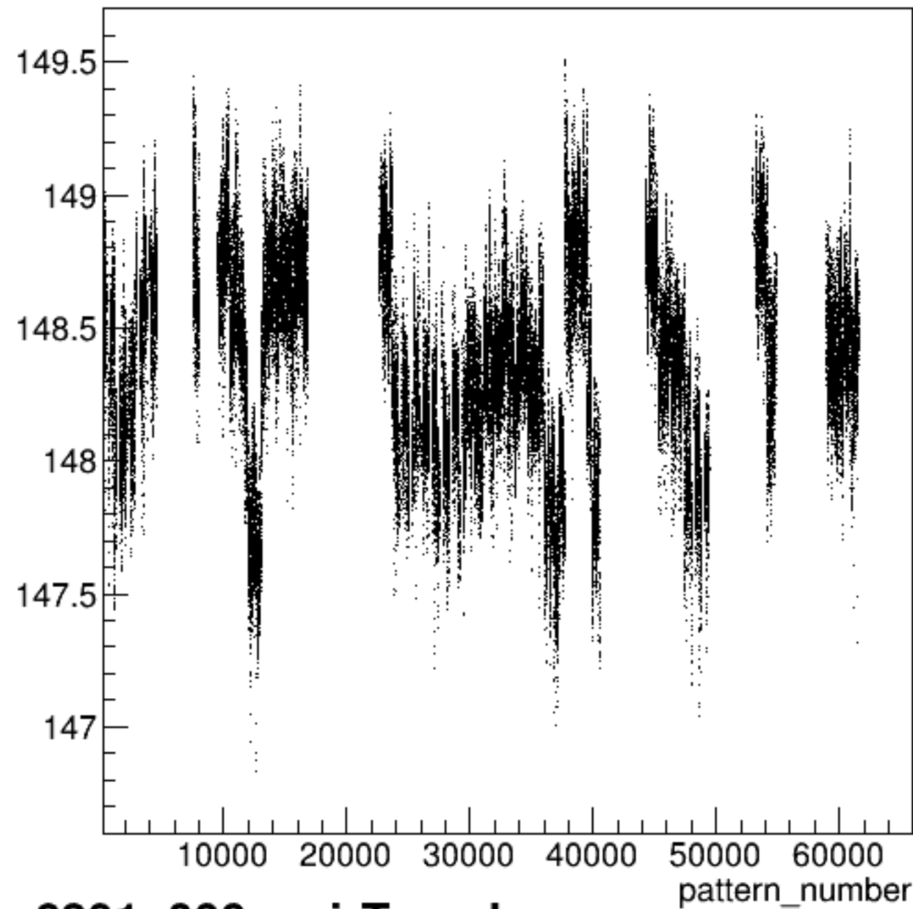
yield_bcm_an_us:pattern_number {ErrorFlag==0}
