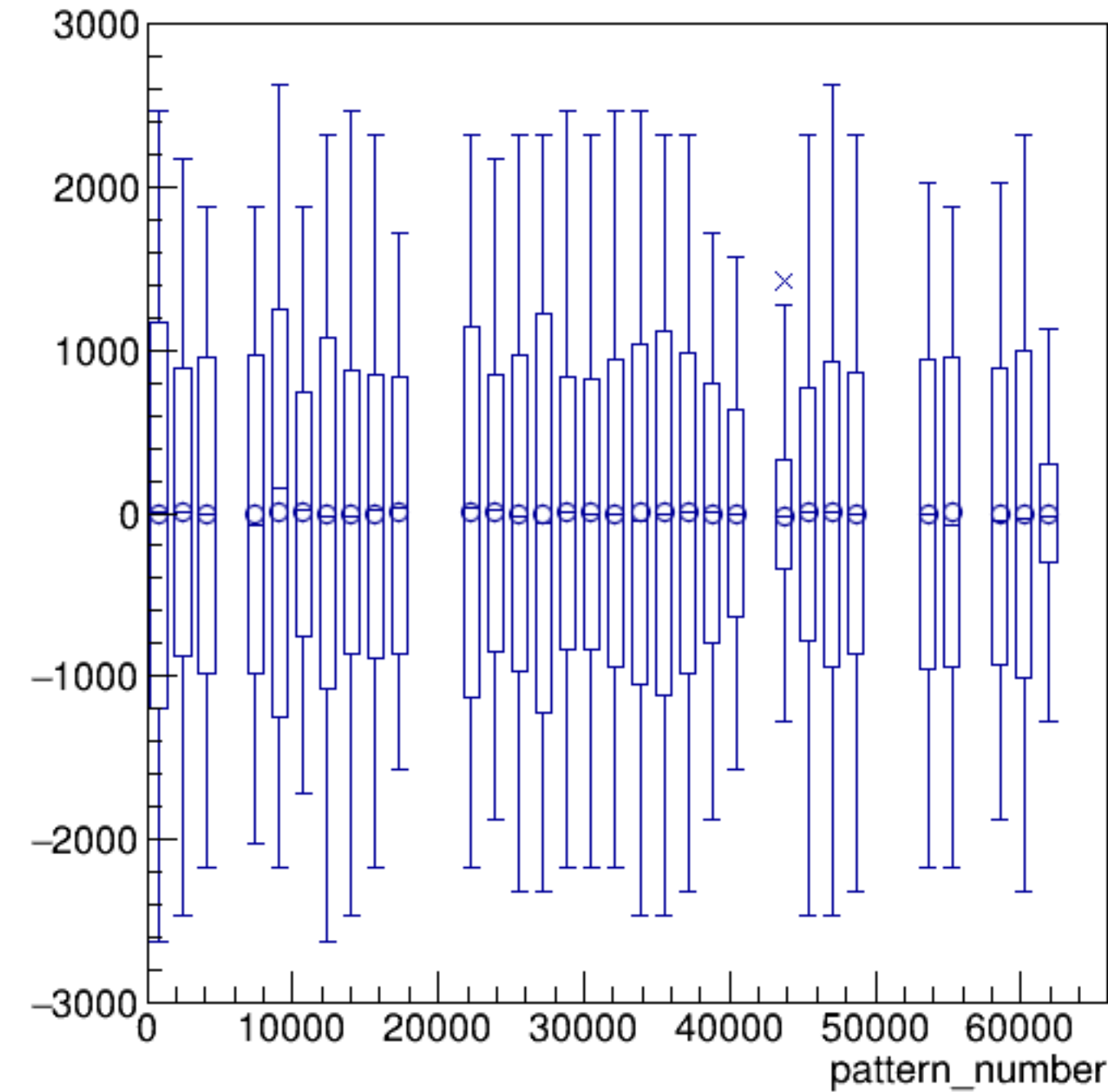
asym_bcm_an_us/ppm:pattern_number {ErrorFlag==0}
