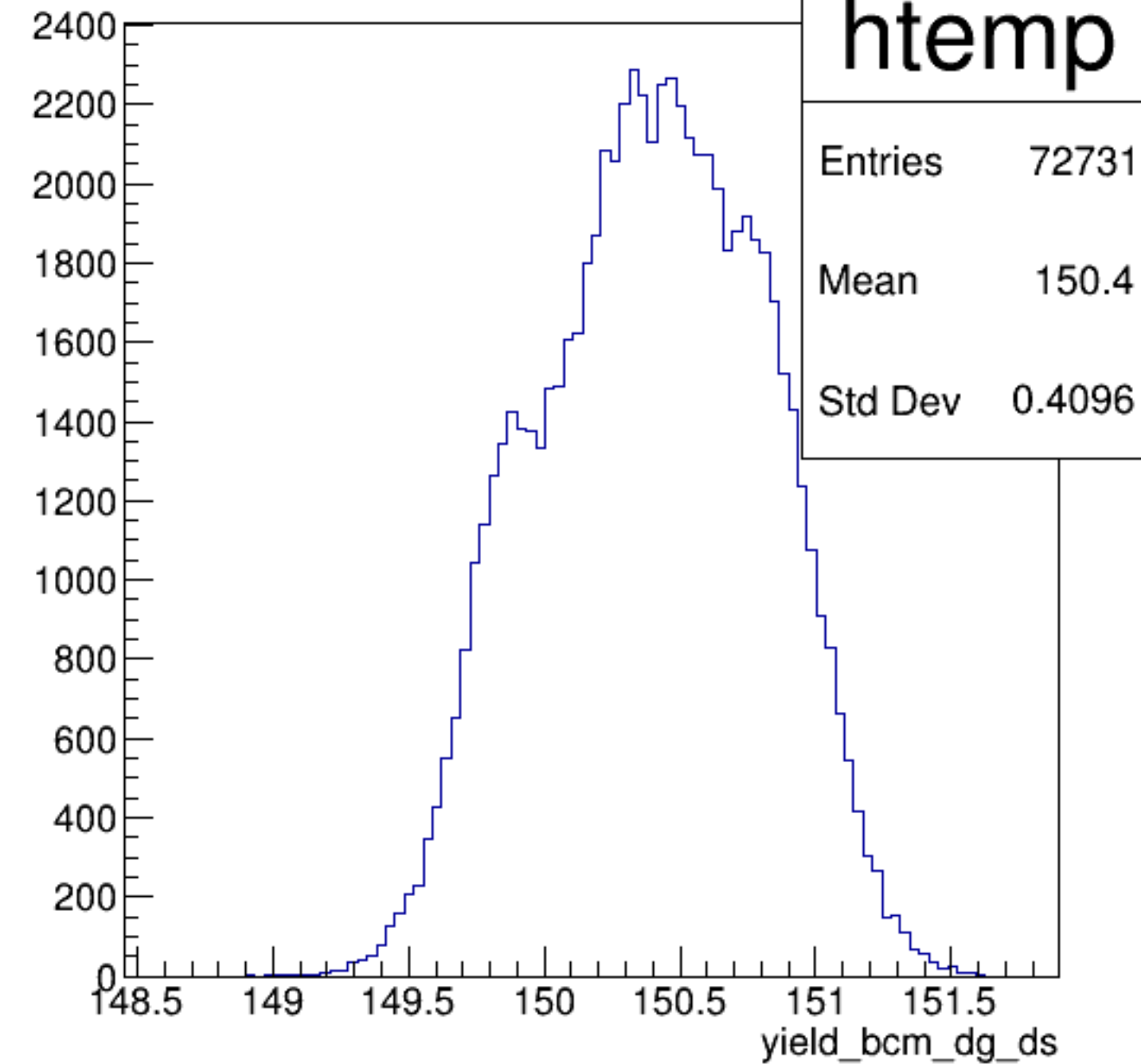
yield_bcm_dg_ds {ErrorFlag==0}
