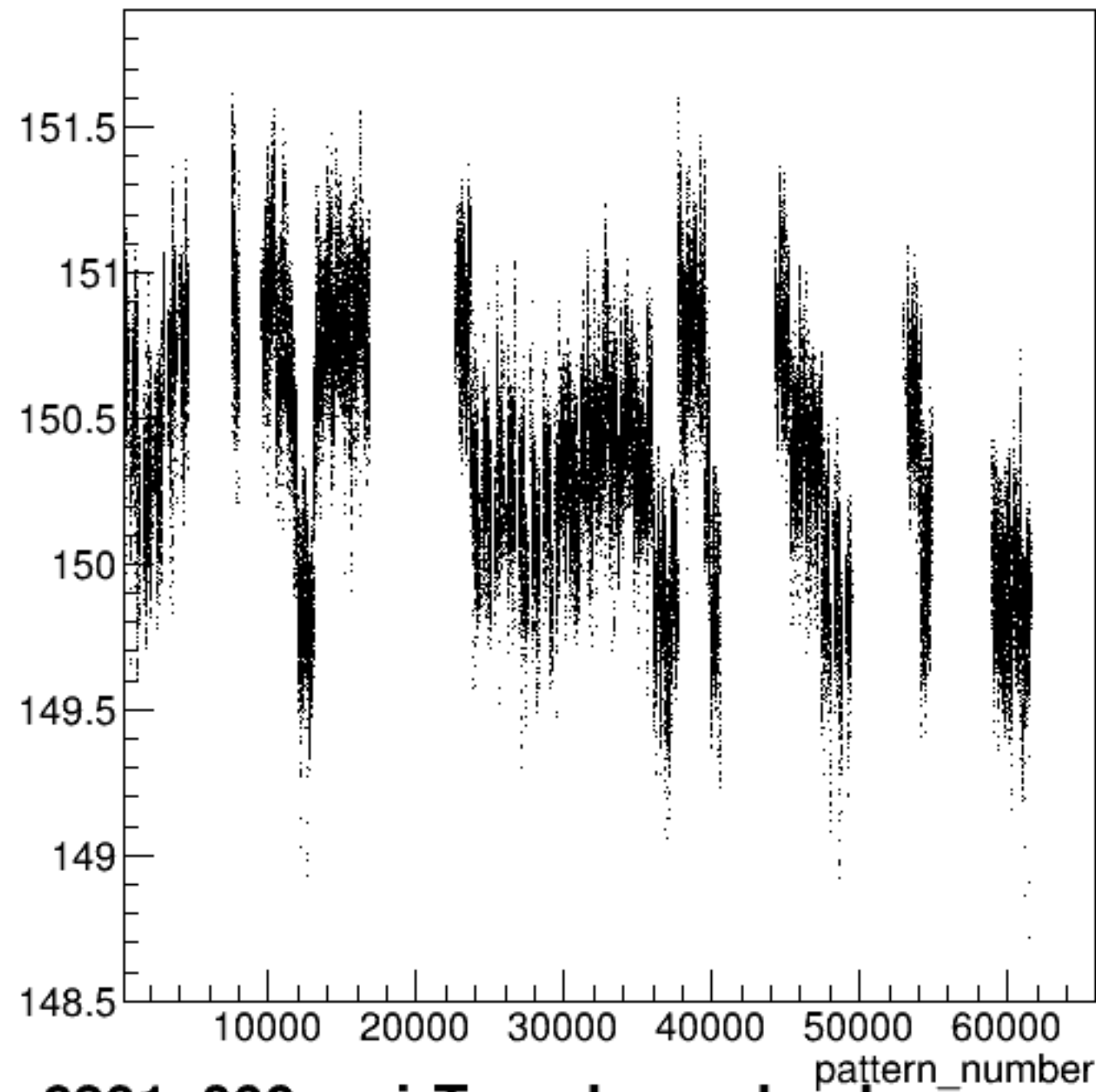
yield_bcm_dg_ds:pattern_number {ErrorFlag==0}
