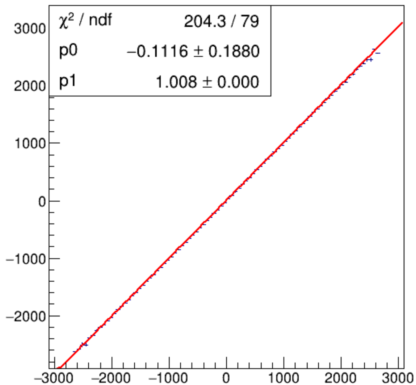
run6391_000_asym_bcm_dg_ds_vs_asym_bcm_an_us_pr.png
