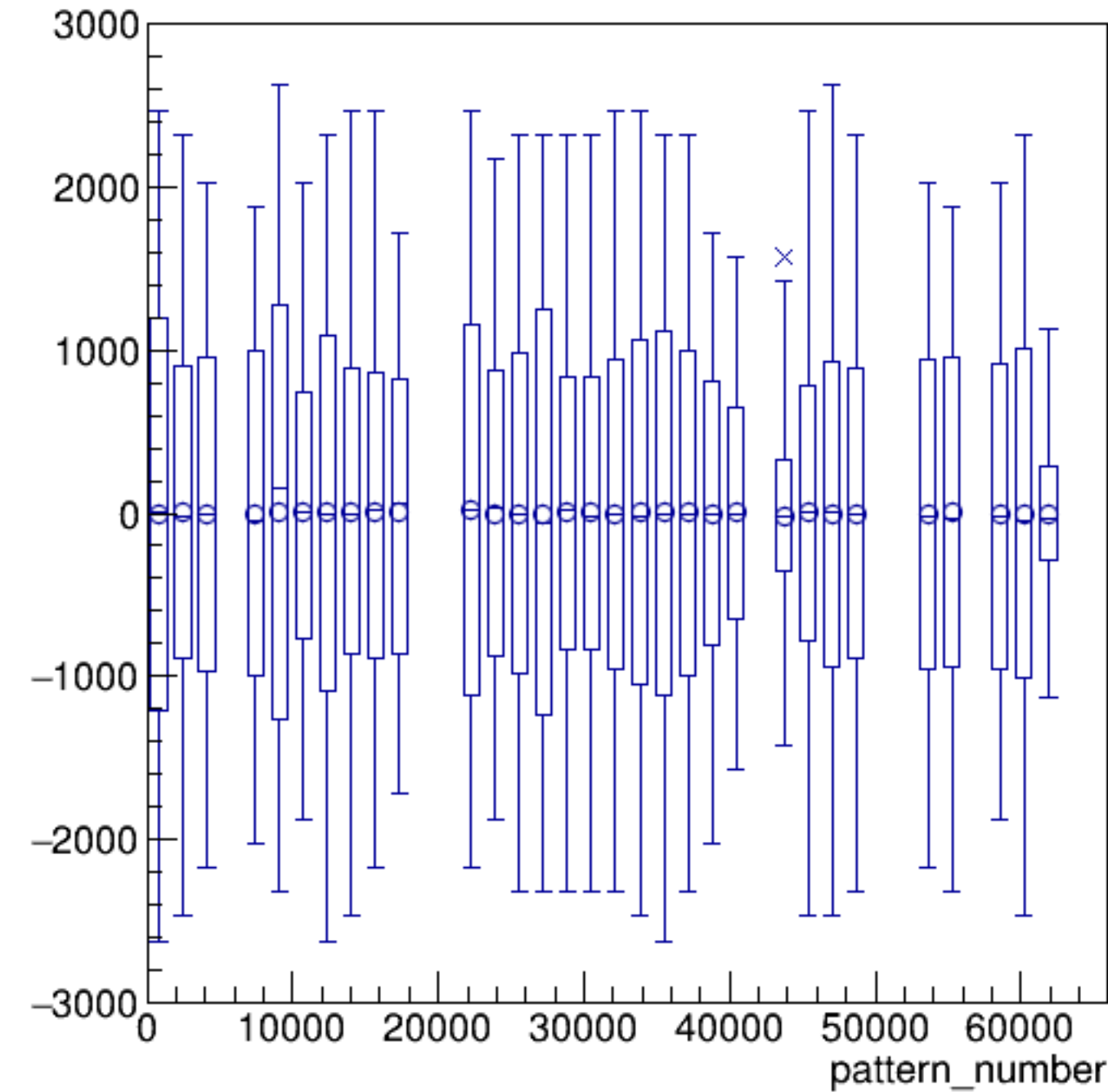
asym_bcm_dg_ds/ppm:pattern_number {ErrorFlag==0}
