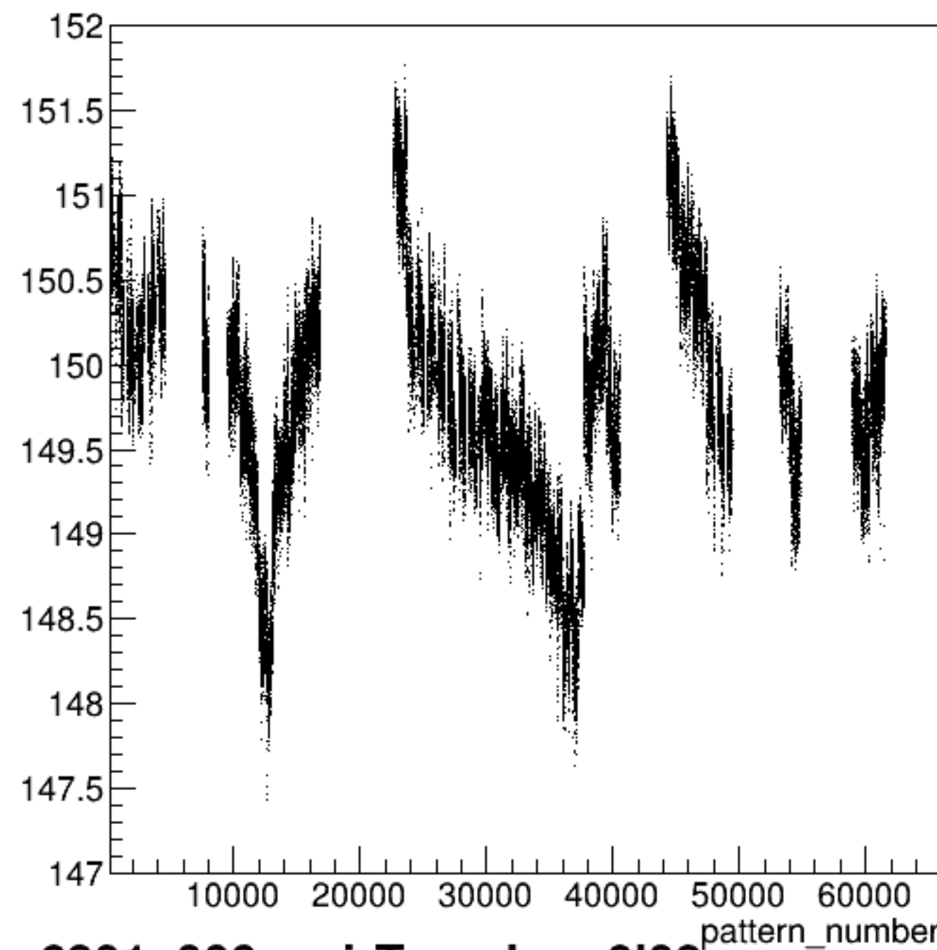
yield_bcm0l02:pattern_number {ErrorFlag==0}
