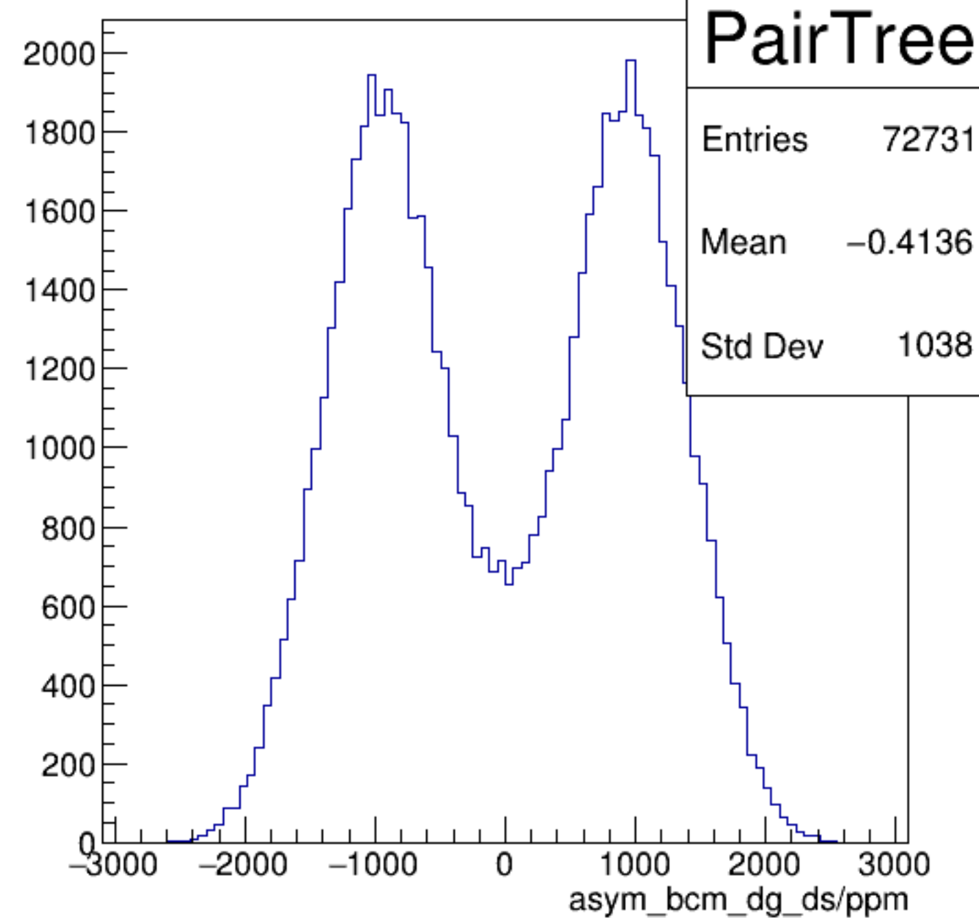
asym_bcm_dg_ds/ppm {ErrorFlag==0}
