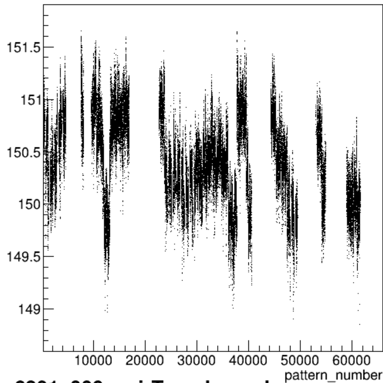
yield_bcm_dg_us:pattern_number {ErrorFlag==0}
