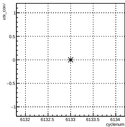
usl_coil7:cyclenum {run == 6394}
