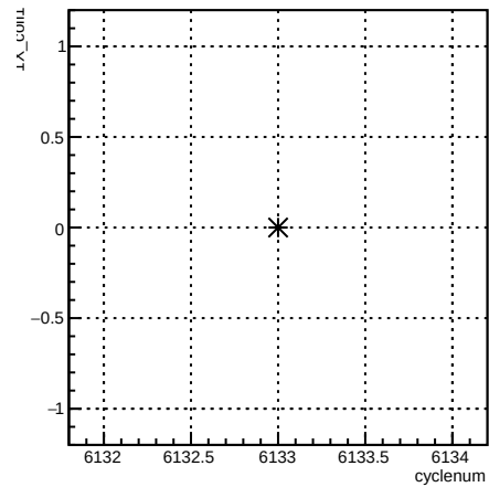
1X_coil1:cyclenum {run == 6394}
