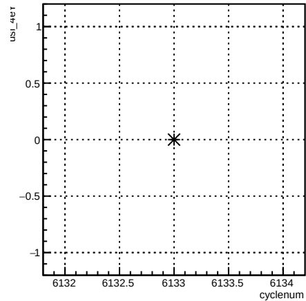
usl_4eY:cyclenum {run == 6394}
