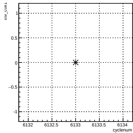
usl_coil1:cyclenum {run == 6394}
