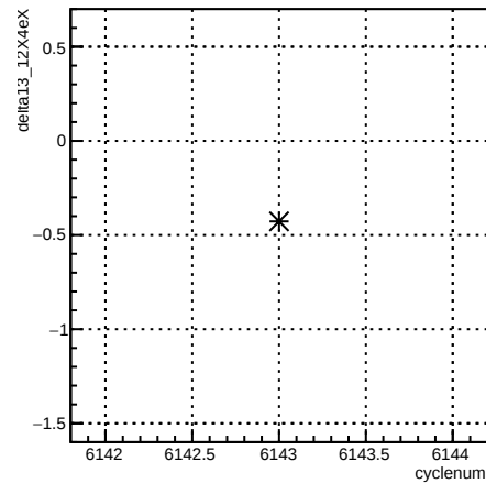
delta13_12X4eX:cyclenum {run == 6398}
