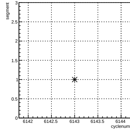
segment:cyclenum {run == 6398}
