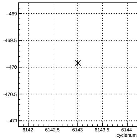
4eX_coil1:cyclenum {run == 6398}
