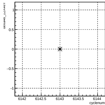
delta46_12X4eY:cyclenum {run == 6398}
