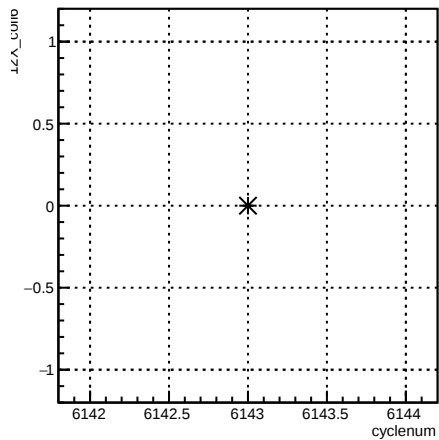
12X_coil6:cyclenum {run == 6398}
