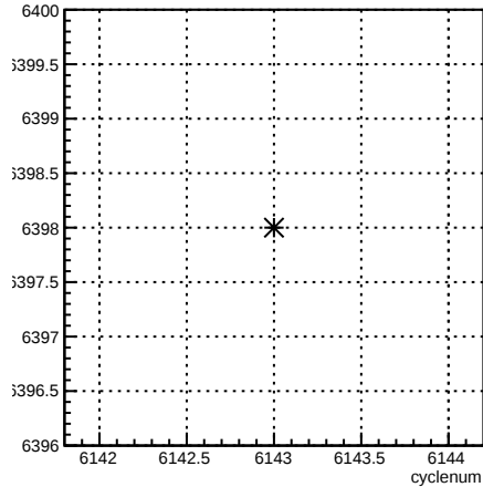
run:cyclenum {run == 6398}
