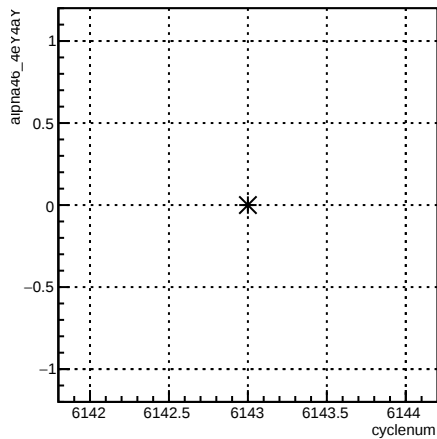
alpha46_4eY4aY:cyclenum {run == 6398}
