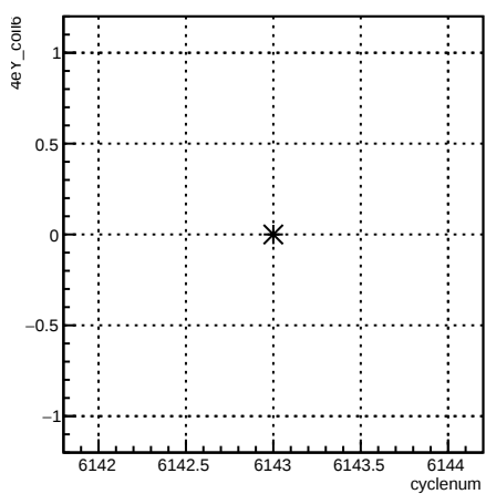
4eY_coil6:cyclenum {run == 6398}
