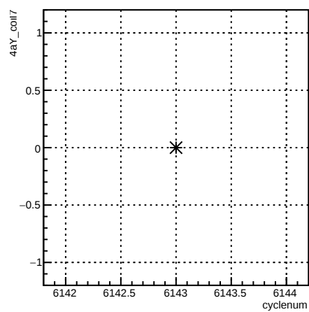
4aY_coil7:cyclenum {run == 6398}
