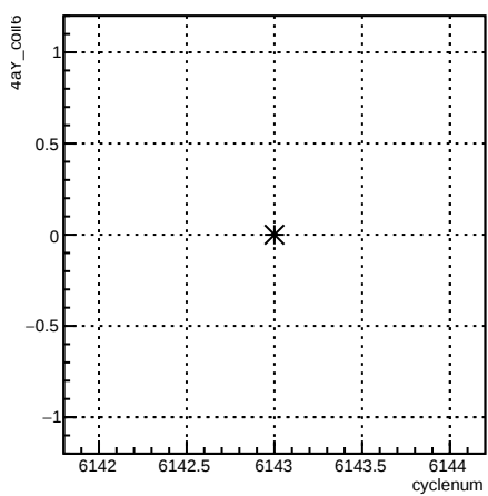
4aY_coil6:cyclenum {run == 6398}
