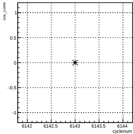
usl_coil6:cyclenum {run == 6398}
