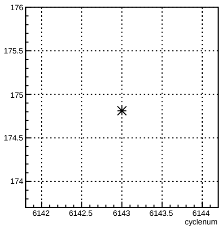
4aY_coil4:cyclenum {run == 6398}
