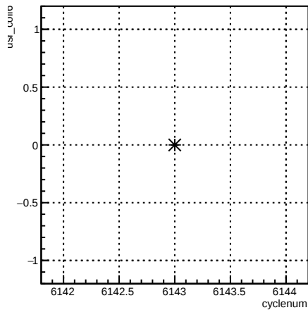
usr_coil6:cyclenum {run == 6398}
