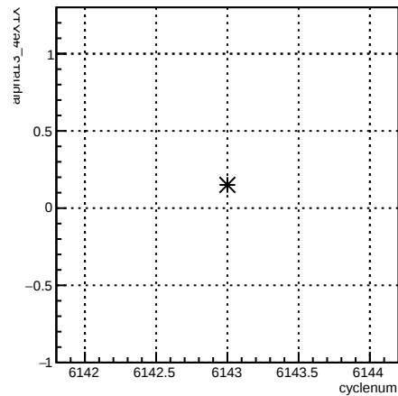
alpha13_4eX1X:cyclenum {run == 6398}
