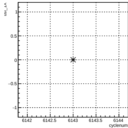
usl_4eY:cyclenum {run == 6398}
