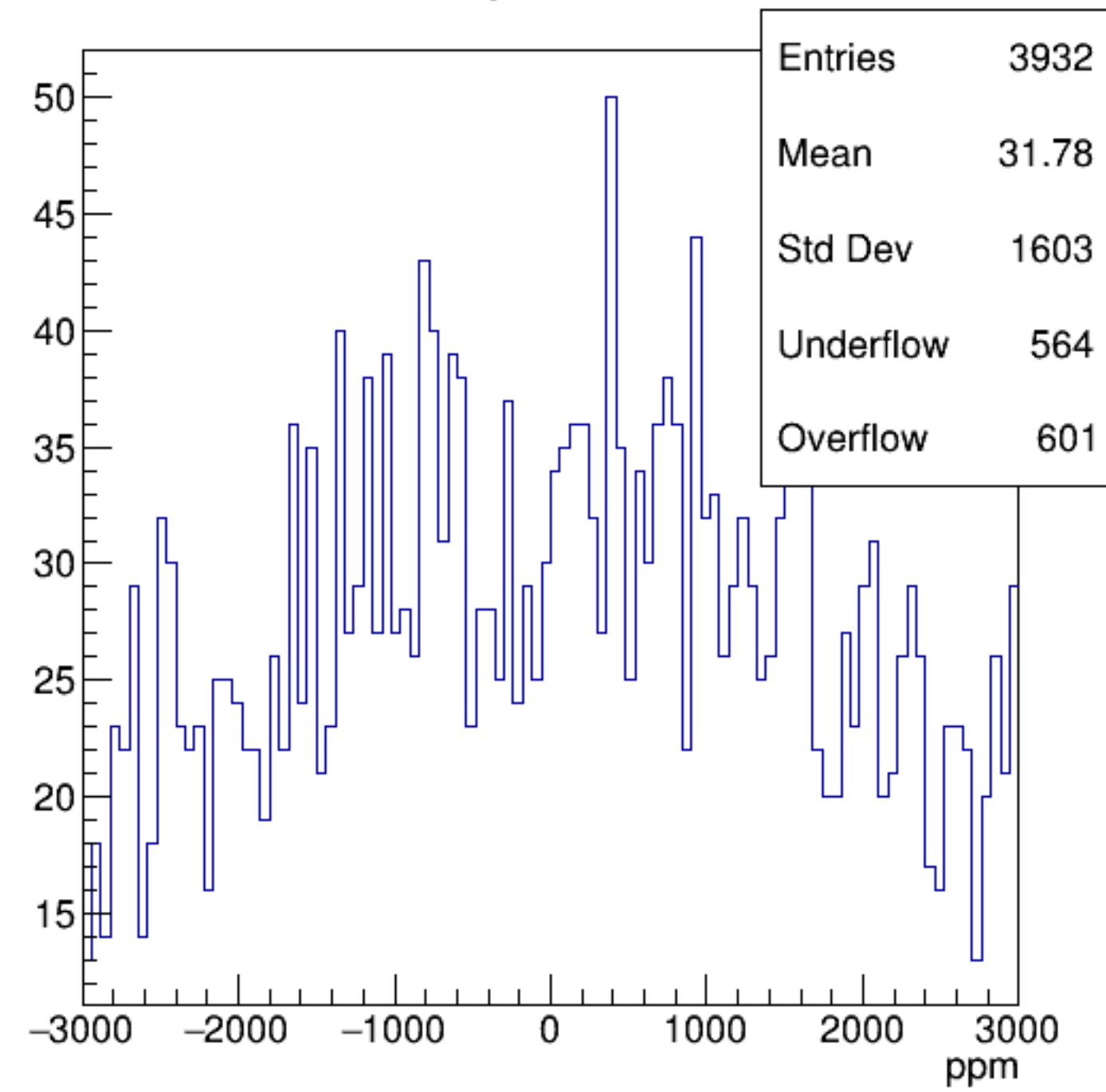
asym_atl1
