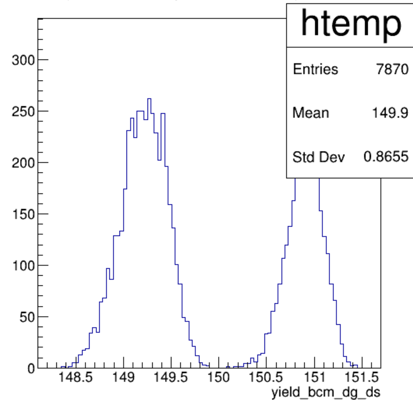
yield_bcm_dg_ds {ErrorFlag==0}
