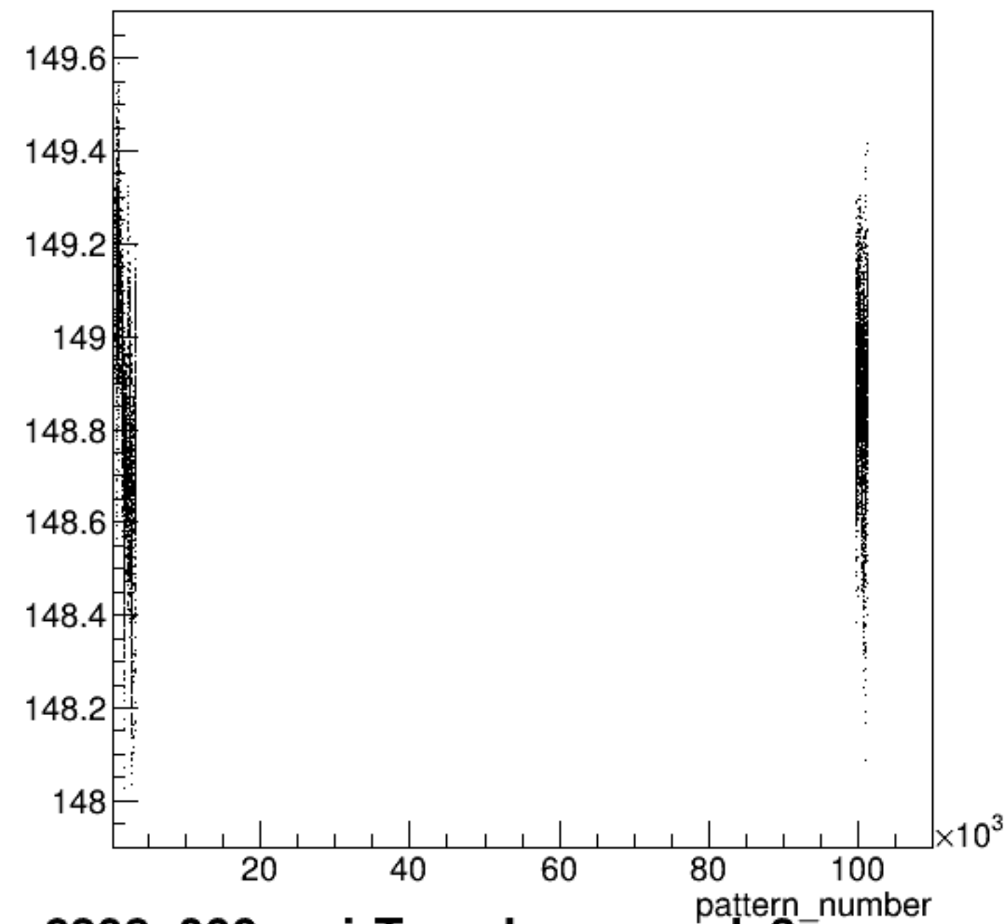
yield_bcm_an_ds3:pattern_number {ErrorFlag==0}
