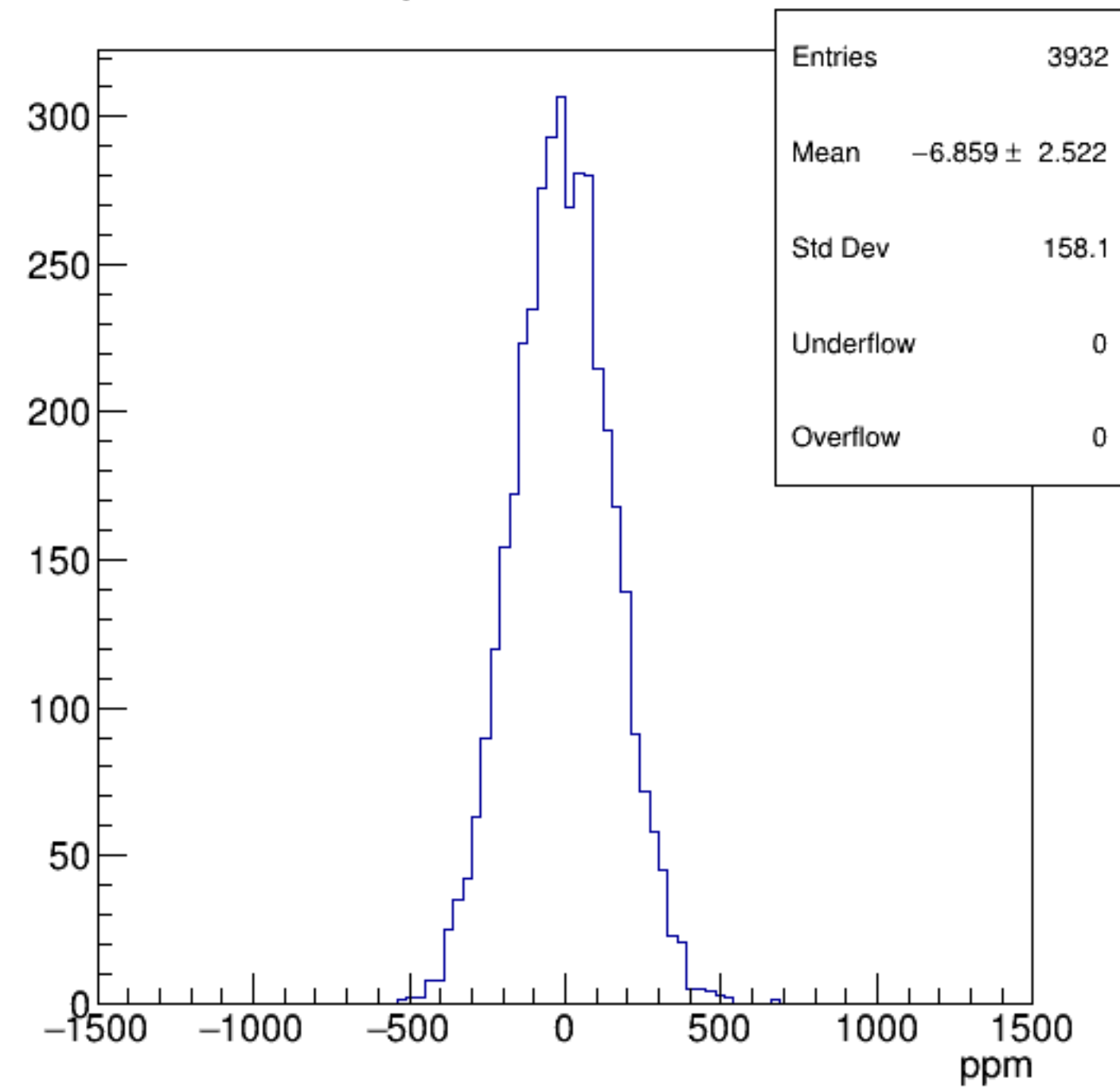
asym_bcm_an_us
