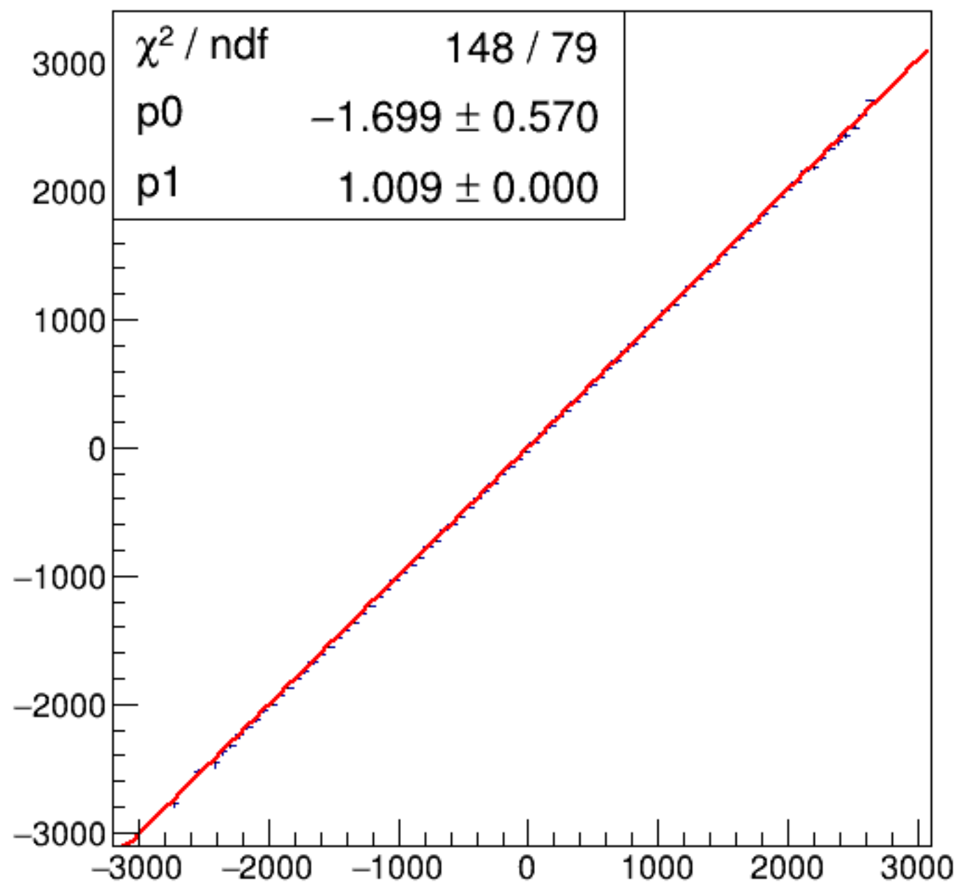
run6398_000_asym_bcm_dg_ds_vs_asym_bcm_an_us_pr.png
