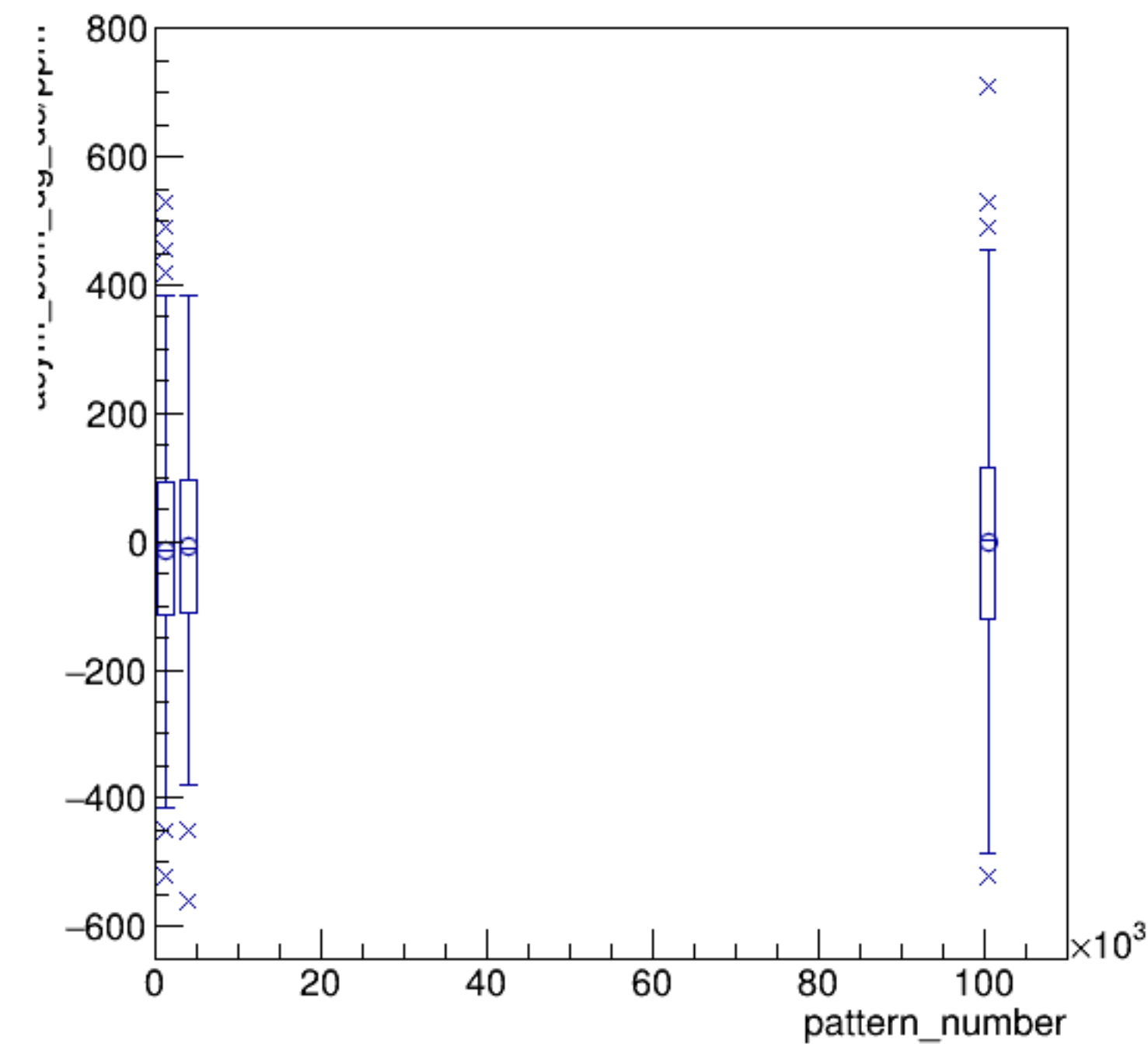
asym_bcm_dg_ds/ppm:pattern_number {ErrorFlag==0}
