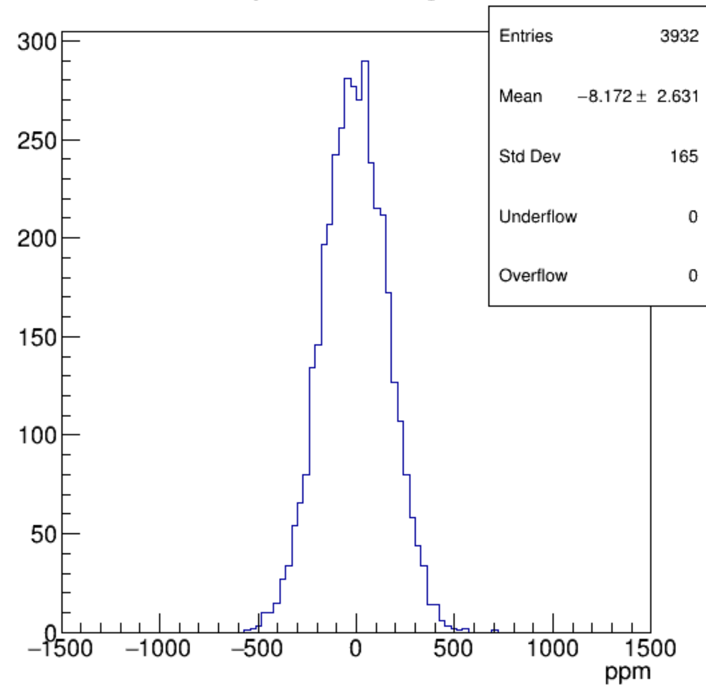
asym_bcm_dg_us
