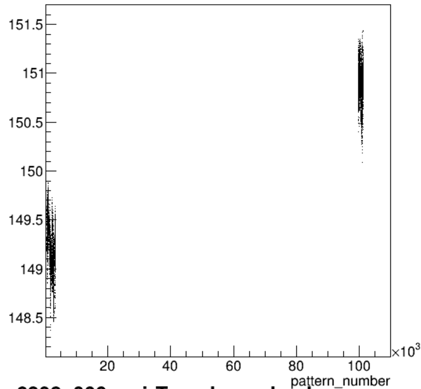
yield_bcm_dg_ds:pattern_number {ErrorFlag==0}
