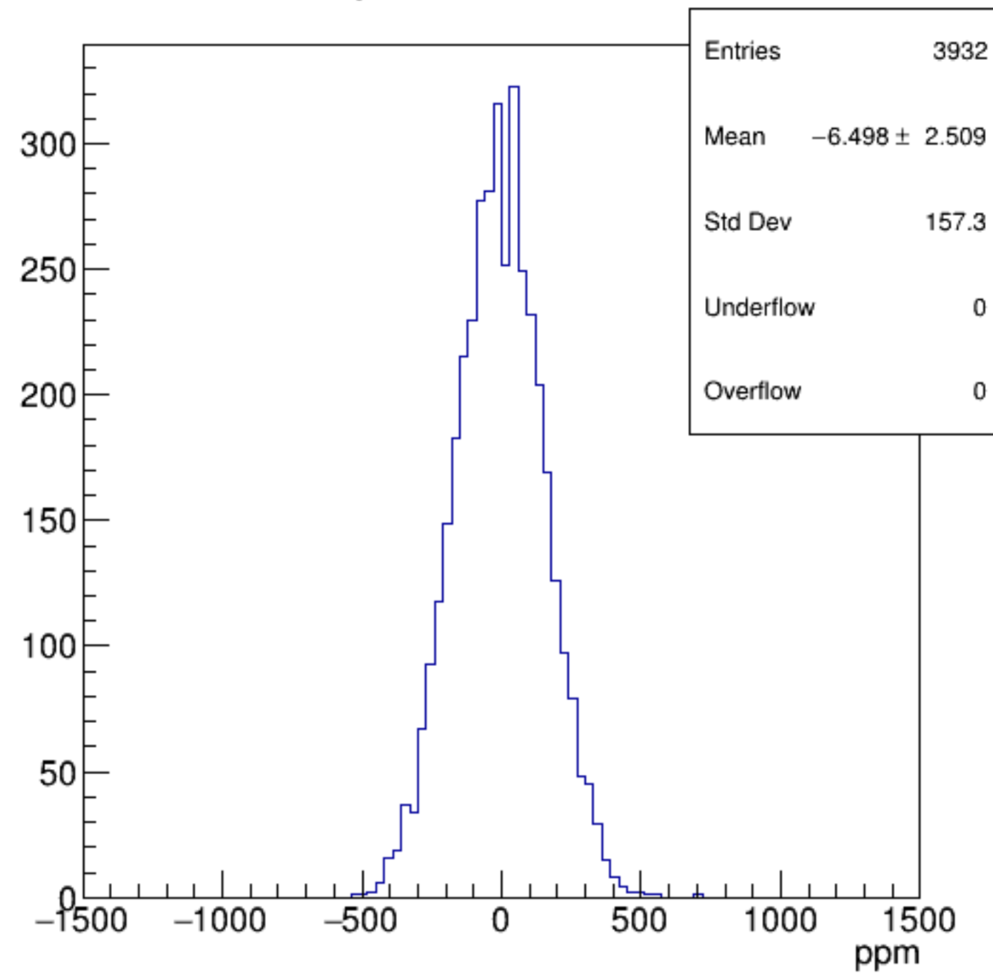
asym_bcm_an_ds
