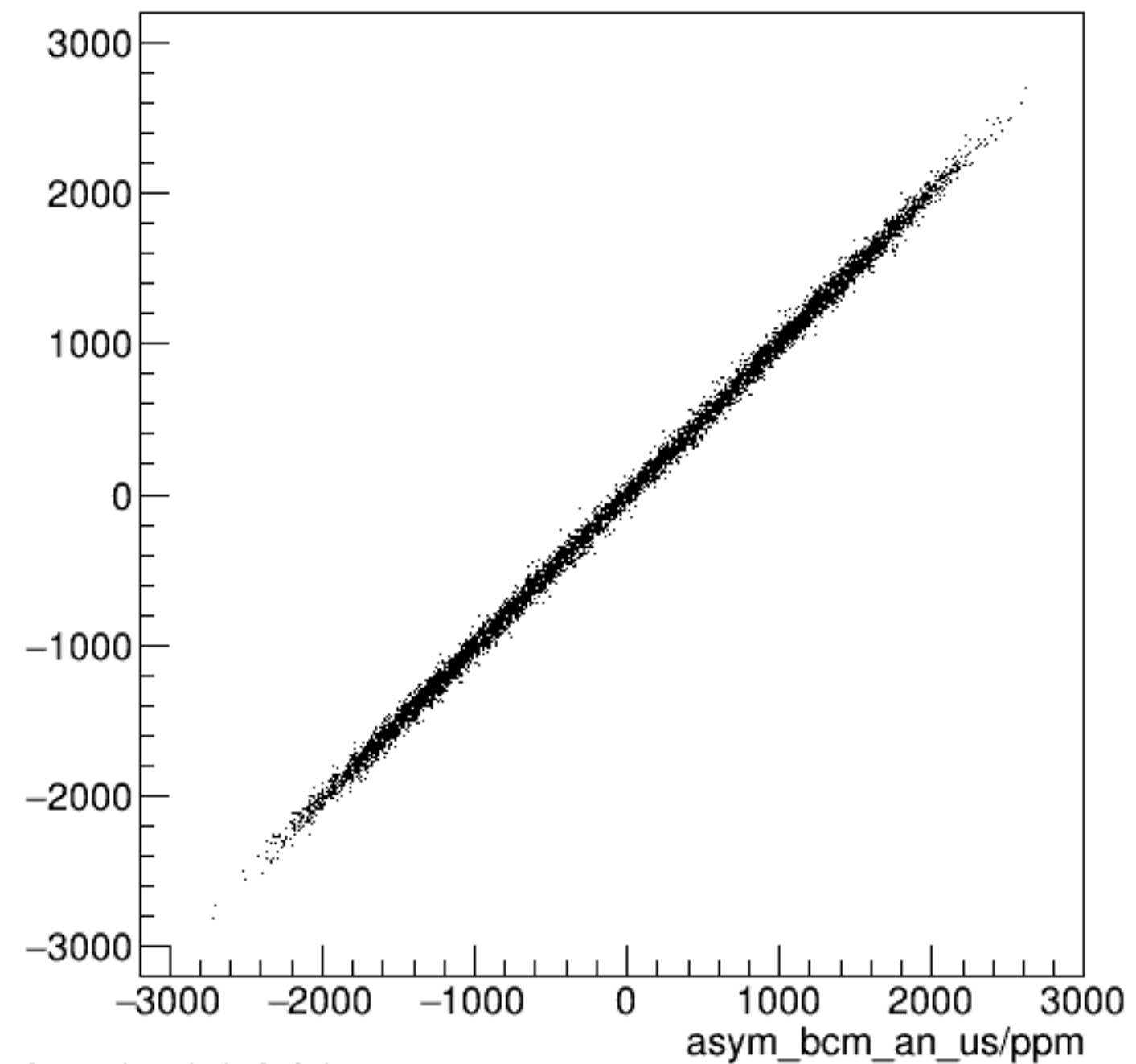
run6398_000_asym_bcm_dg_ds_vs_asym_bcm_an_us_pr.png
