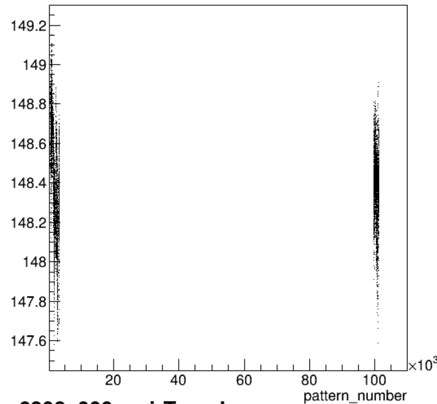
yield_bcm_an_us:pattern_number {ErrorFlag==0}
