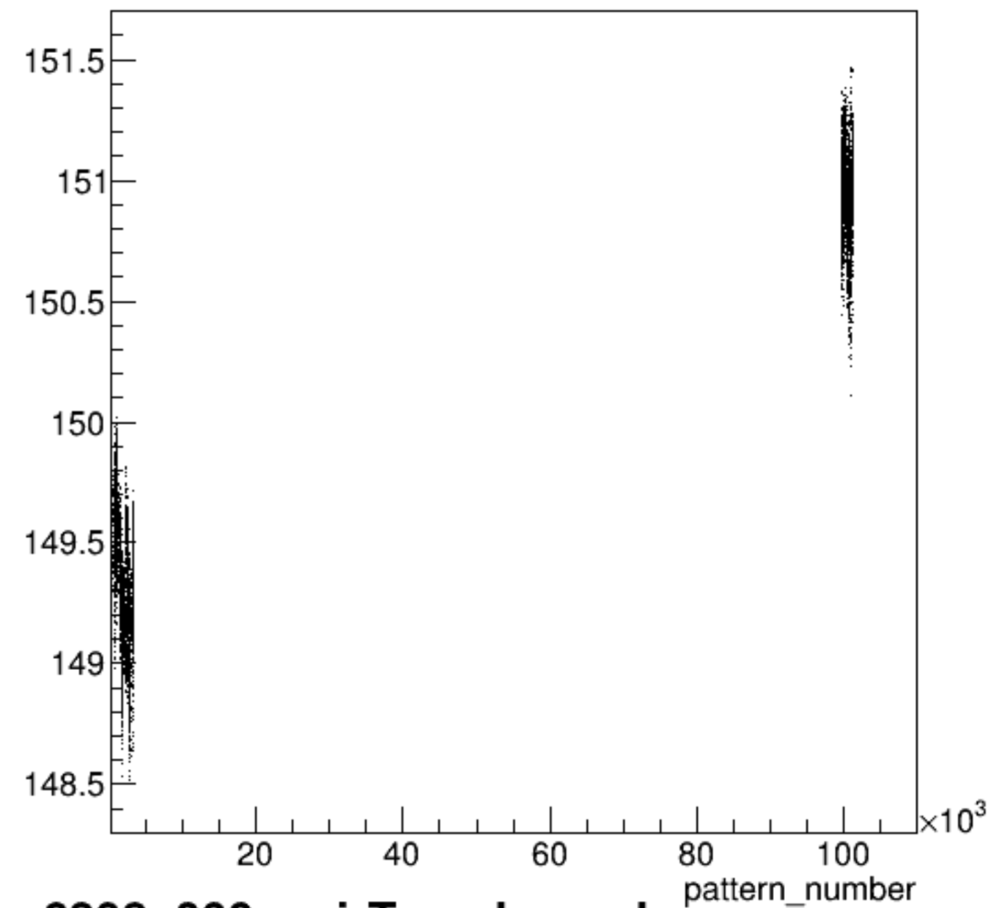
yield_bcm_dg_us:pattern_number {ErrorFlag==0}
