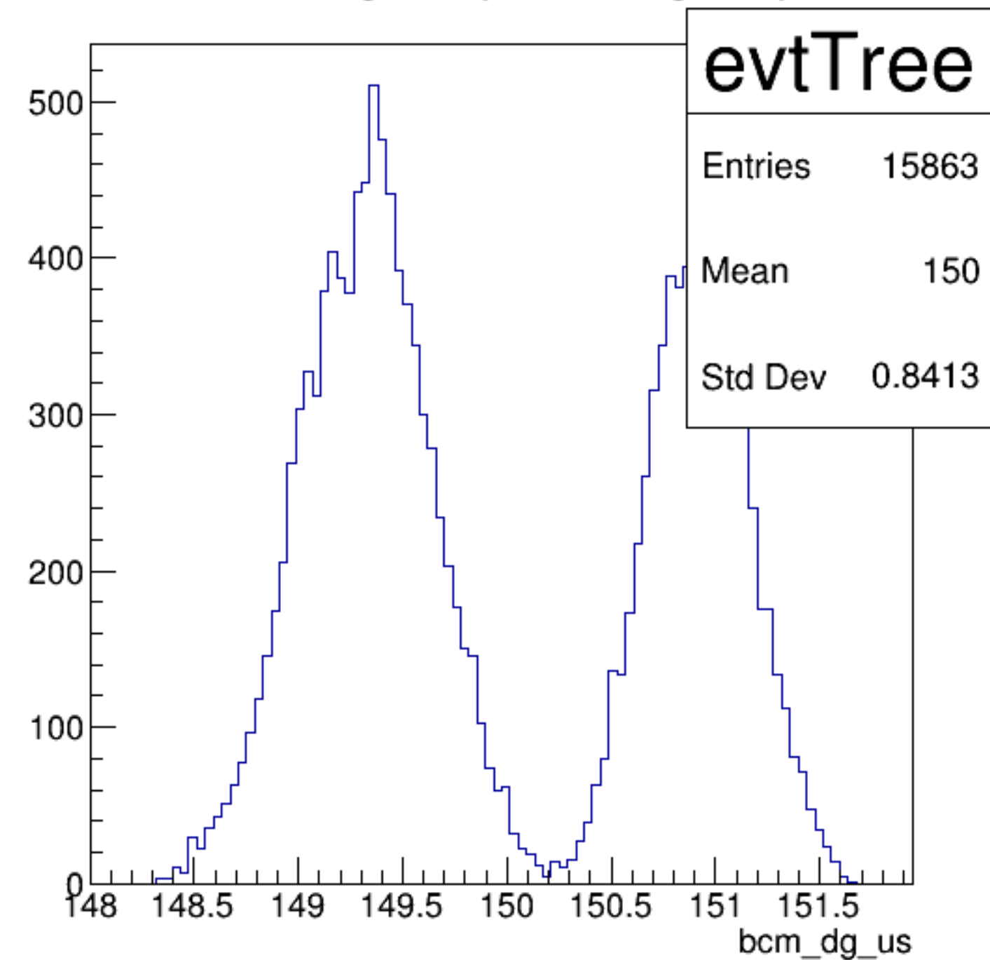
bcm_dg_us {ErrorFlag==0}
