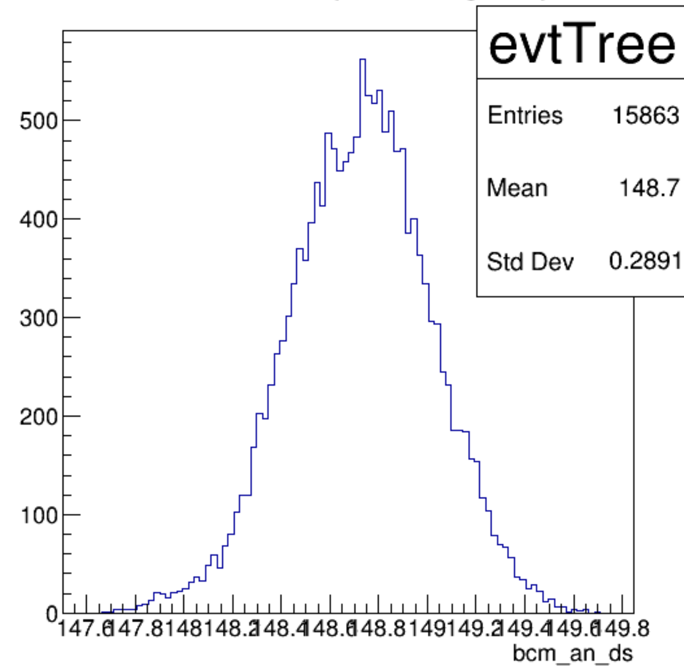
bcm_an_ds {ErrorFlag==0}
