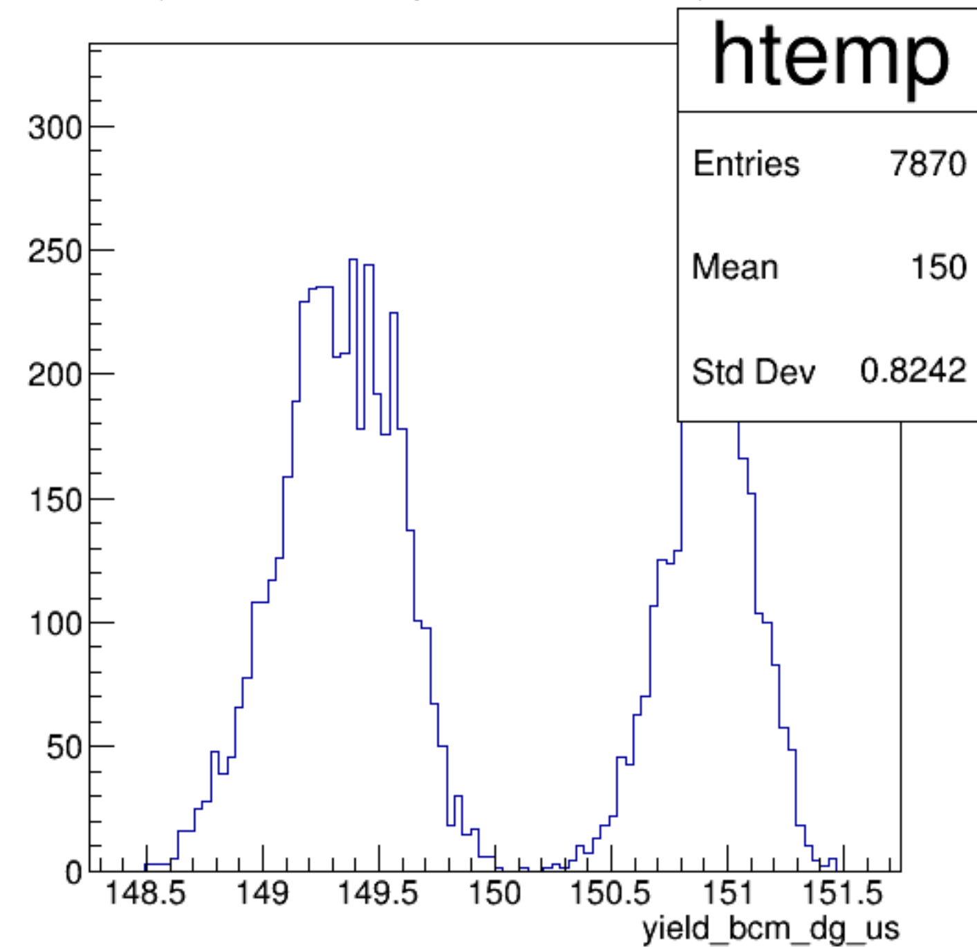
yield_bcm_dg_us {ErrorFlag==0}
