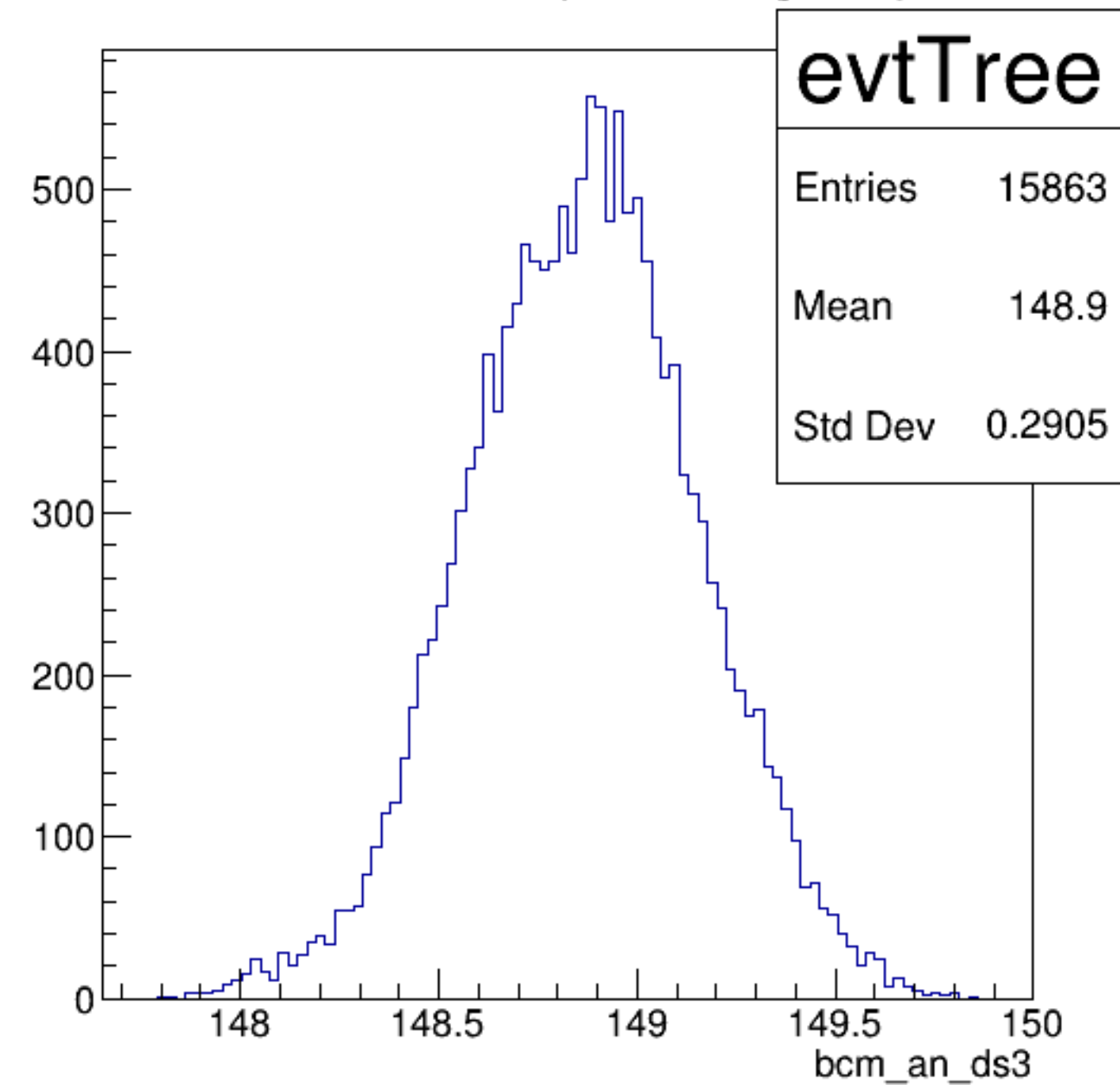
bcm_an_ds3 {ErrorFlag==0}
