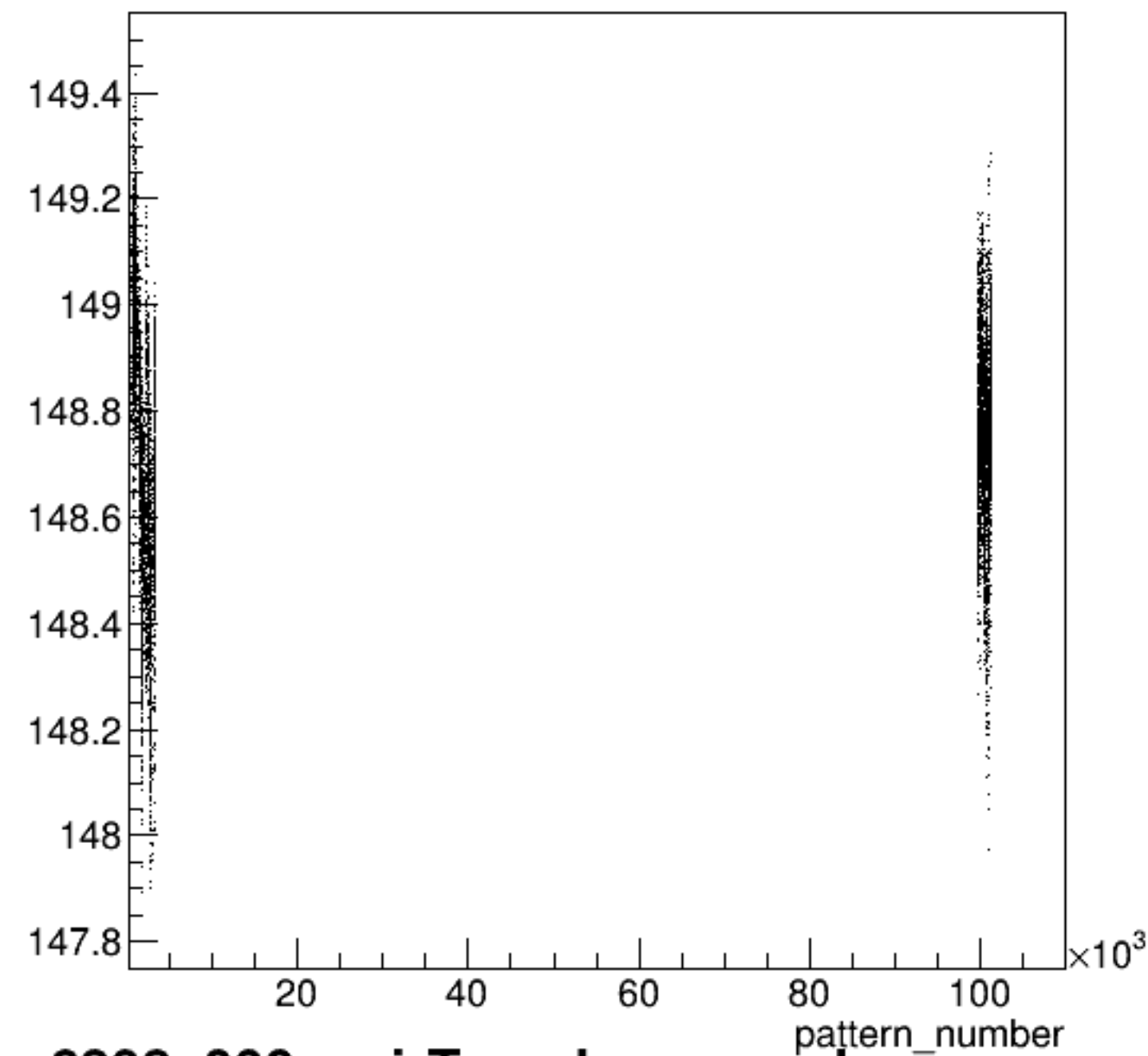
yield_bcm_an_ds:pattern_number {ErrorFlag==0}
