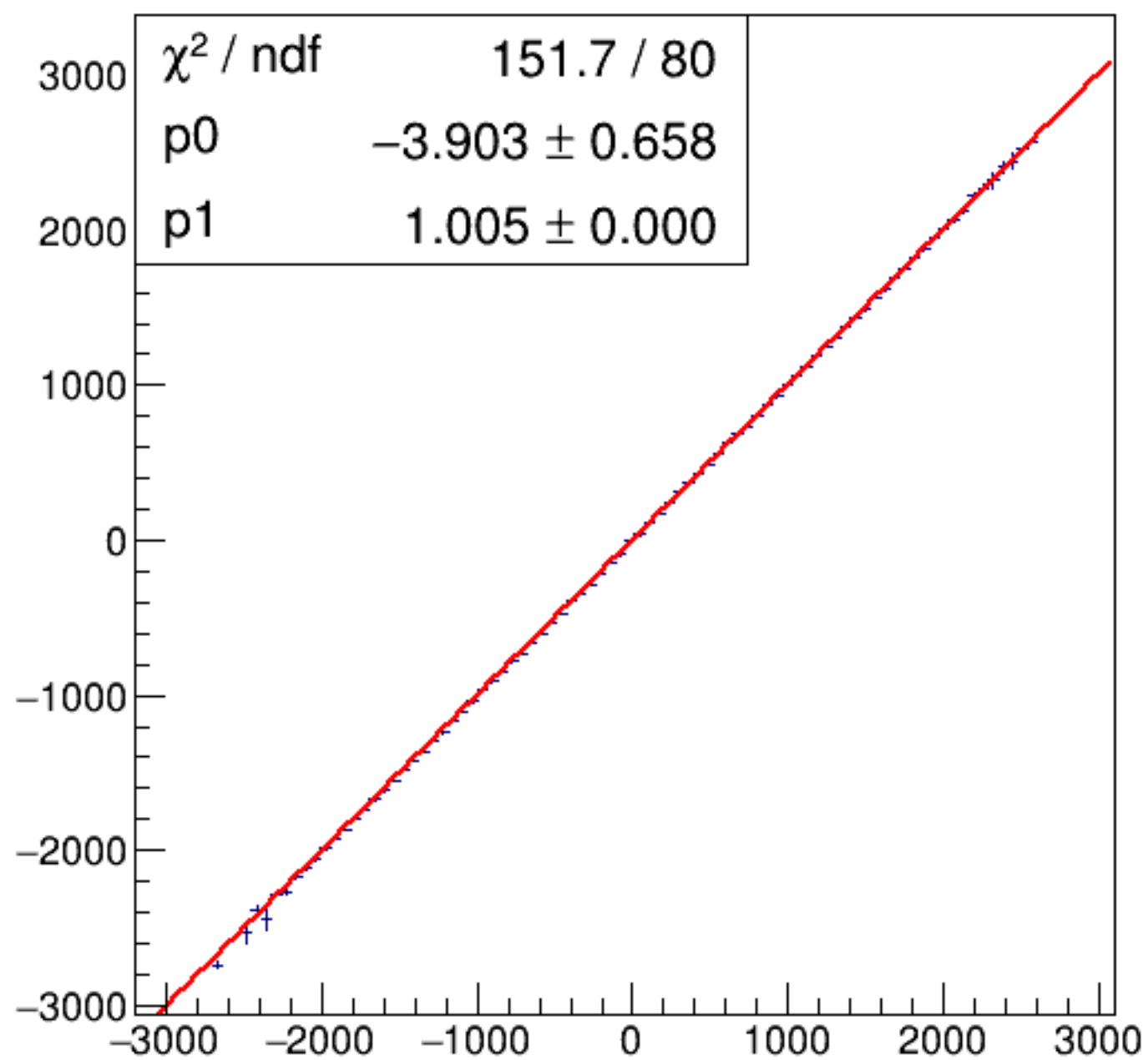
run6398_000_asym_bcm_dg_us_vs_asym_bcm_an_ds_pr.png
