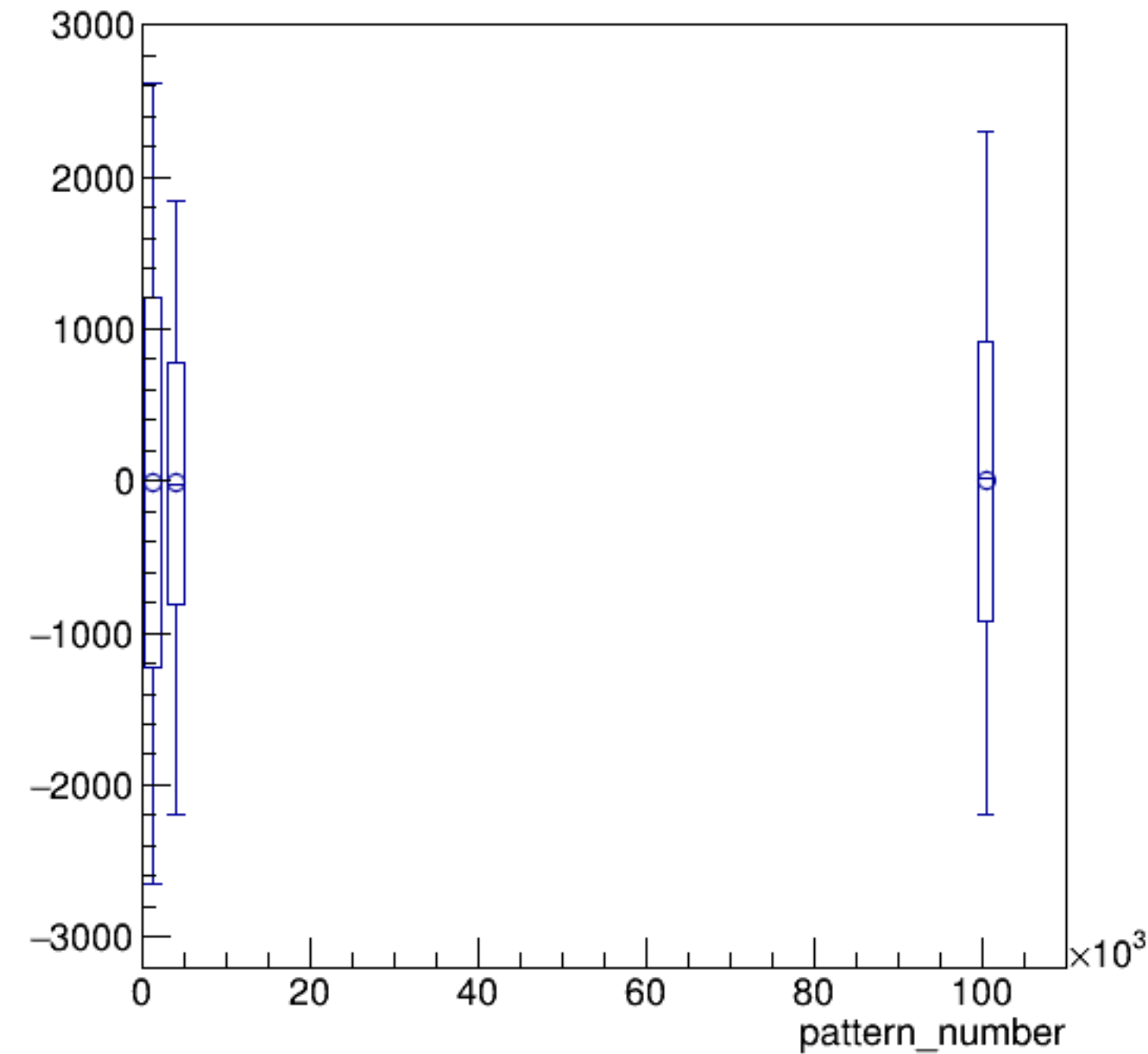
asym_bcm_an_ds/ppm:pattern_number {ErrorFlag==0}
