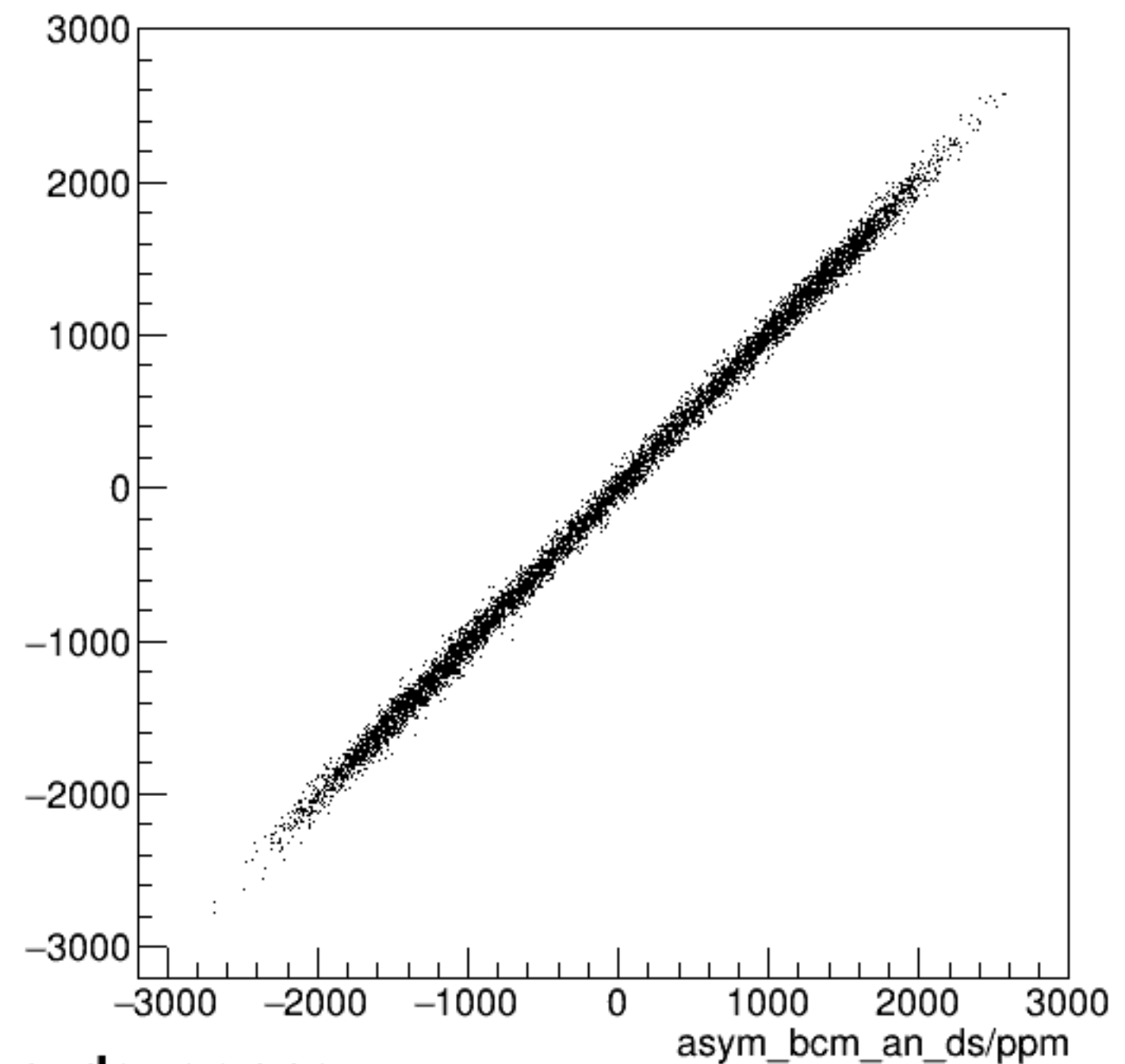
run6398_000_asym_bcm_dg_us_vs_asym_bcm_an_ds_pr.png
