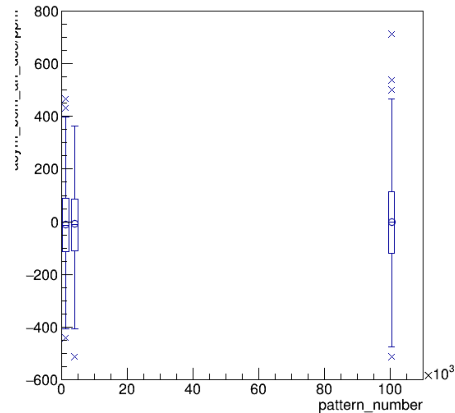
asym_bcm_an_ds3/ppm:pattern_number {ErrorFlag==0}
