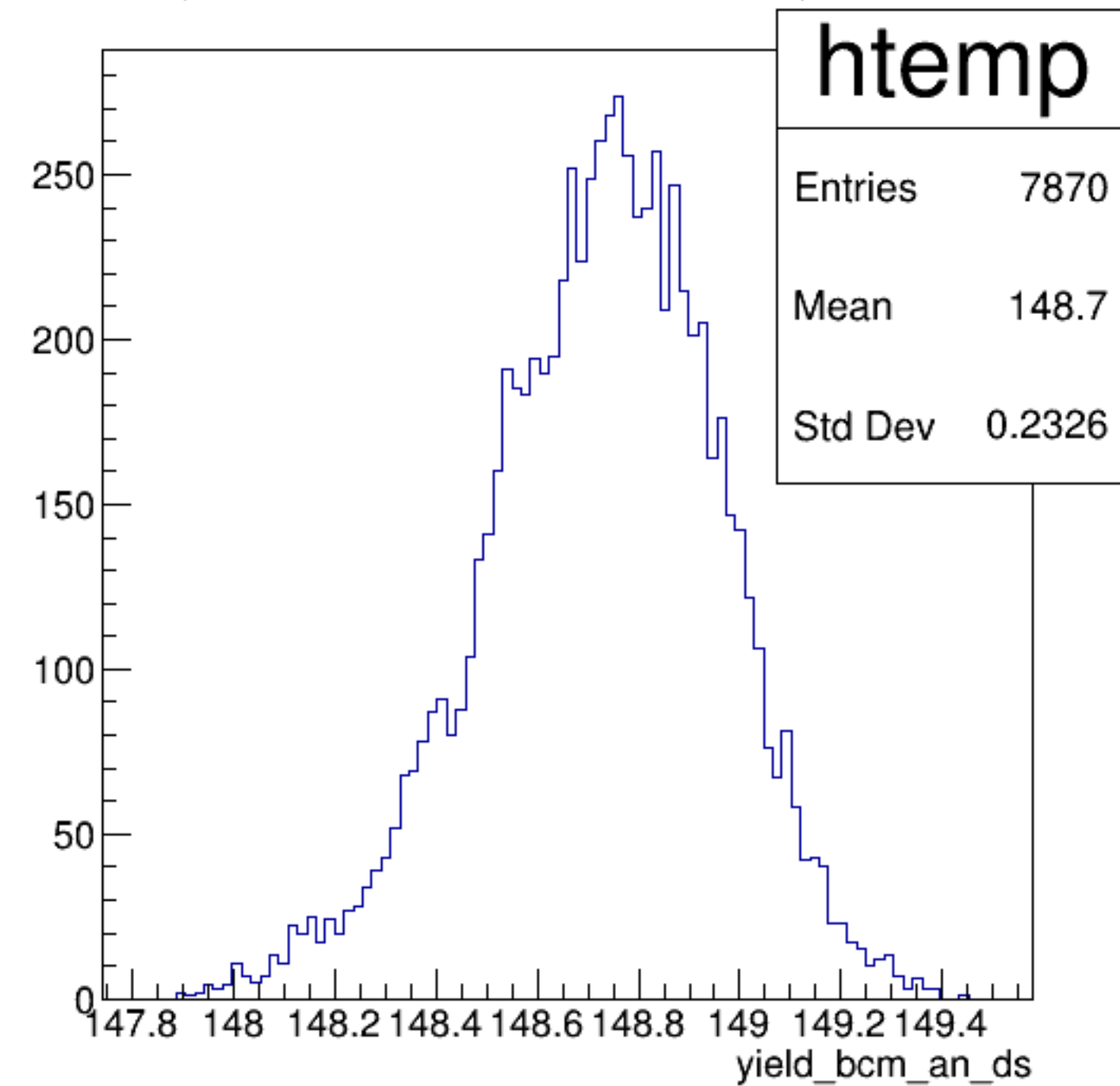
yield_bcm_an_ds {ErrorFlag==0}
