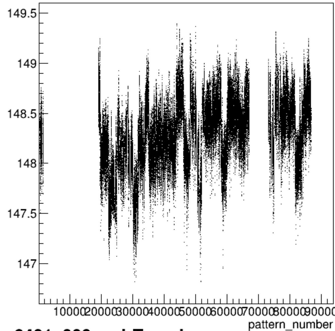
yield_bcm_an_us:pattern_number {ErrorFlag==0}
