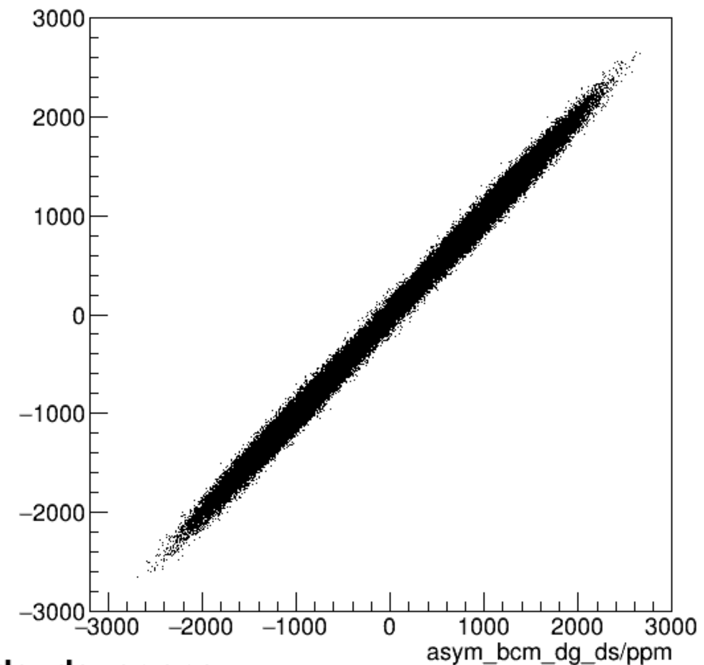
run6401_000_asym_bcm_dg_us_vs_asym_bcm_dg_ds_pr.png
