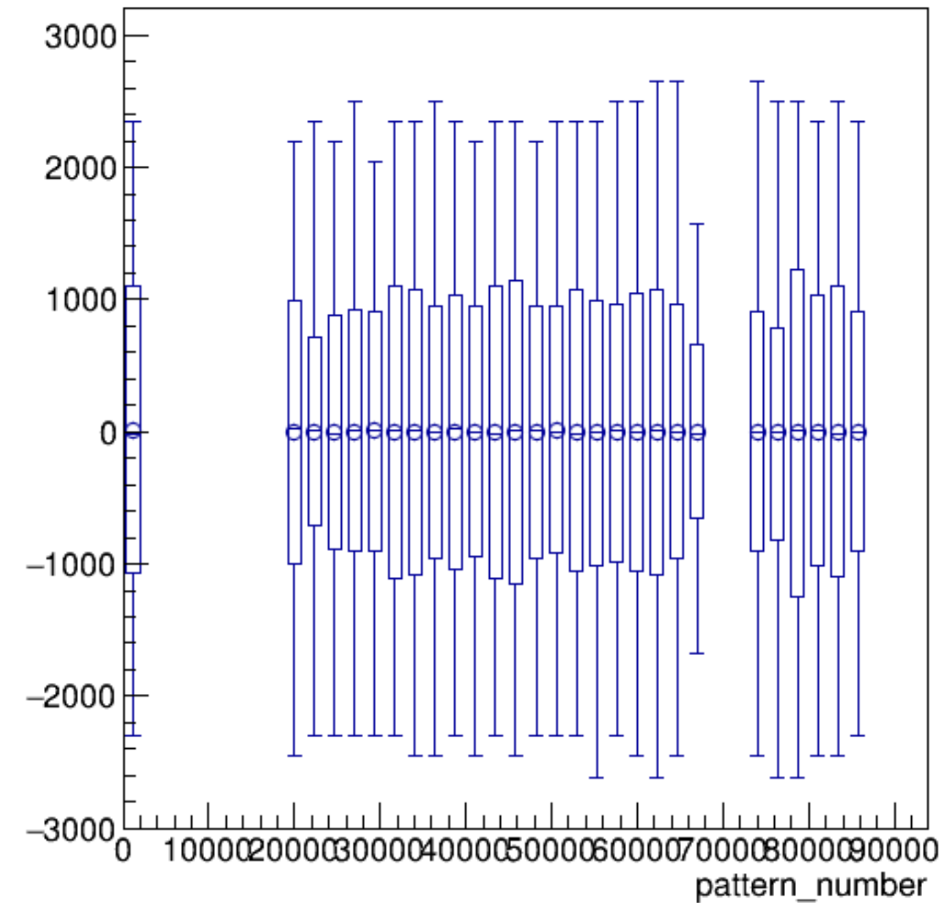
asym_bcm_an_us/ppm:pattern_number {ErrorFlag==0}
