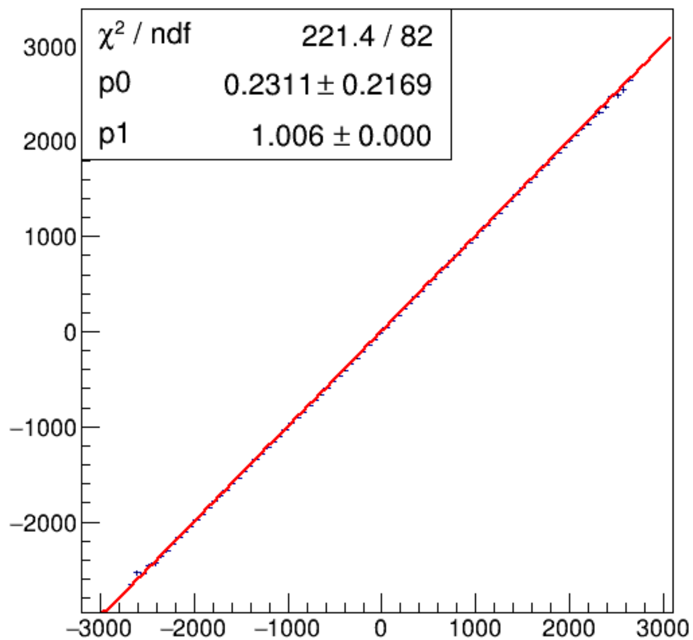
run6401_000_asym_bcm_dg_us_vs_asym_bcm_dg_ds_pr.png
