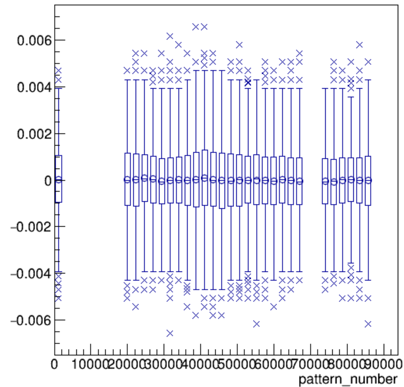
asym_bcm_an_diff*yield_bcm_an_diff:pattern_number {ErrorFlag==0}
