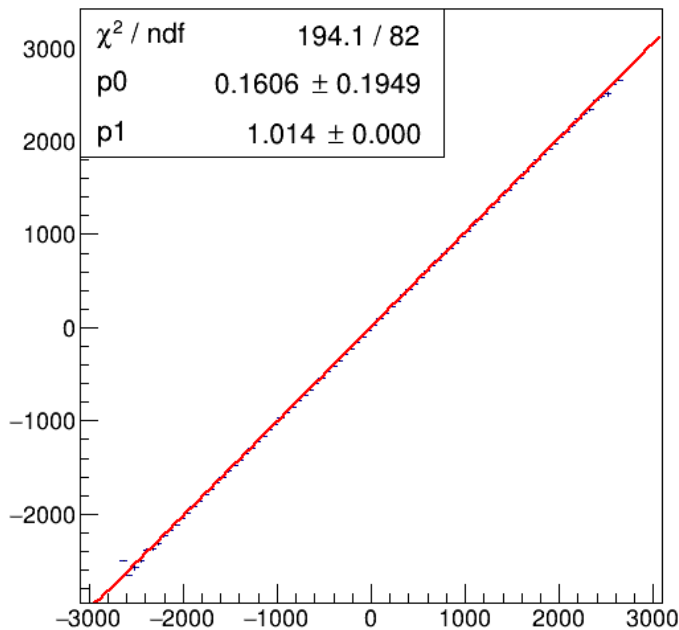
run6401_000_asym_bcm_dg_us_vs_asym_bcm_an_ds_pr.png
