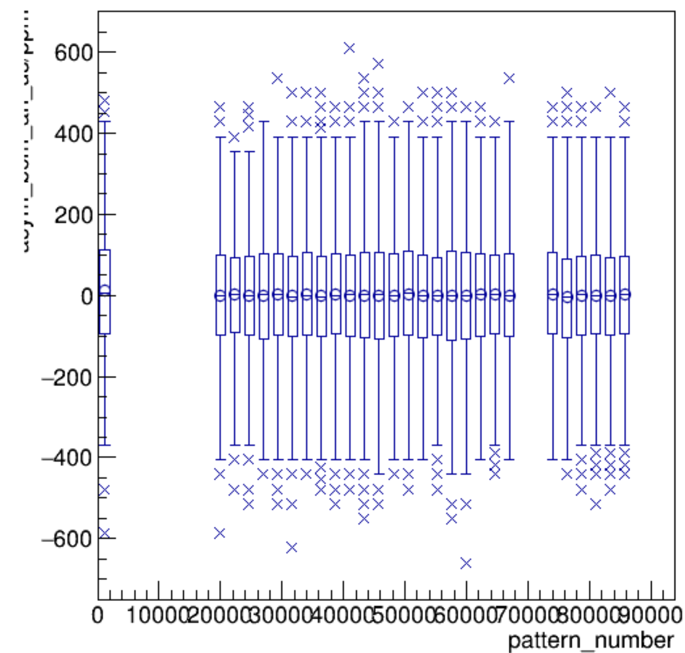
asym_bcm_an_us/ppm:pattern_number {ErrorFlag==0}
