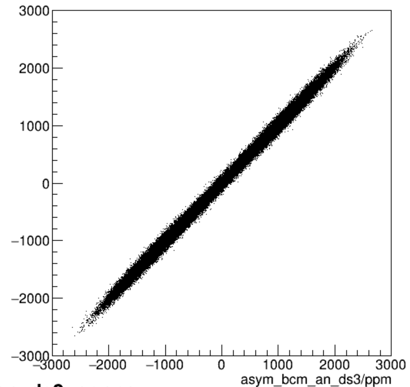
run6401_000_asym_bcm_dg_us_vs_asym_bcm_an_ds3_pr.png
