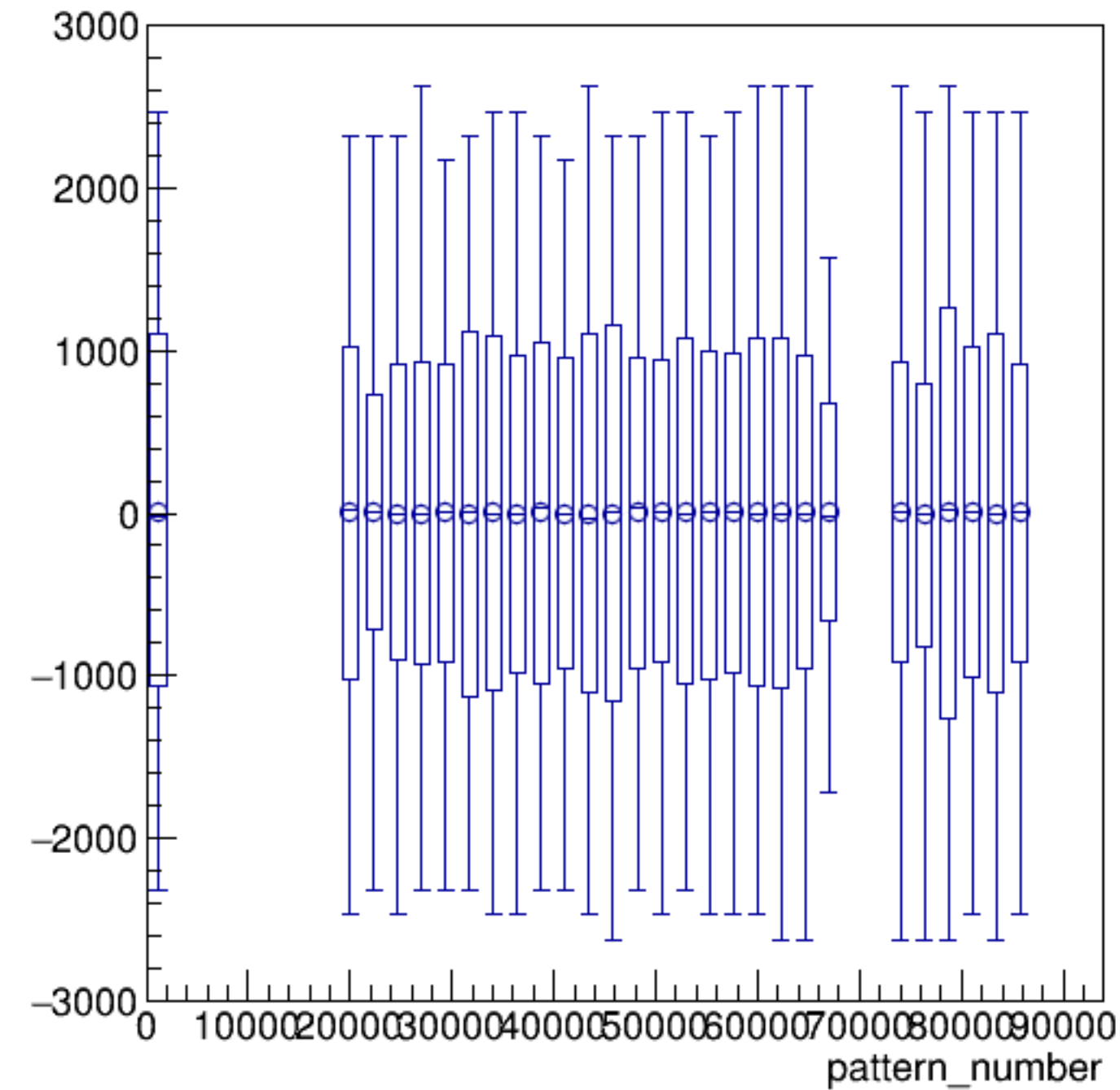
asym_bcm_dg_us/ppm:pattern_number {ErrorFlag==0}
