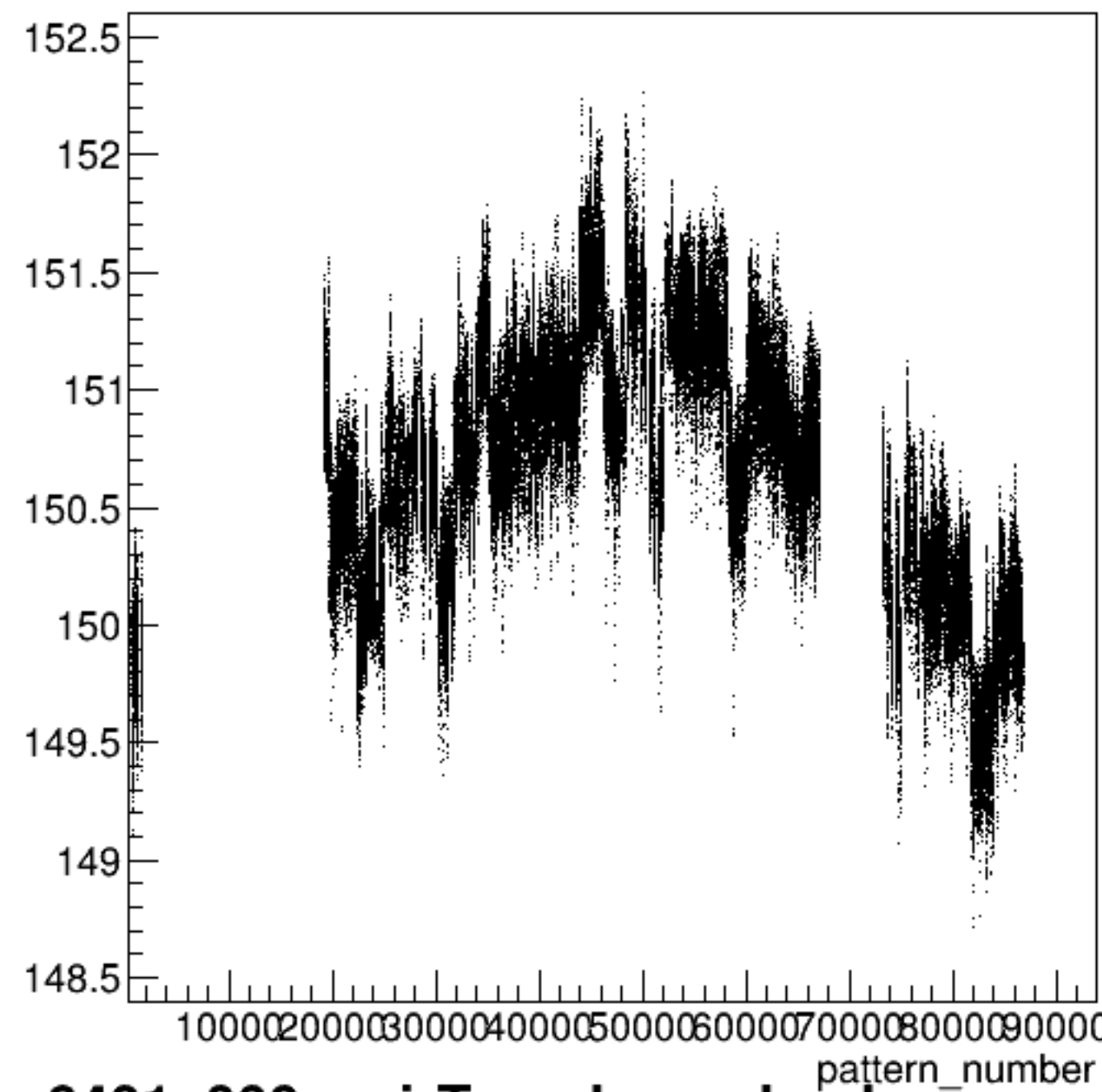
yield_bcm_dg_ds:pattern_number {ErrorFlag==0}
