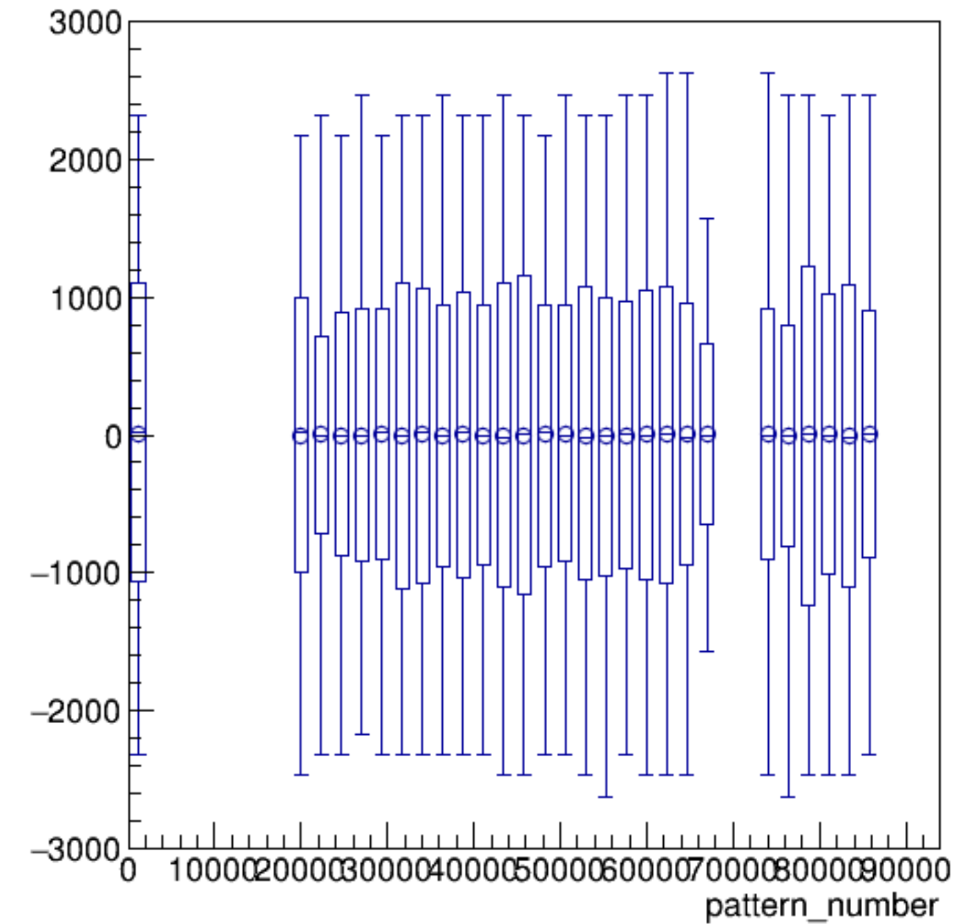
asym_bcm_an_ds3/ppm:pattern_number {ErrorFlag==0}
