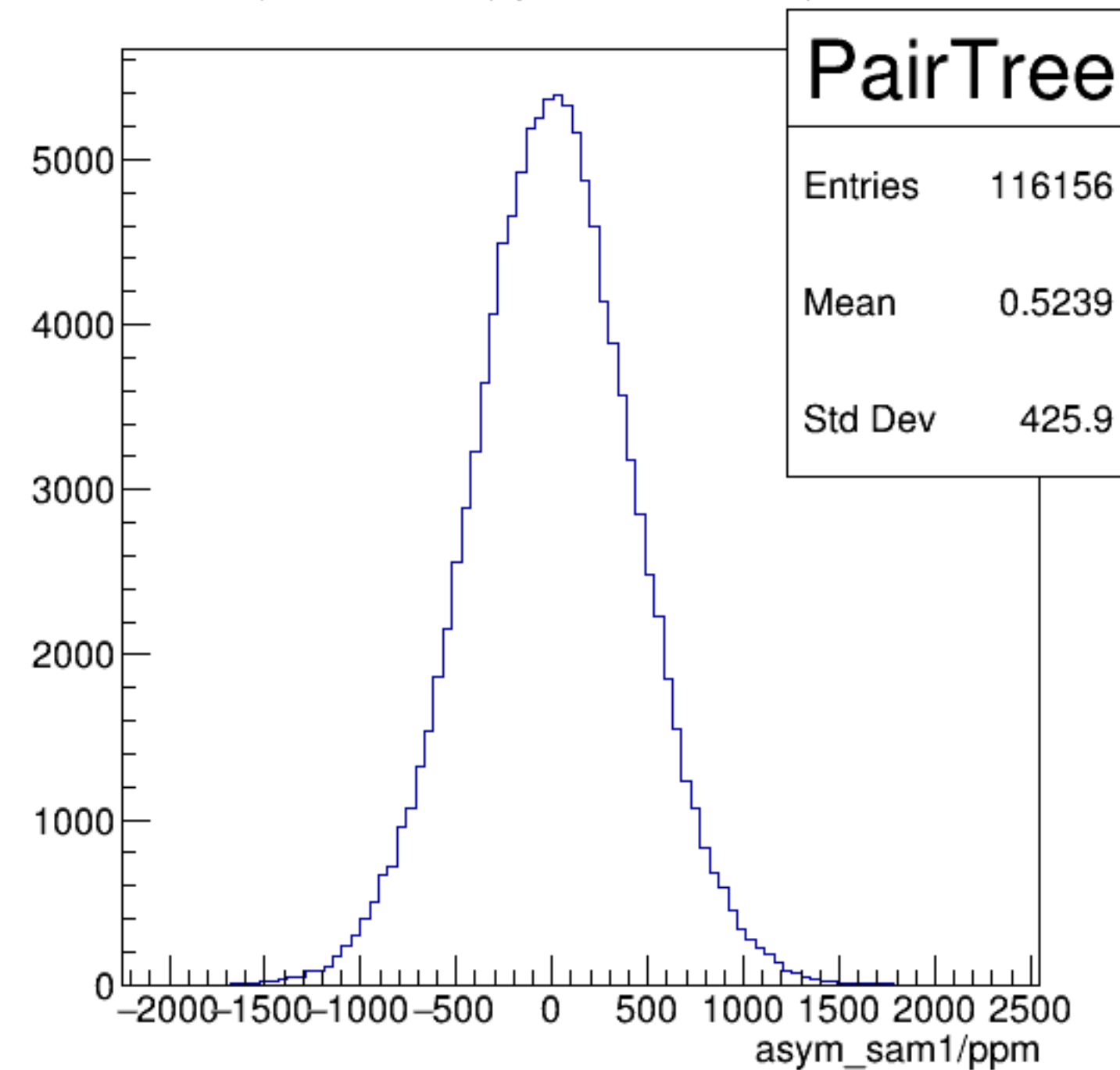
asym_sam1/ppm {ErrorFlag==0}
