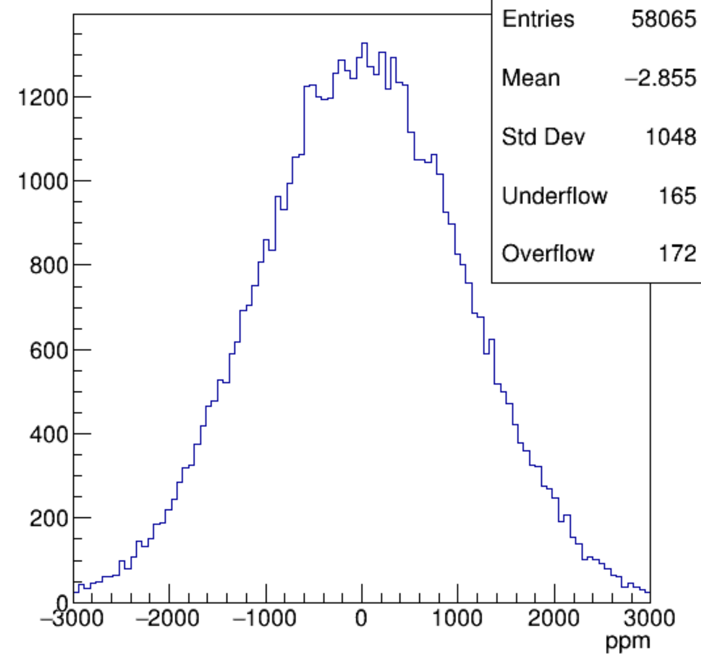
asym_sam6
