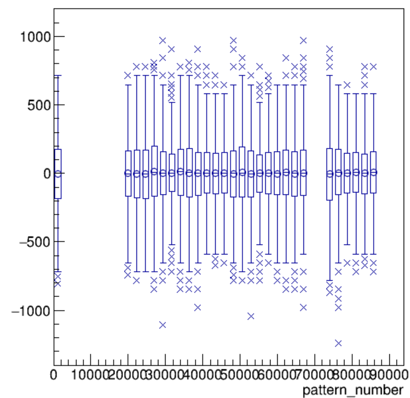
asym_sam8/ppm:pattern_number {ErrorFlag==0}
