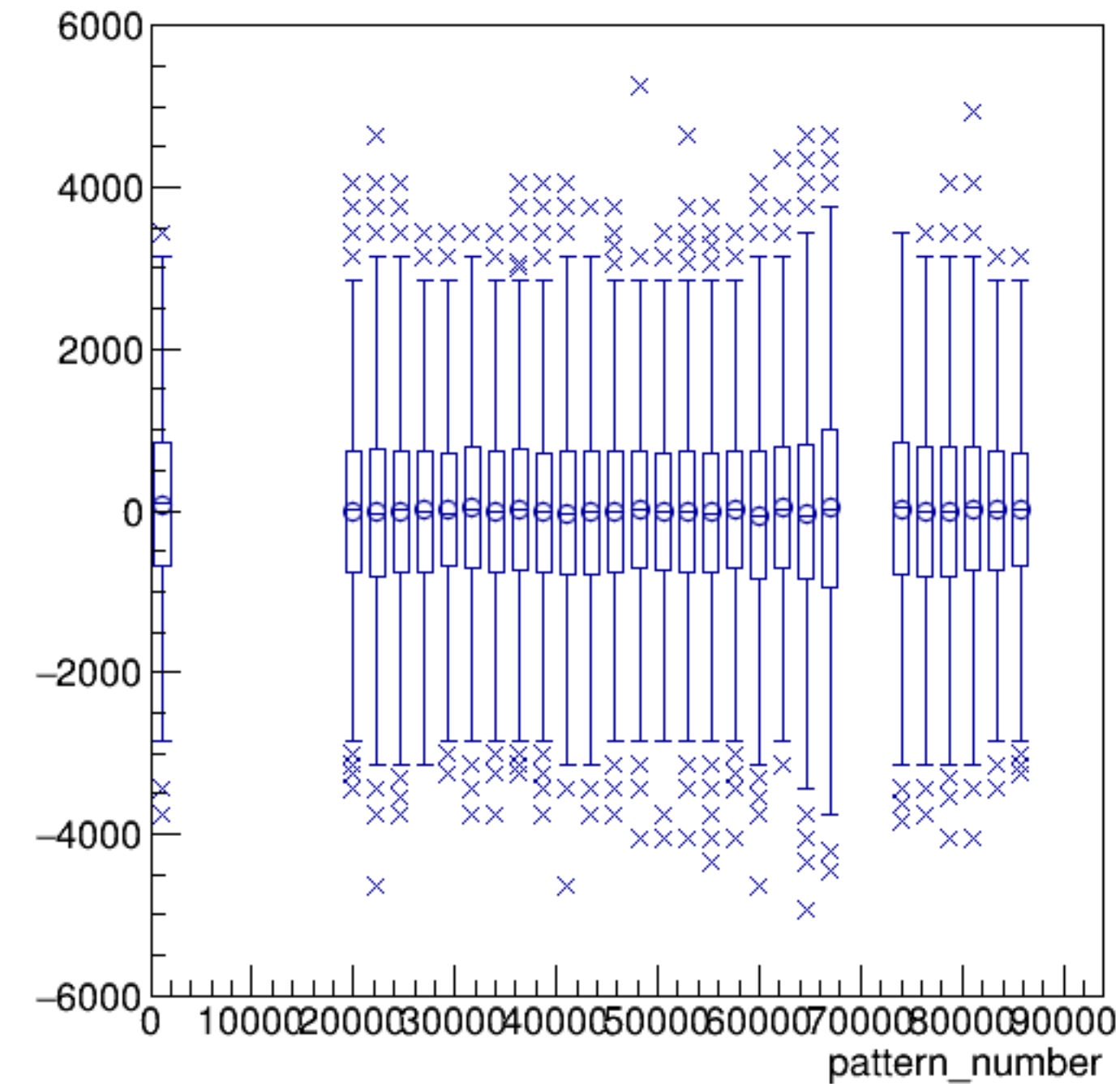
asym_sam5/ppm:pattern_number {ErrorFlag==0}
