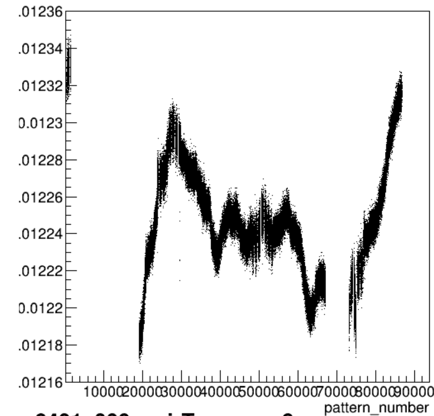
yield_sam8:pattern_number {ErrorFlag==0}
