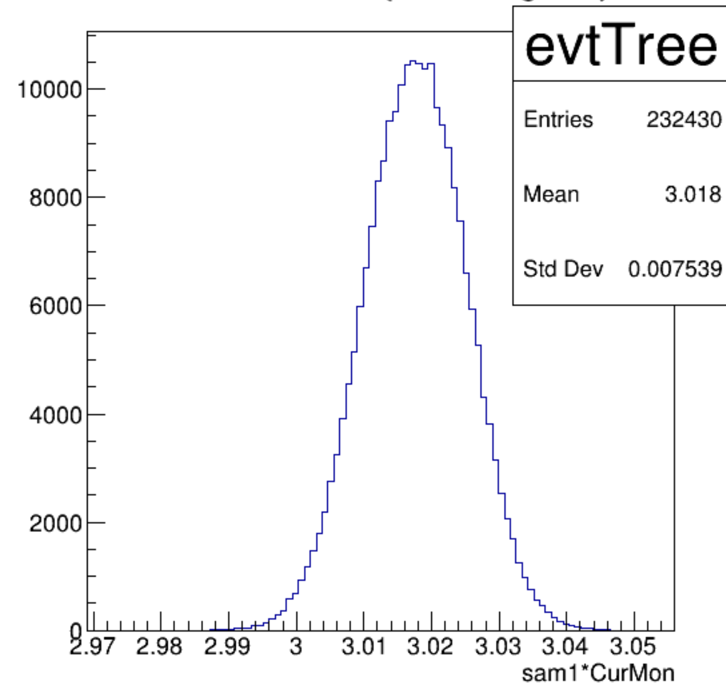
sam1*CurMon {ErrorFlag==0}
