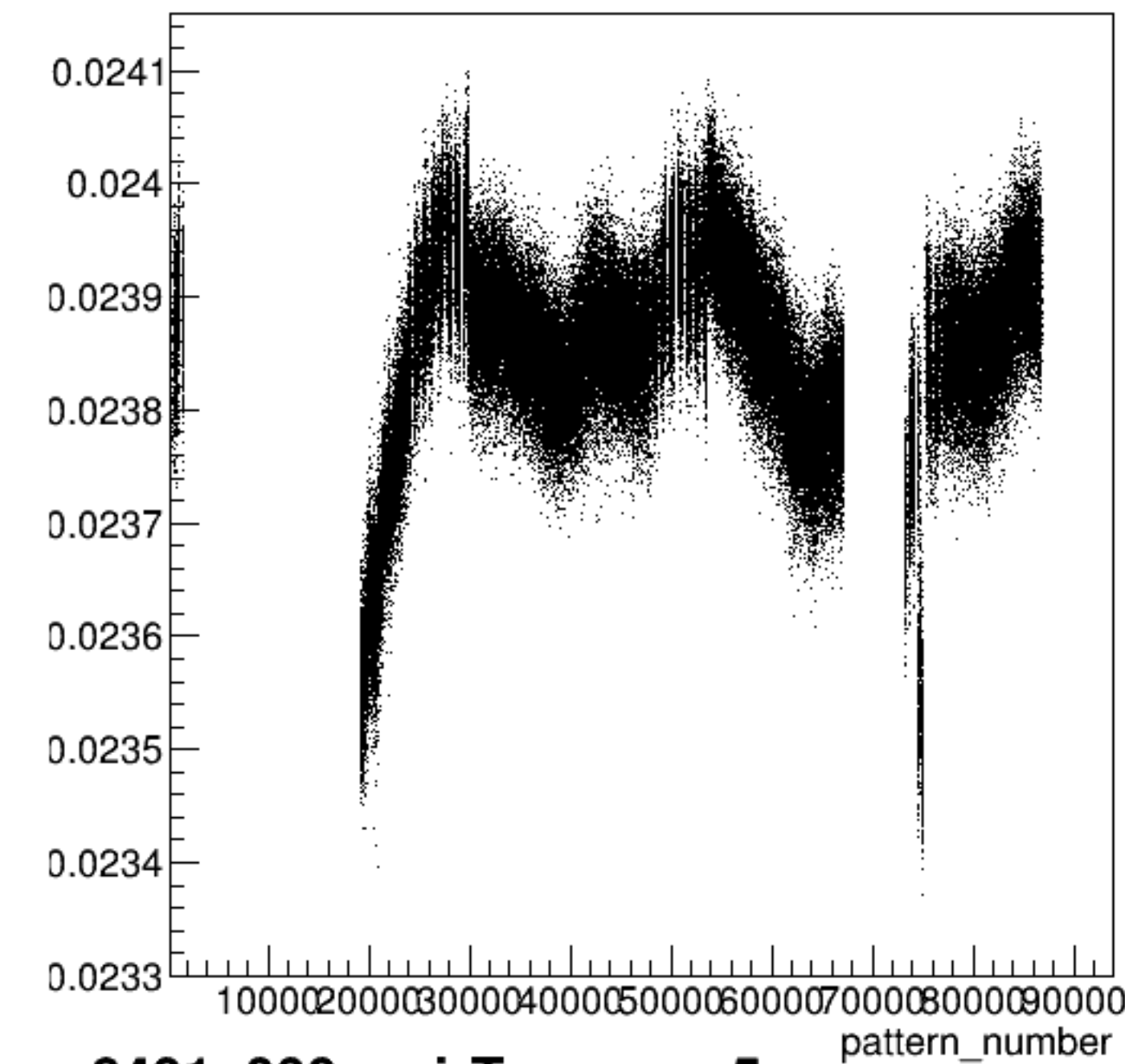
yield_sam5:pattern_number {ErrorFlag==0}
