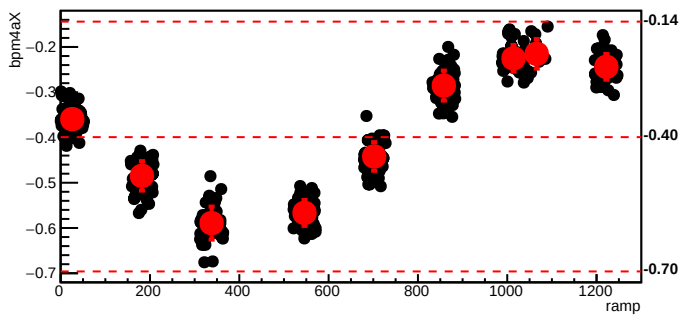
bmod_trim3,cyc=6156
