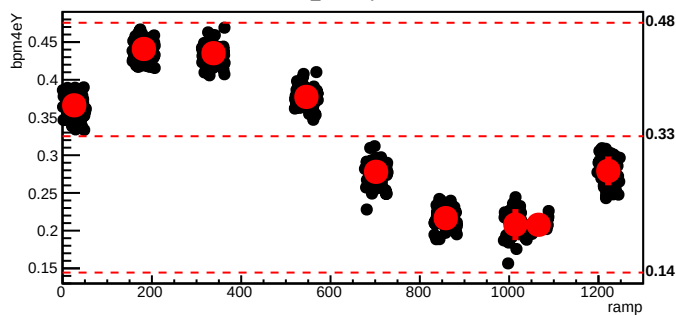
bmod_trim4,cyc=6156
