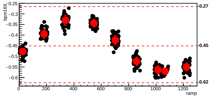
bmod_trim3,cyc=6156
