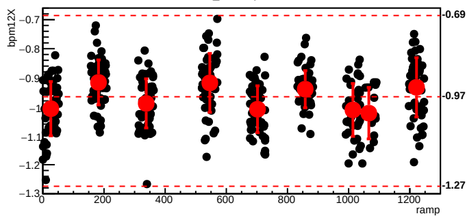
bmod_trim6,cyc=6156
