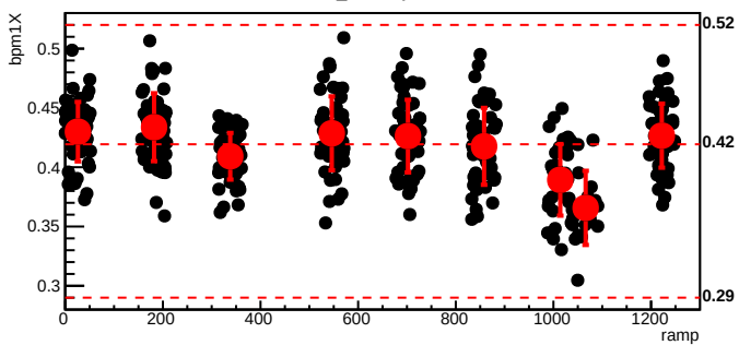
bmod_trim6,cyc=6156
