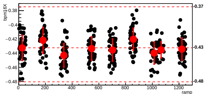
bmod_trim6,cyc=6157
