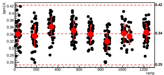
bmod_trim6,cyc=6157
