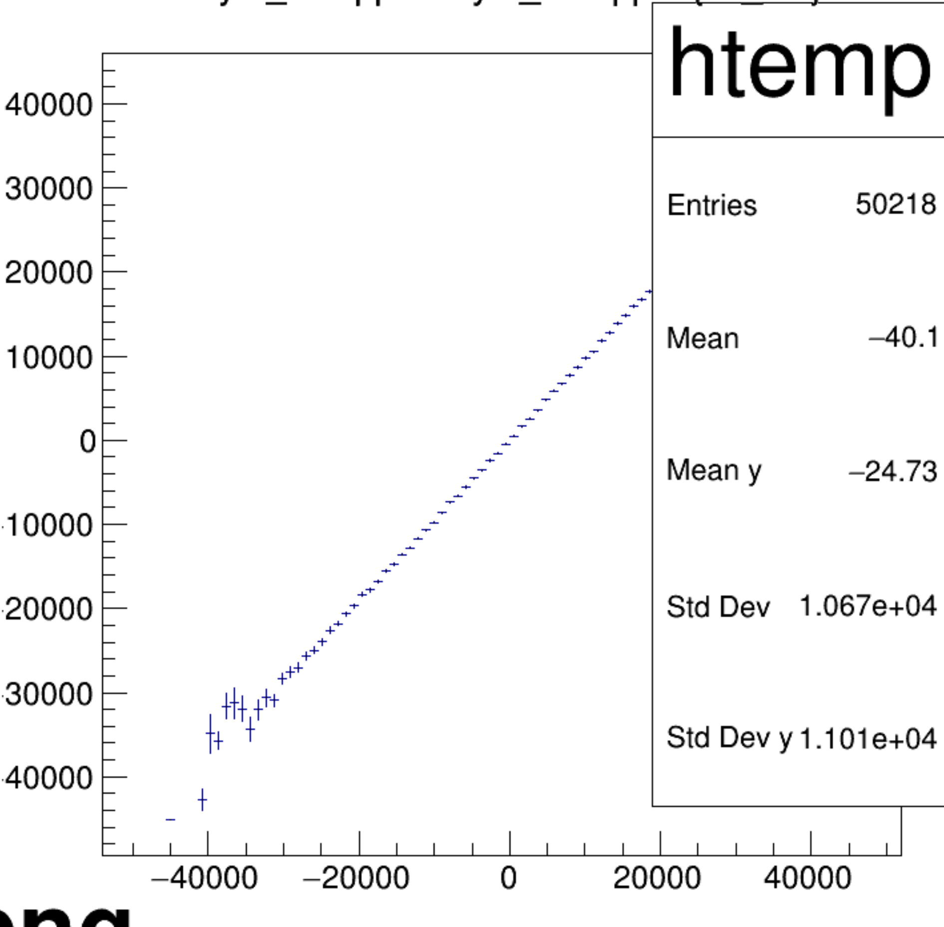
asym_atl2/ppm:asym_atr2/ppm {ok_cut}
