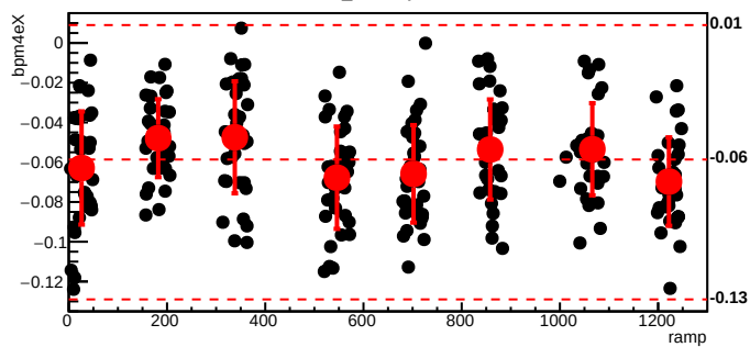
bmod_trim4,cyc=6164
