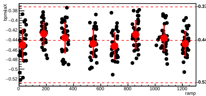
bmod_trim4,cyc=6164
