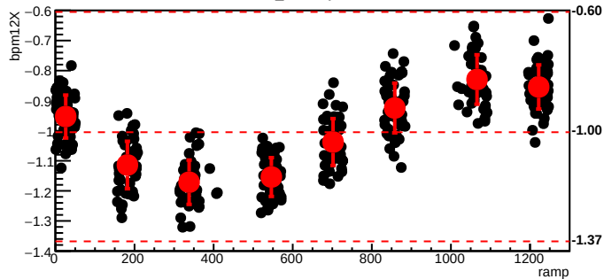
bmod_trim3,cyc=6164
