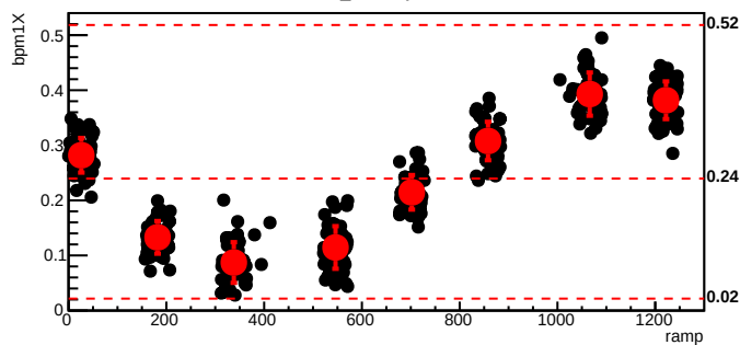
bmod_trim3,cyc=6164
