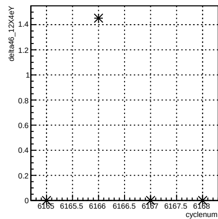
delta46_12X4eY:cyclenum {run == 6404}
