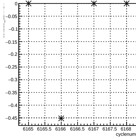
delta13_12X4eX:cyclenum {run == 6404}
