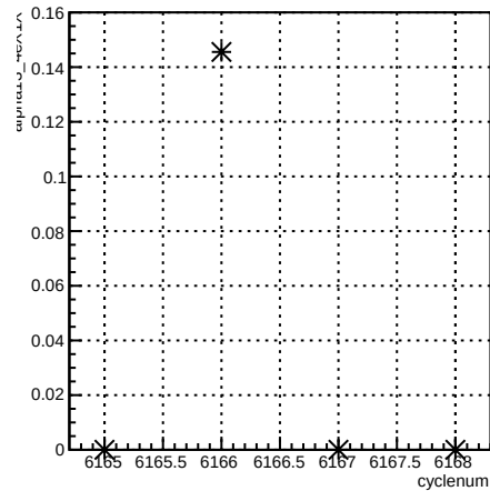
alpha13_4eX1X:cyclenum {run == 6404}
