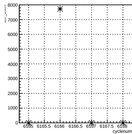
usr_coil4:cyclenum {run == 6404}
