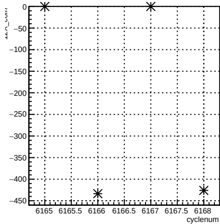
12X_coil7:cyclenum {run == 6404}
