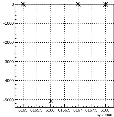
usr_coil3:cyclenum {run == 6404}
