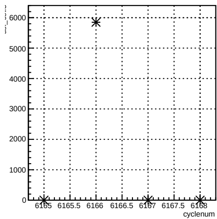
usl_coil3:cyclenum {run == 6404}
