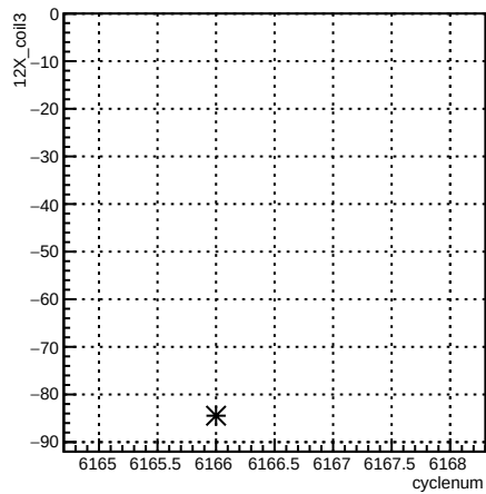
12X_coil3:cyclenum {run == 6404}
