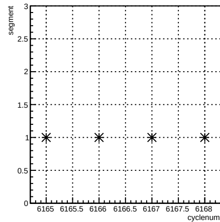
segment:cyclenum {run == 6404}
