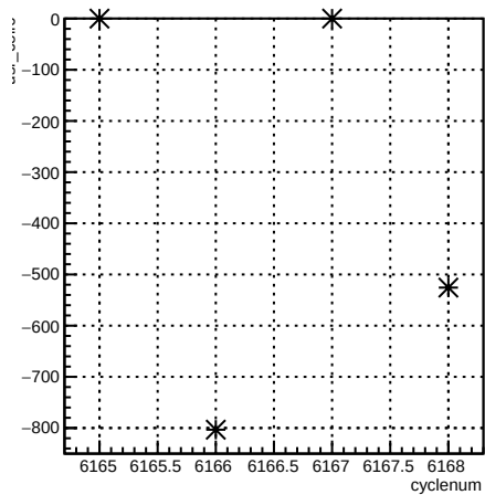
usr_coil6:cyclenum {run == 6404}
