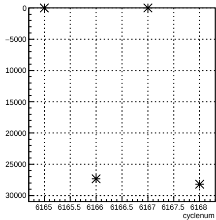
usr_coil1:cyclenum {run == 6404}
