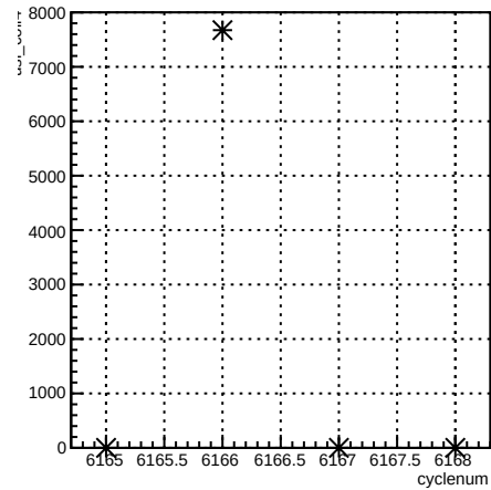
usl_coil4:cyclenum {run == 6404}
