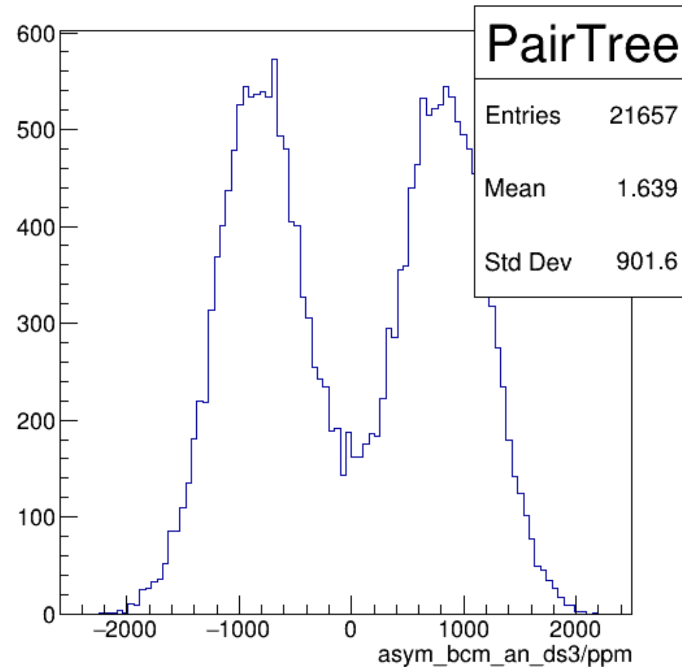
asym_bcm_an_ds3/ppm {ErrorFlag==0}
