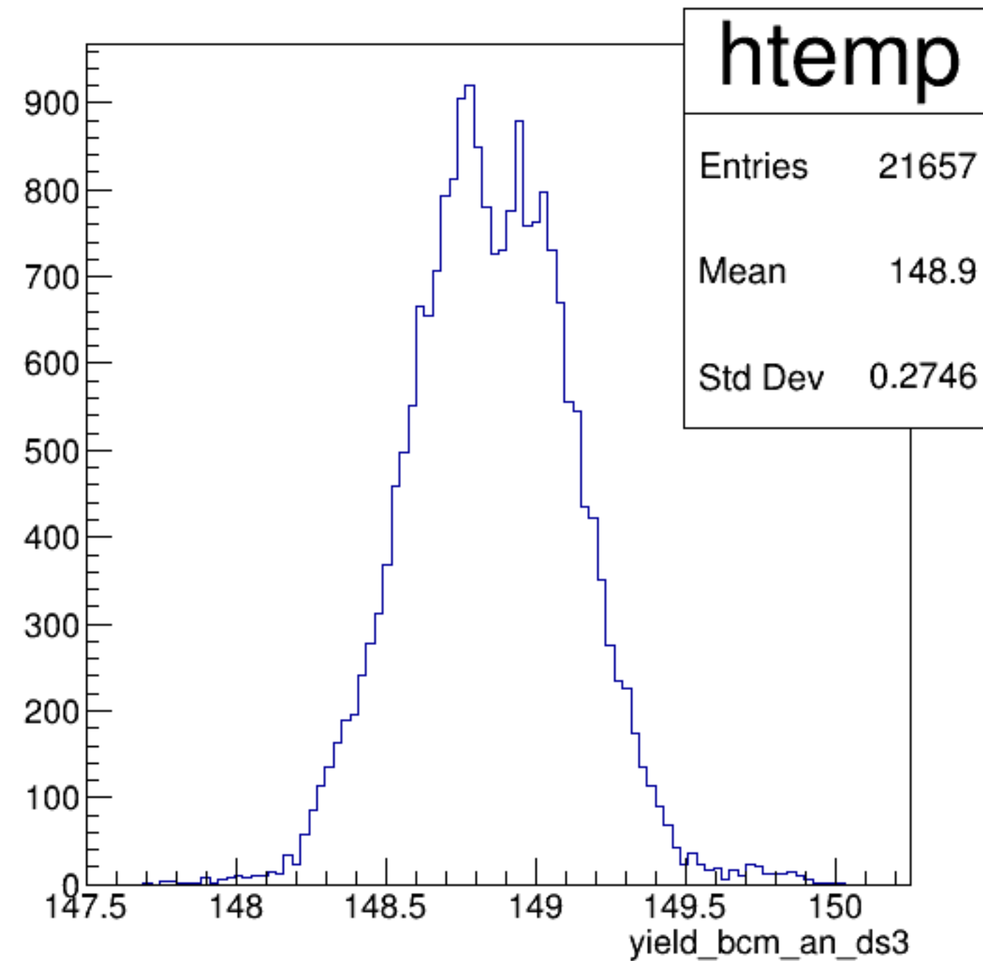
yield_bcm_an_ds3 {ErrorFlag==0}
