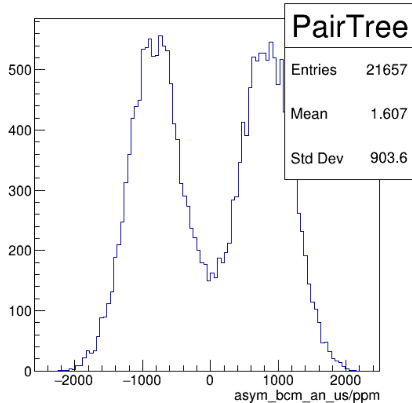
asym_bcm_an_us/ppm {ErrorFlag==0}
