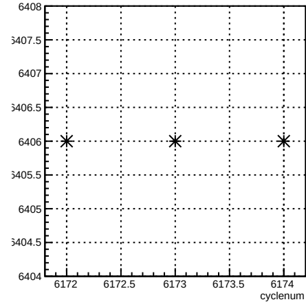
run:cyclenum {run == 6406}
