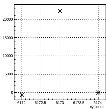
usr_coil7:cyclenum {run == 6406}
