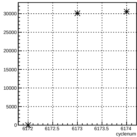
usl_coil6:cyclenum {run == 6406}
