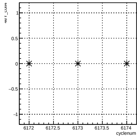
4eY_coil4:cyclenum {run == 6406}
