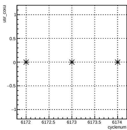
usr_coil3:cyclenum {run == 6406}
