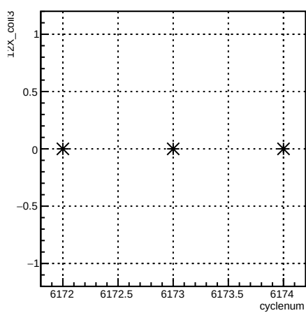
12X_coil3:cyclenum {run == 6406}
