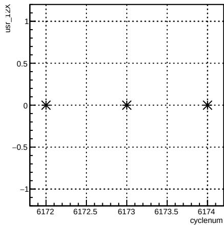
usr_12X:cyclenum {run == 6406}
