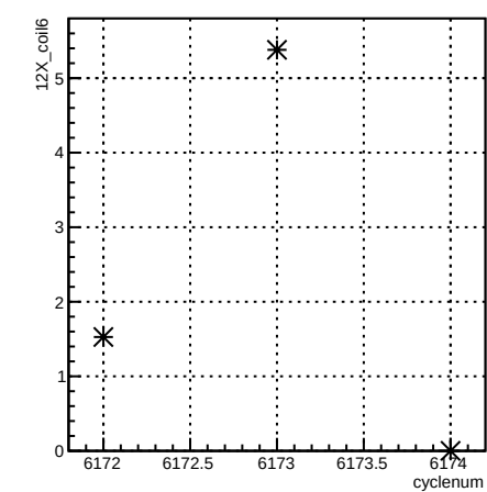
12X_coil6:cyclenum {run == 6406}
