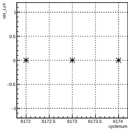
usl_12X:cyclenum {run == 6406}
