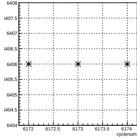
run:cyclenum {run == 6406}
