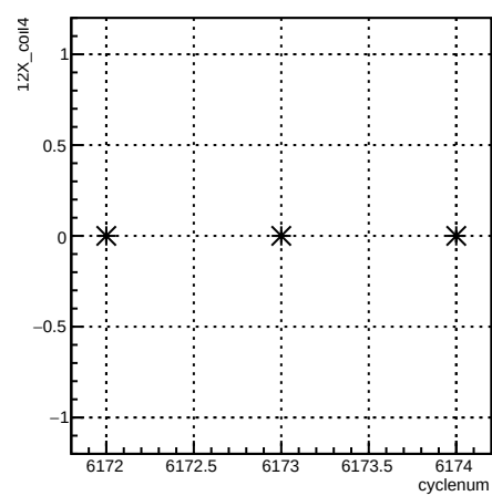
12X_coil4:cyclenum {run == 6406}
