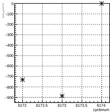
usl_coil6:cyclenum {run == 6406}
