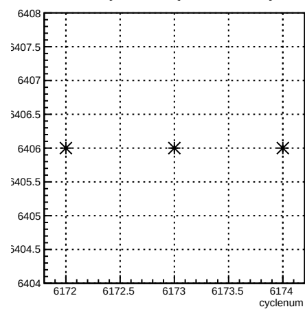
run:cyclenum {run == 6406}
