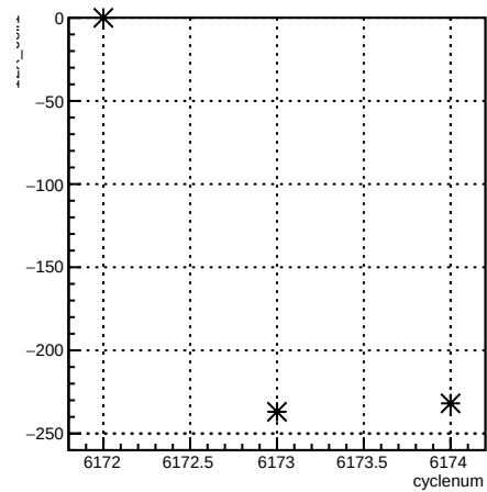
12X_coil1:cyclenum {run == 6406}
