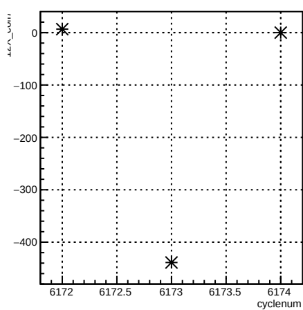
12X_coil7:cyclenum {run == 6406}
