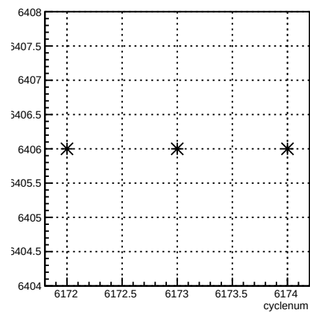
run:cyclenum {run == 6406}
