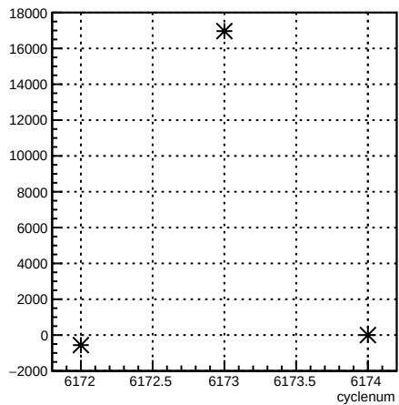
usl_coil7:cyclenum {run == 6406}
