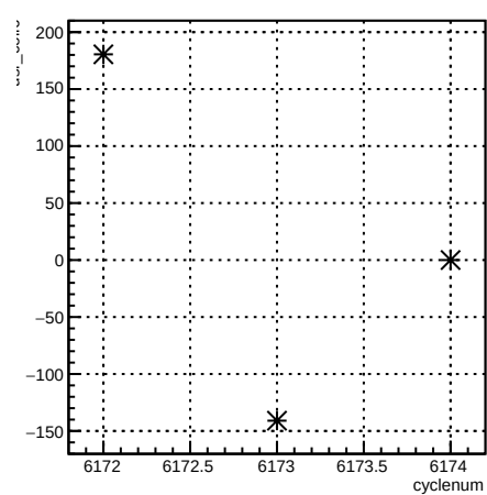
usr_coil6:cyclenum {run == 6406}
