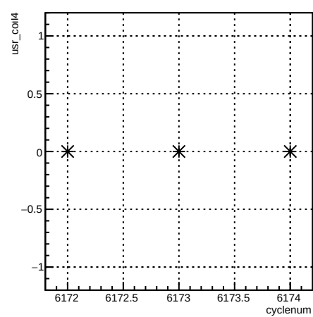
usr_coil4:cyclenum {run == 6406}
