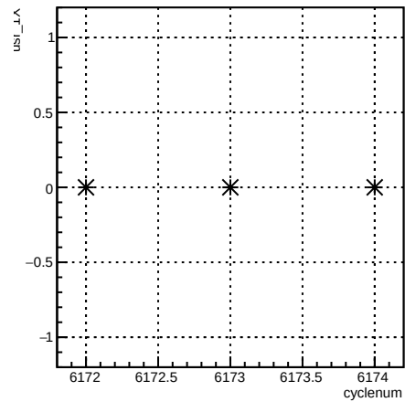
usr_4eY:cyclenum {run == 6406}
