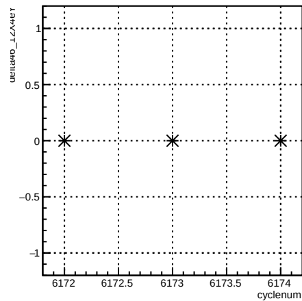
delta46_12X4eY:cyclenum {run == 6406}
