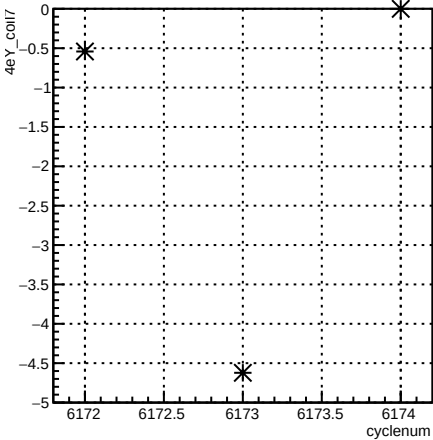
4eY_coil7:cyclenum {run == 6406}
