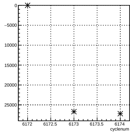
usr_coil1:cyclenum {run == 6406}
