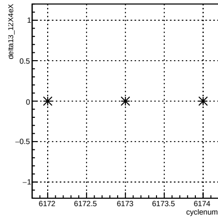
segment:cyclenum {run == 6406}
