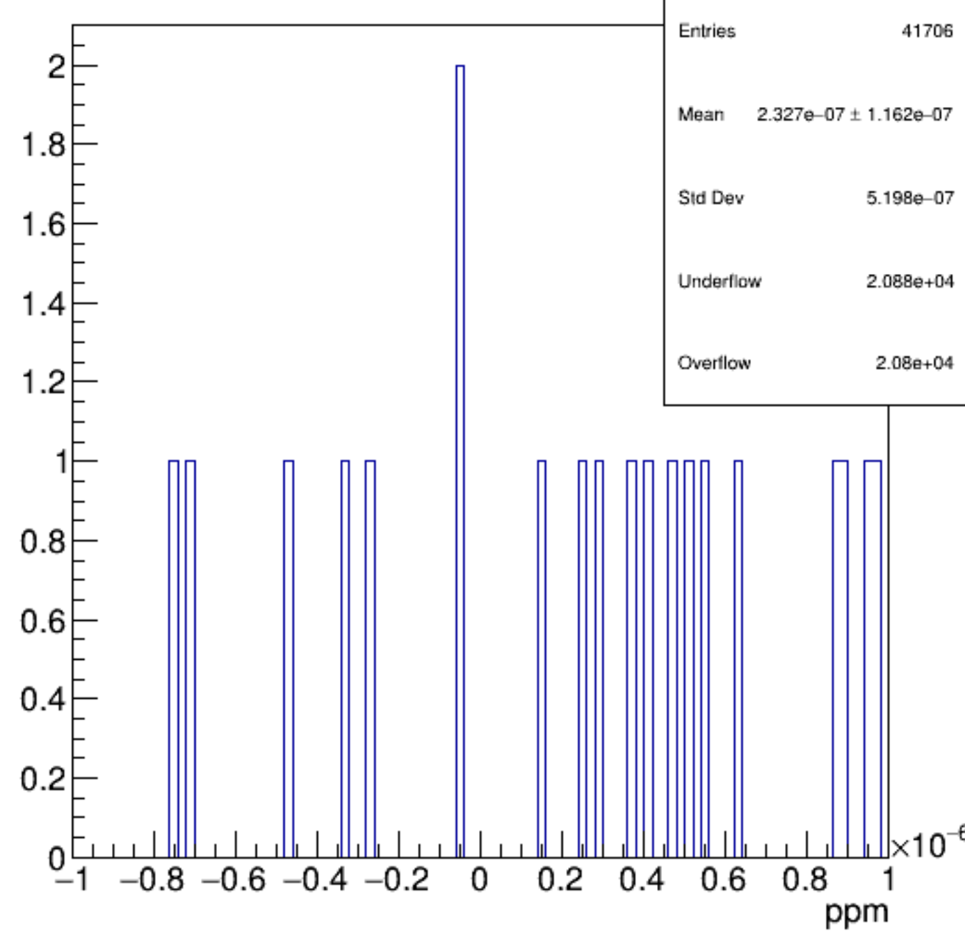
asym_bcm_an_diff
