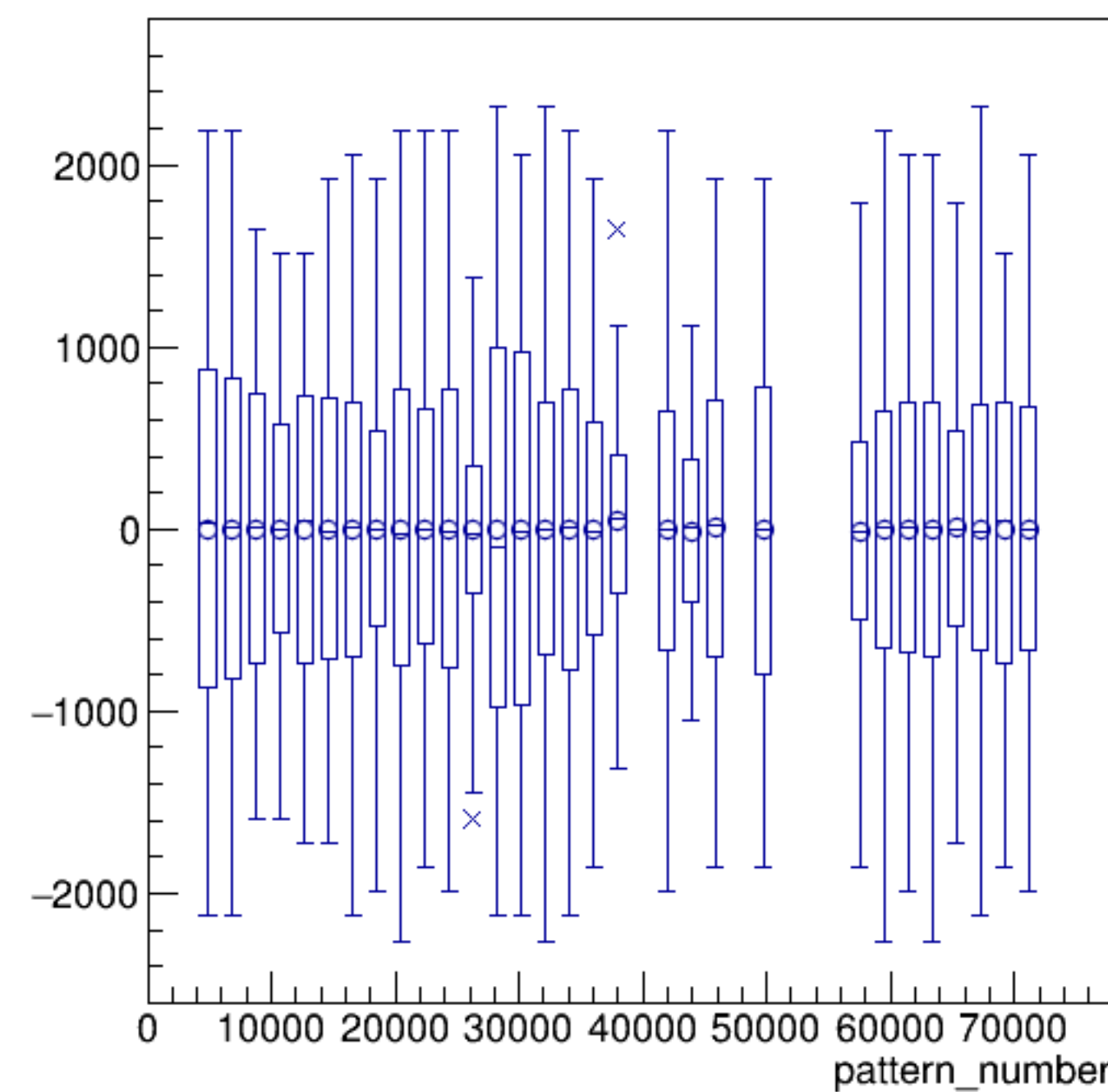
asym_bcm_an_ds3/ppm:pattern_number {ErrorFlag==0}
