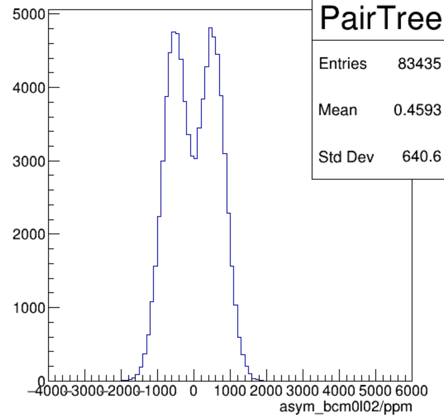
asym_bcm0l02/ppm {ErrorFlag==0}
