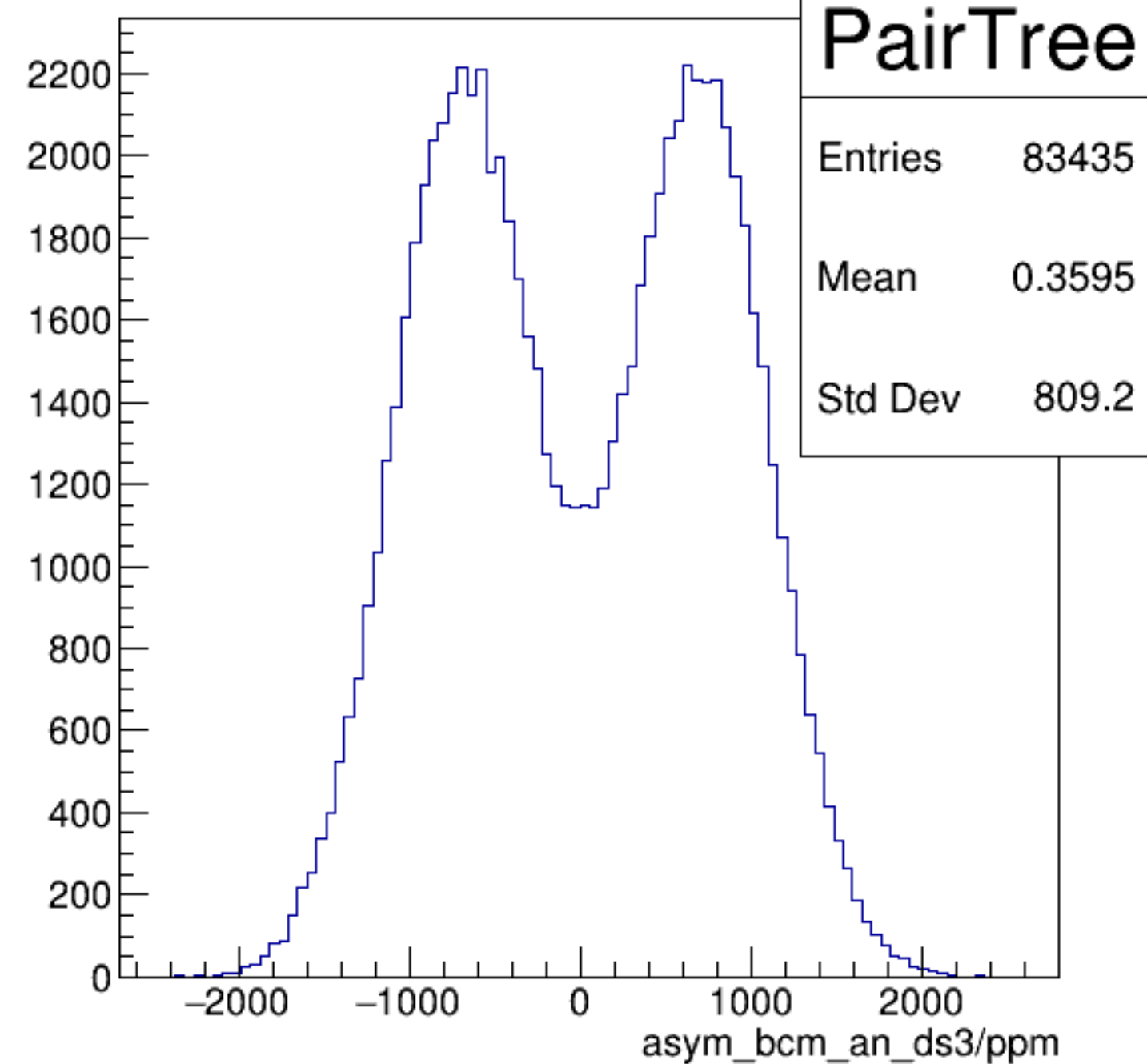
asym_bcm_an_ds3/ppm {ErrorFlag==0}
