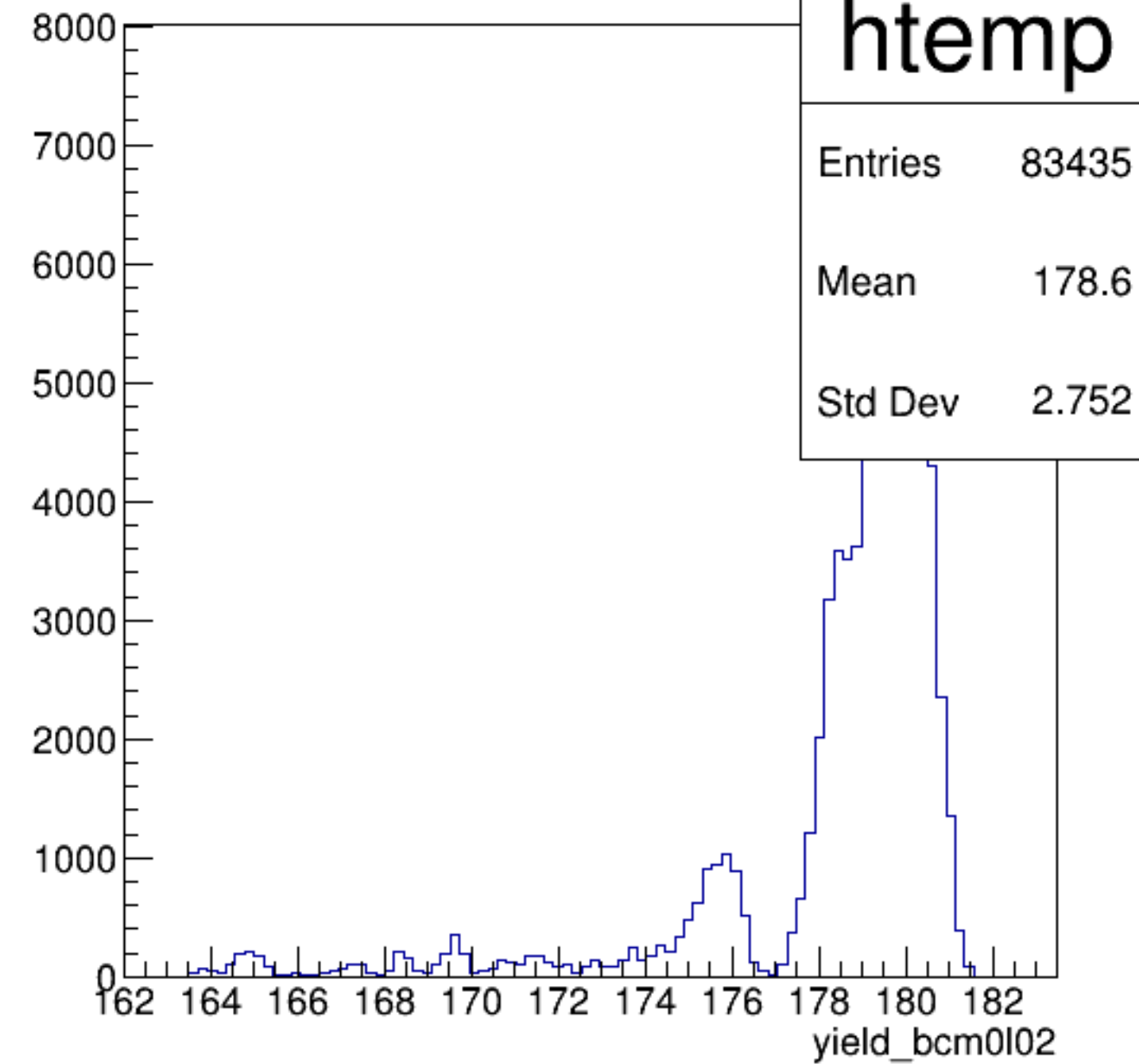
yield_bcm0l02 {ErrorFlag==0}
