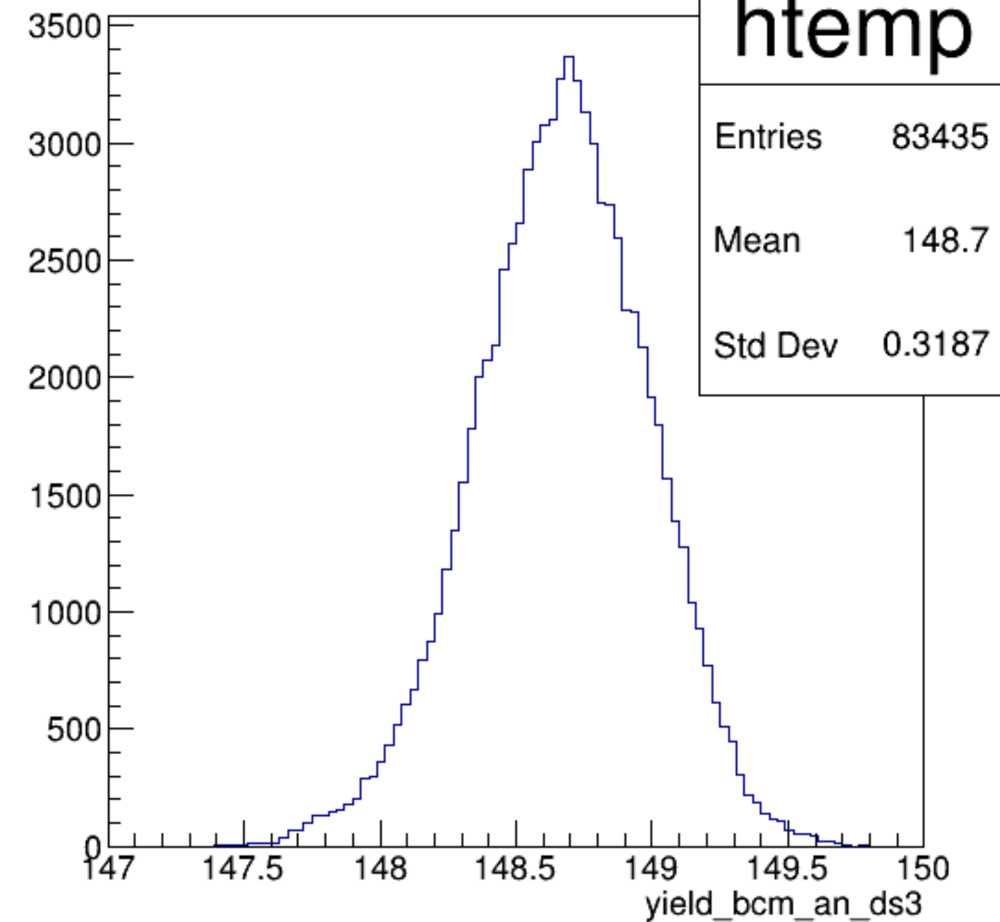
yield_bcm_an_ds3 {ErrorFlag==0}
