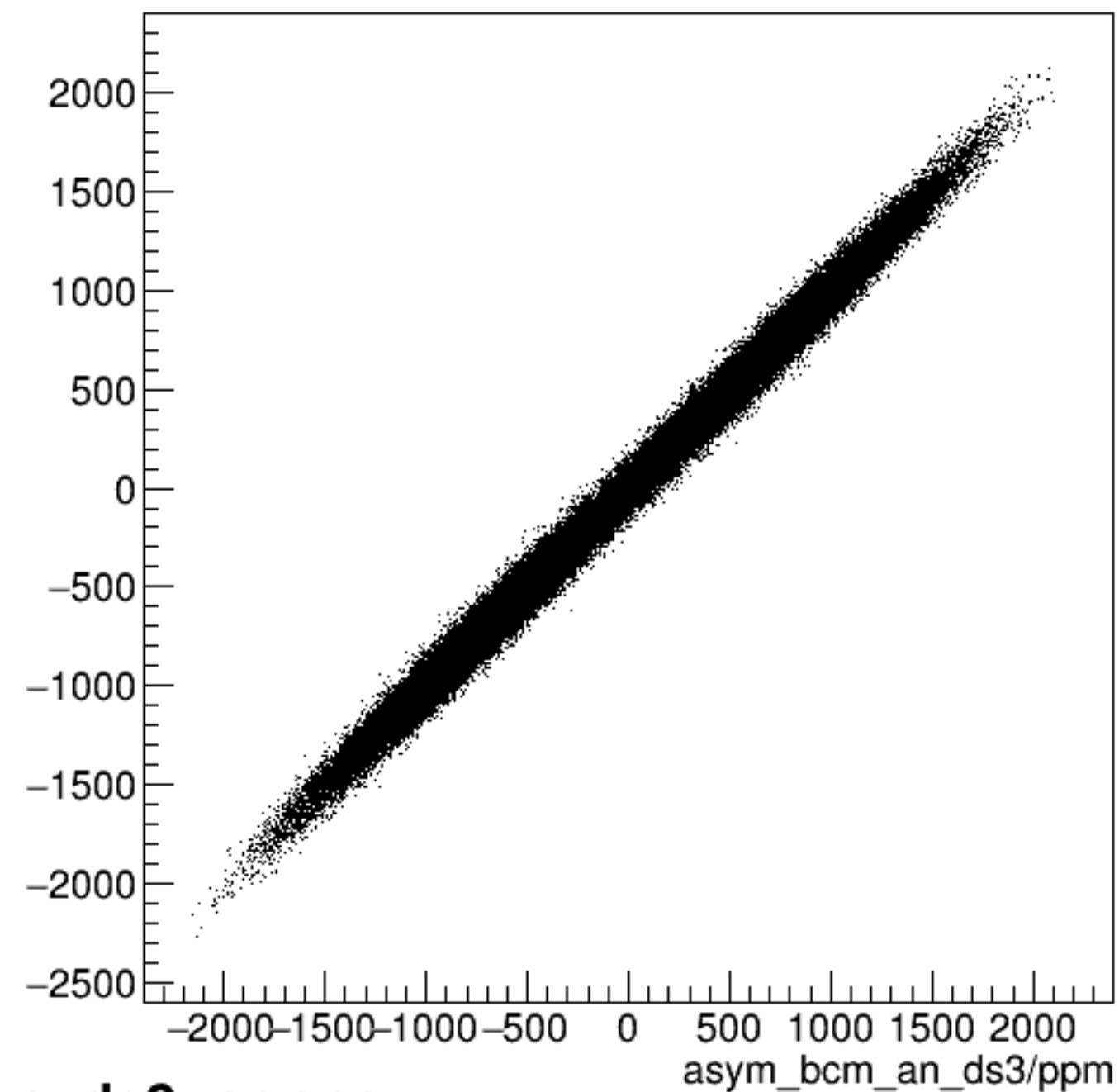
run6407_000_asym_bcm_dg_us_vs_asym_bcm_an_ds3_pr.png
