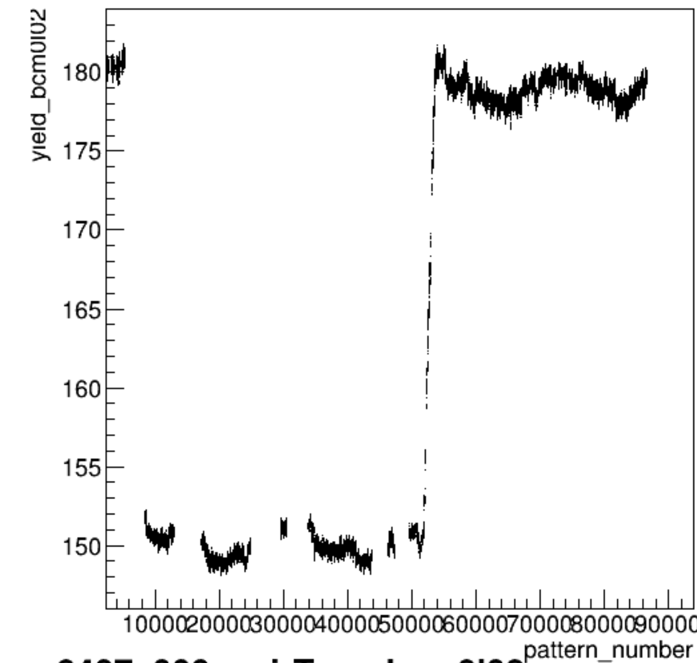
yield_bcm0l02:pattern_number {ErrorFlag==0}
