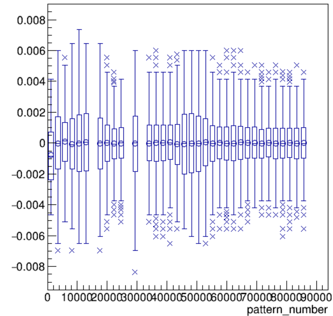
asym_bcm_an_diff*yield_bcm_an_diff:pattern_number {ErrorFlag==0}
