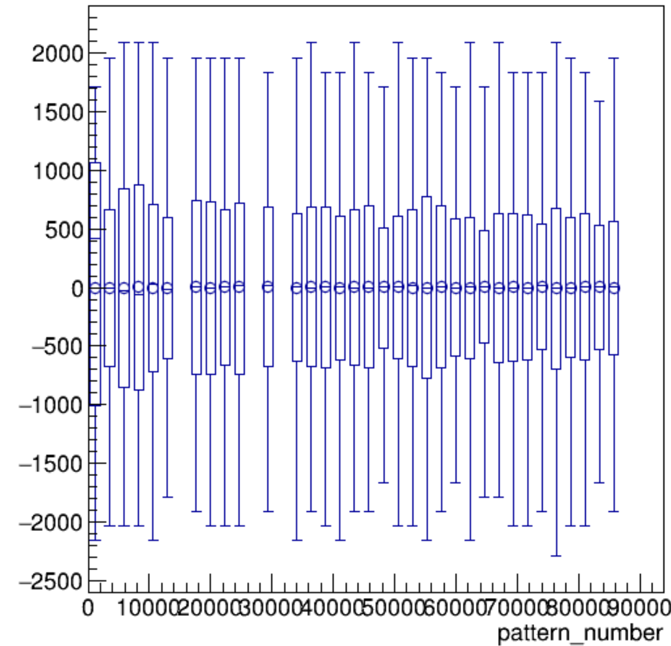
asym_bcm_dg_us/ppm:pattern_number {ErrorFlag==0}
