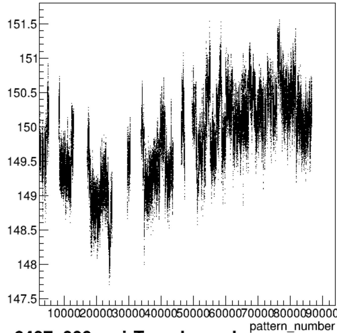
yield_bcm_dg_us:pattern_number {ErrorFlag==0}
