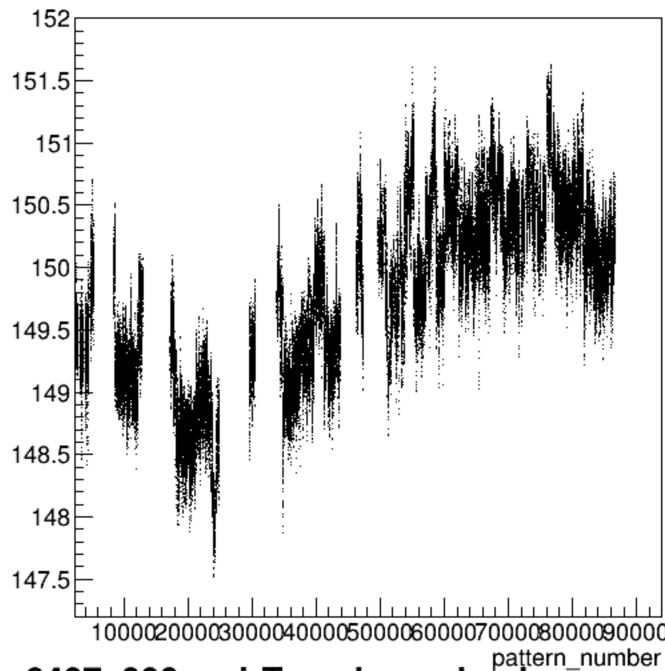
yield_bcm_dg_ds:pattern_number {ErrorFlag==0}
