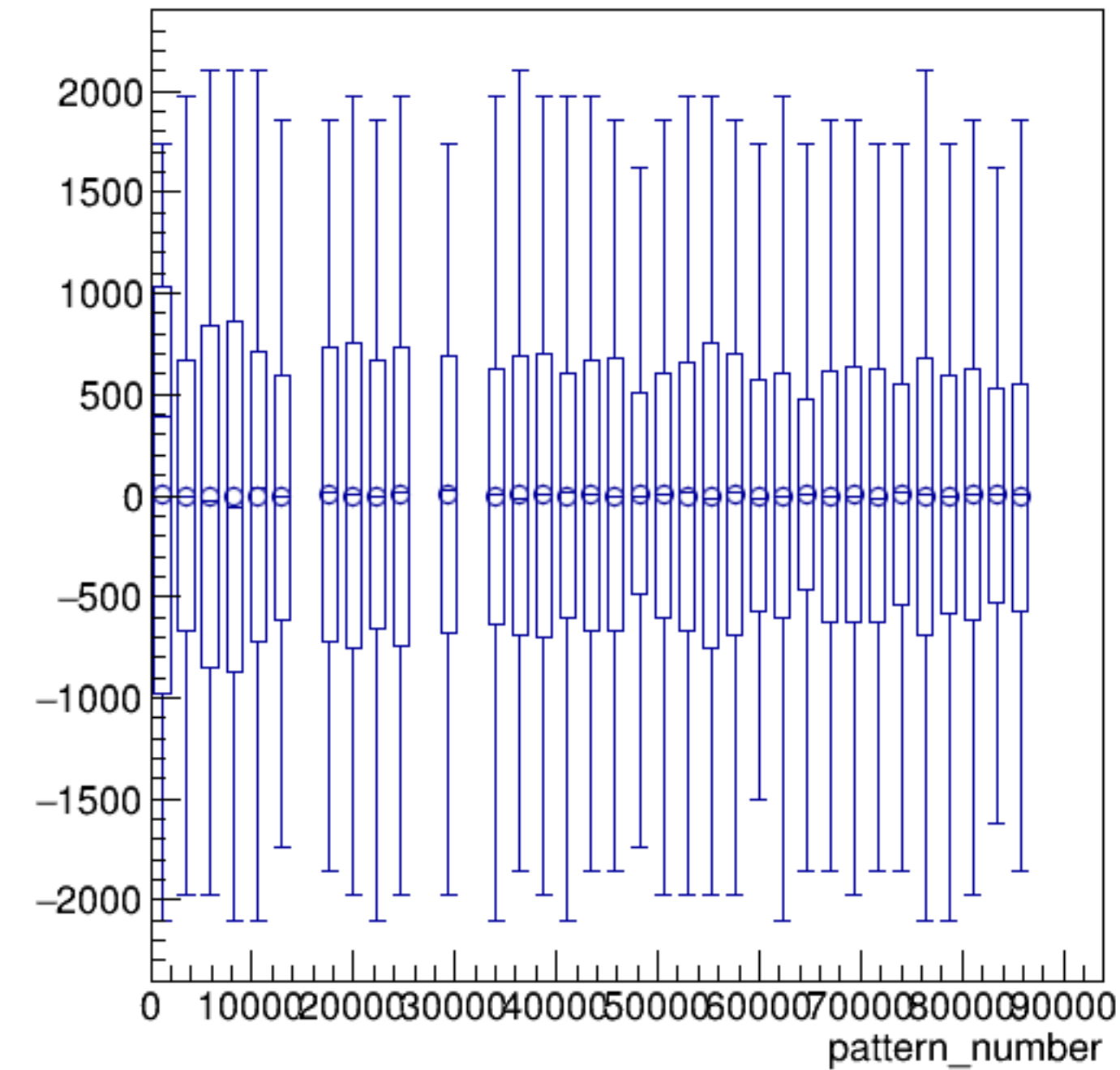
asym_bcm_an_ds/ppm:pattern_number {ErrorFlag==0}
