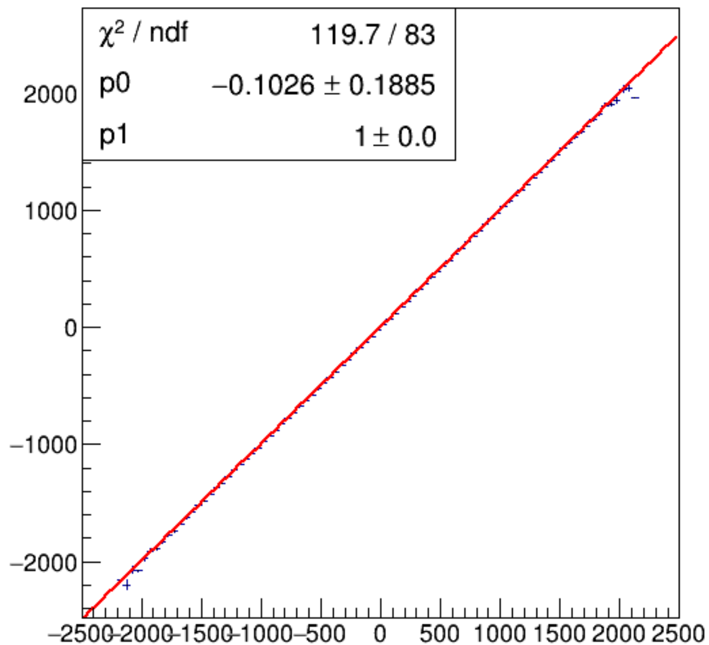
run6407_000_asym_bcm_dg_us_vs_asym_bcm_an_ds3_pr.png
