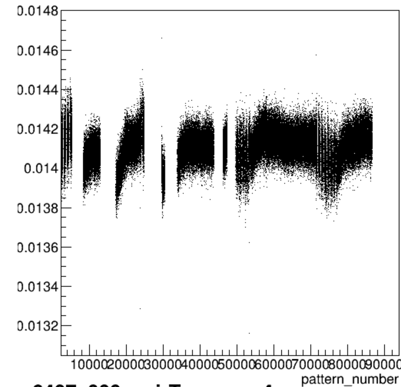
yield_sam4:pattern_number {ErrorFlag==0}
