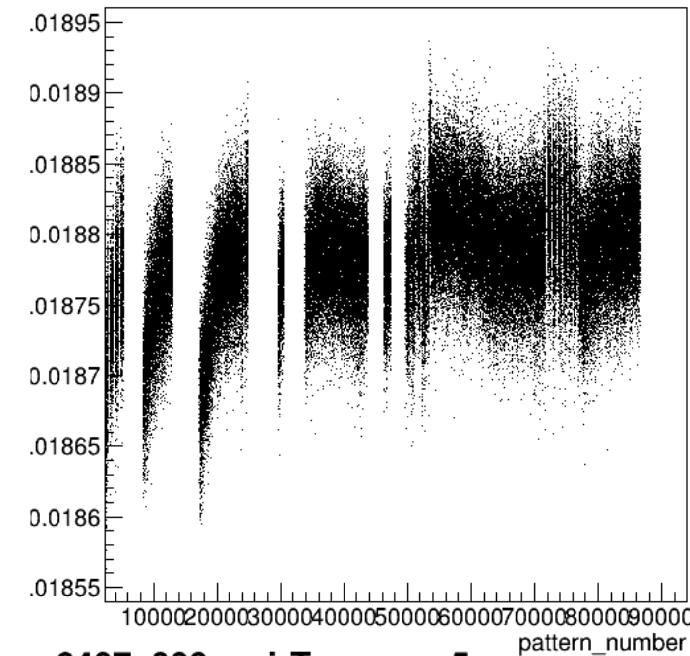
yield_sam5:pattern_number {ErrorFlag==0}
