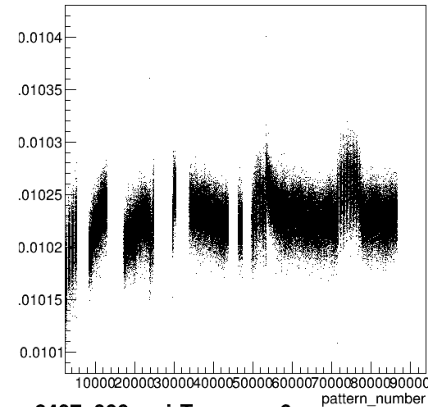
yield_sam6:pattern_number {ErrorFlag==0}
