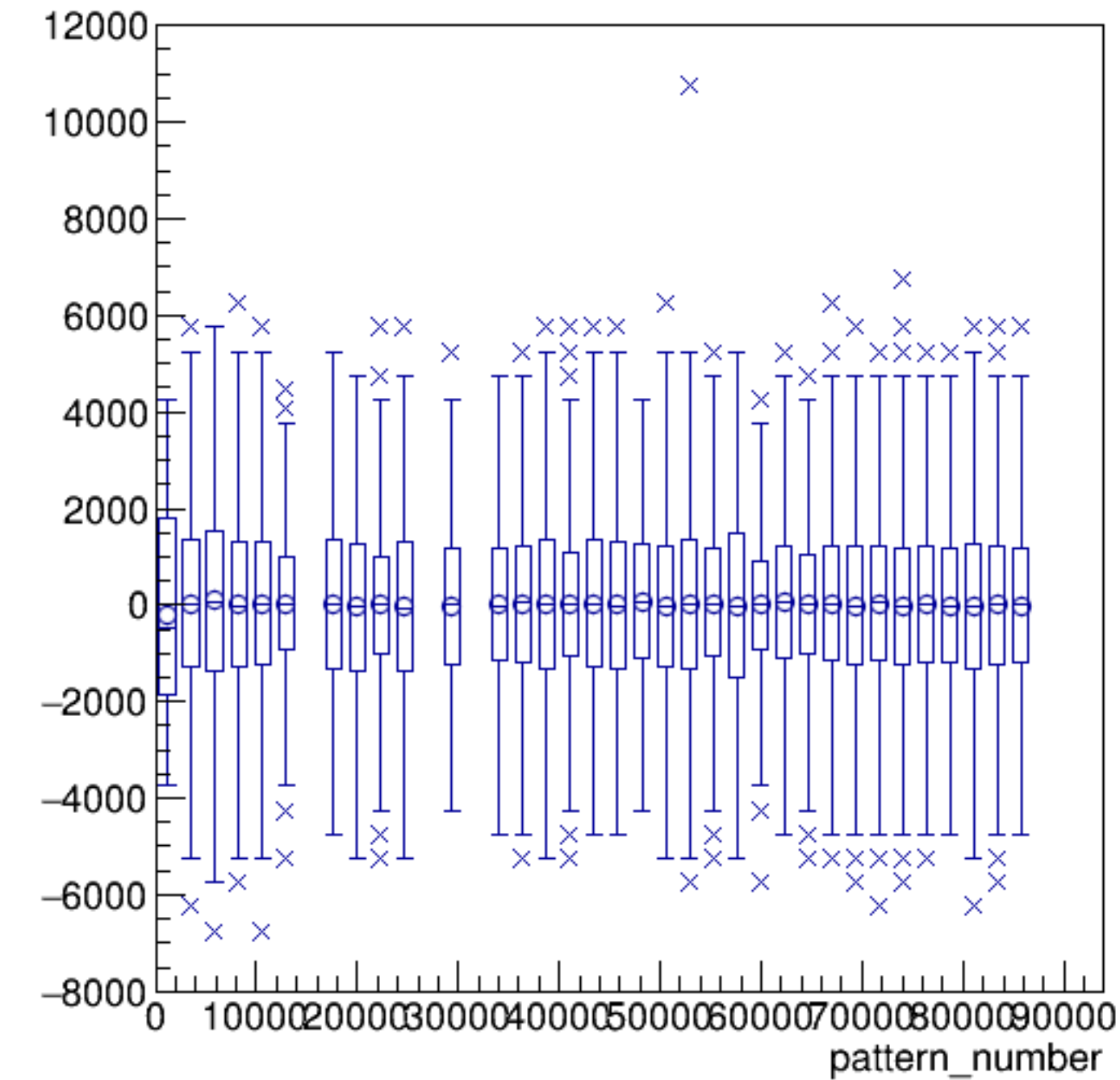
asym_sam6/ppm:pattern_number {ErrorFlag==0}
