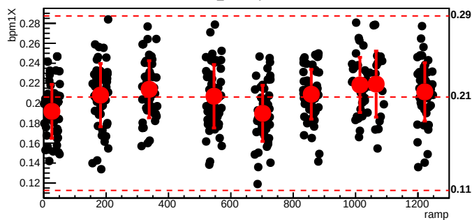
bmod_trim4,cyc=6178
