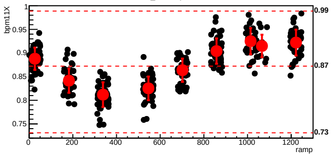
bmod_trim3,cyc=6178
