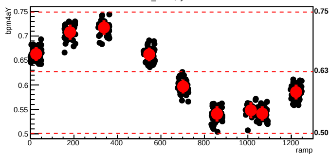
bmod_trim6,cyc=6178
