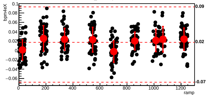
bmod_trim4,cyc=6178
