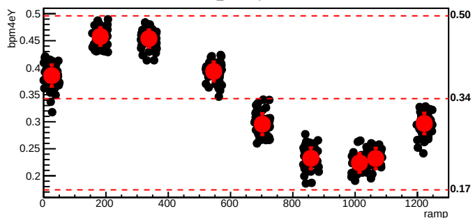
bmod_trim4,cyc=6178
