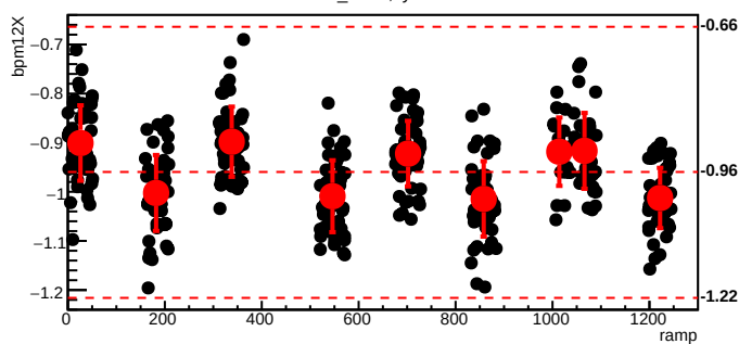
bmod_trim6,cyc=6178
