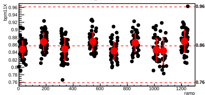
bmod_trim4,cyc=6178
