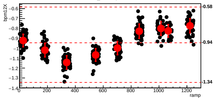
bmod_trim3,cyc=6178
