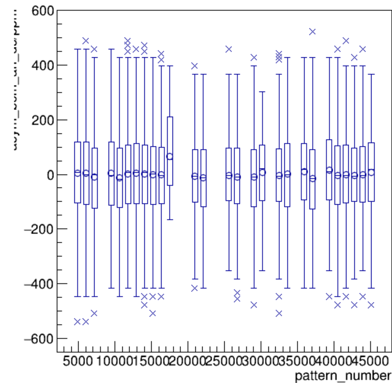
asym_bcm_an_ds/ppm:pattern_number {ErrorFlag==0}
