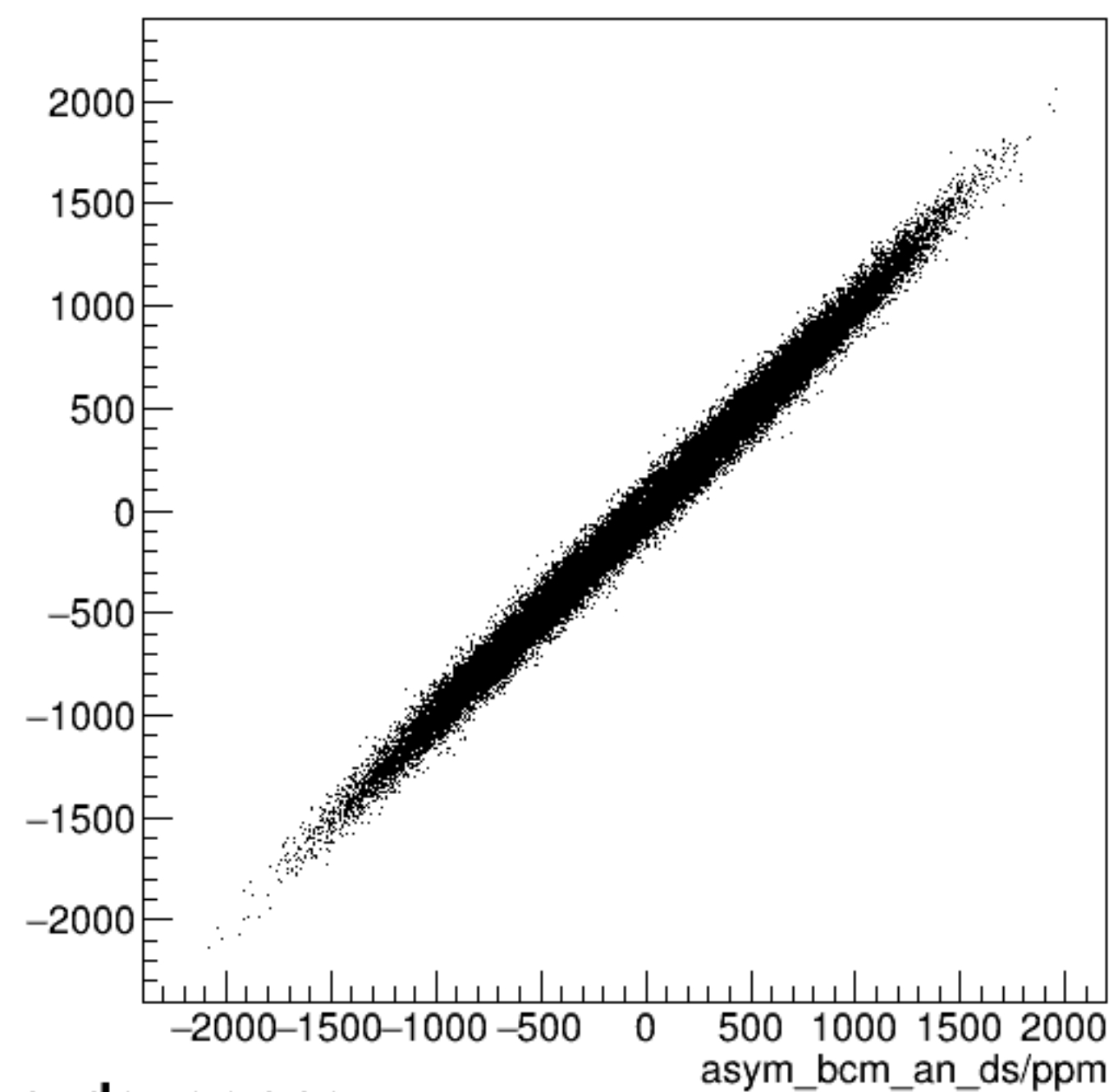
run6408_000_asym_bcm_dg_us_vs_asym_bcm_an_ds_pr.png
