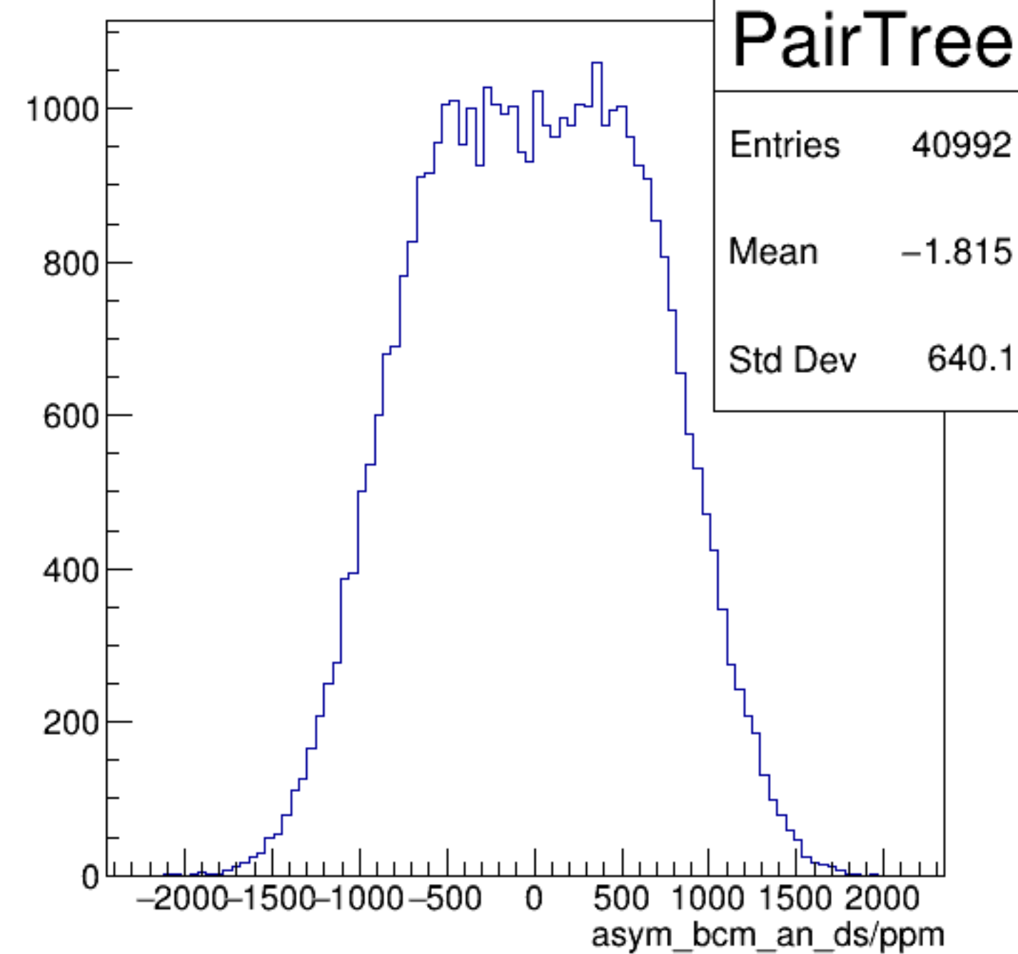
asym_bcm_an_ds/ppm {ErrorFlag==0}
