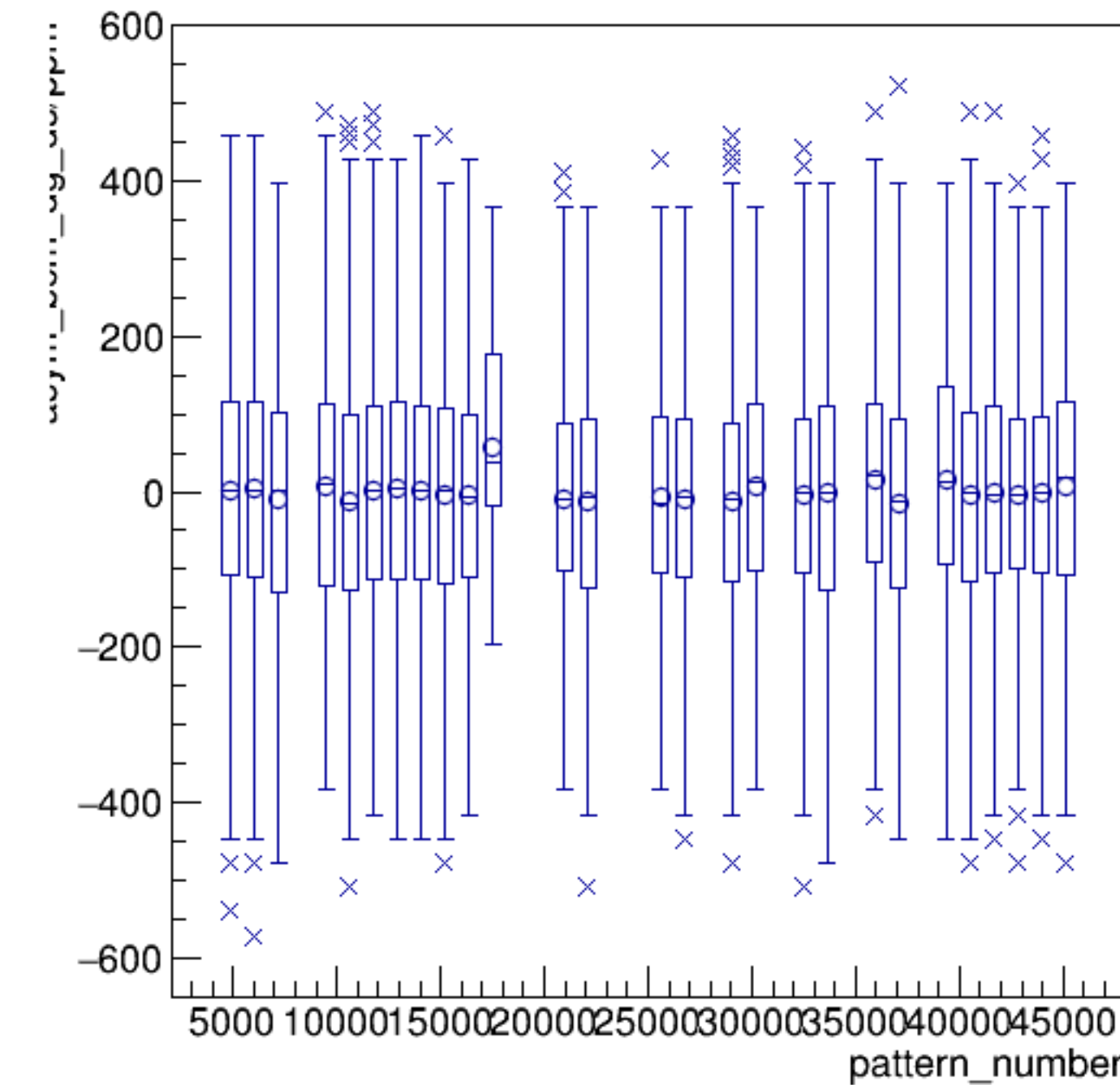
asym_bcm_dg_ds/ppm:pattern_number {ErrorFlag==0}
