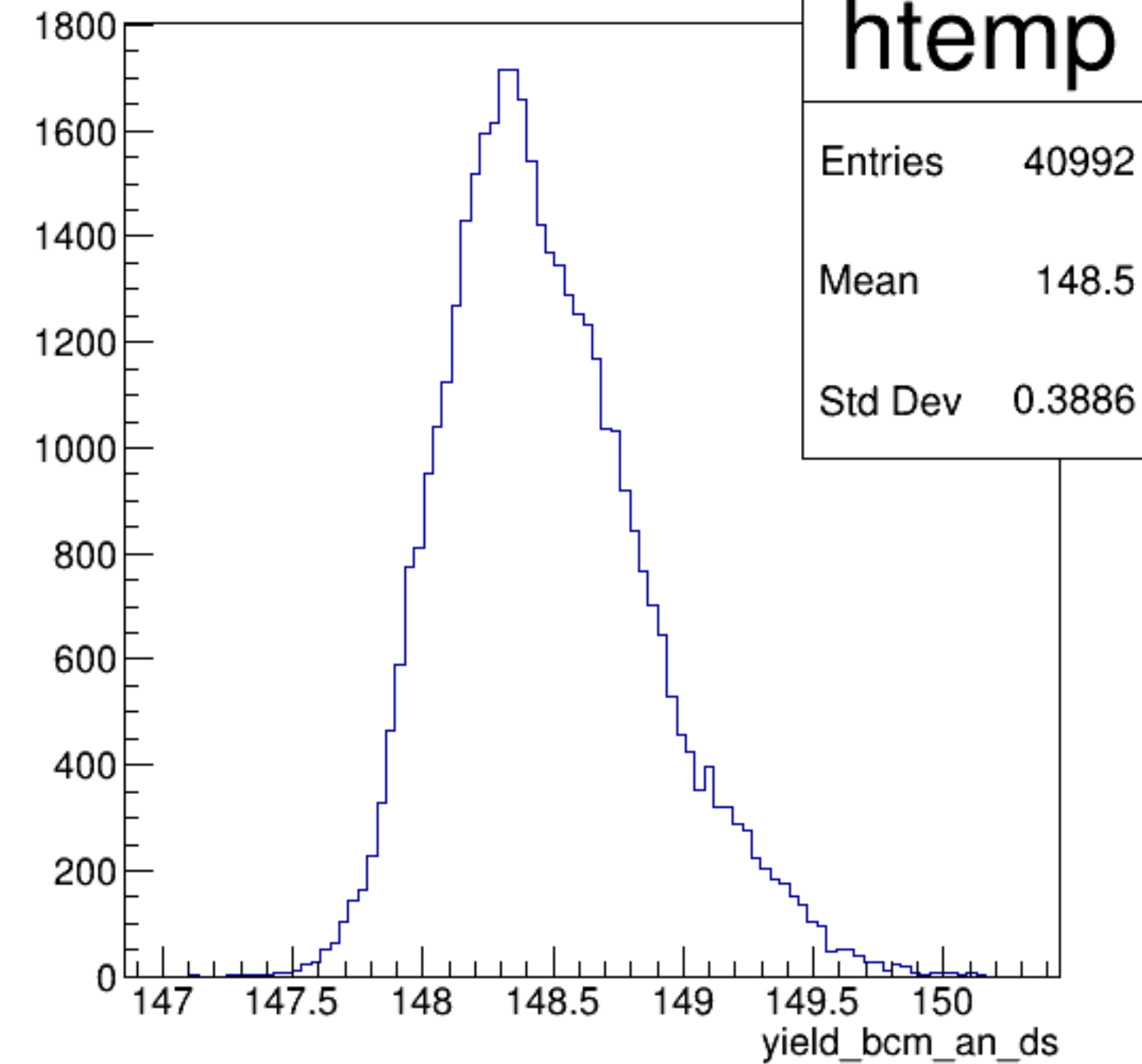
yield_bcm_an_ds {ErrorFlag==0}
