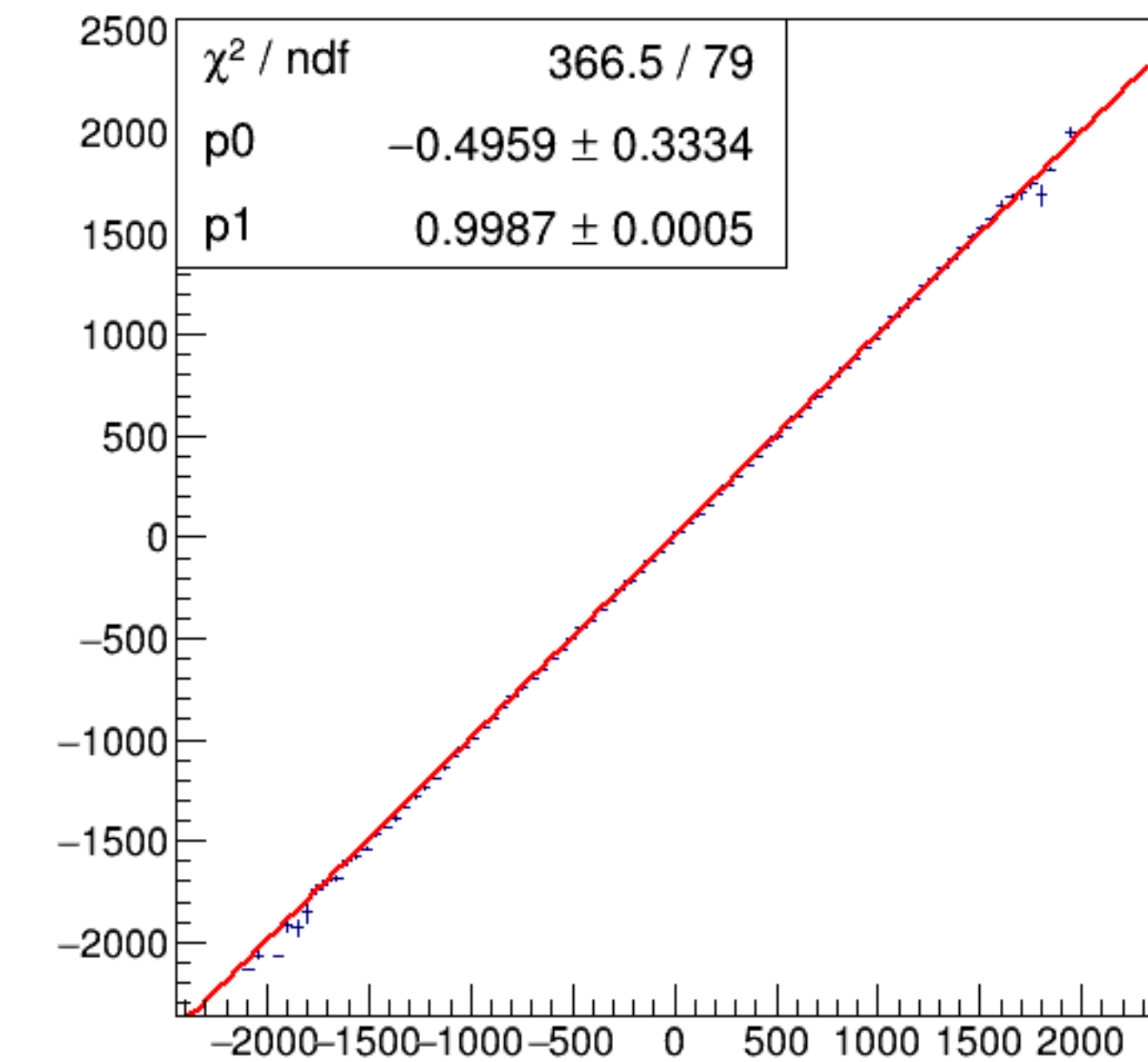
run6408_000_asym_bcm_dg_us_vs_asym_bcm_an_ds_pr.png
