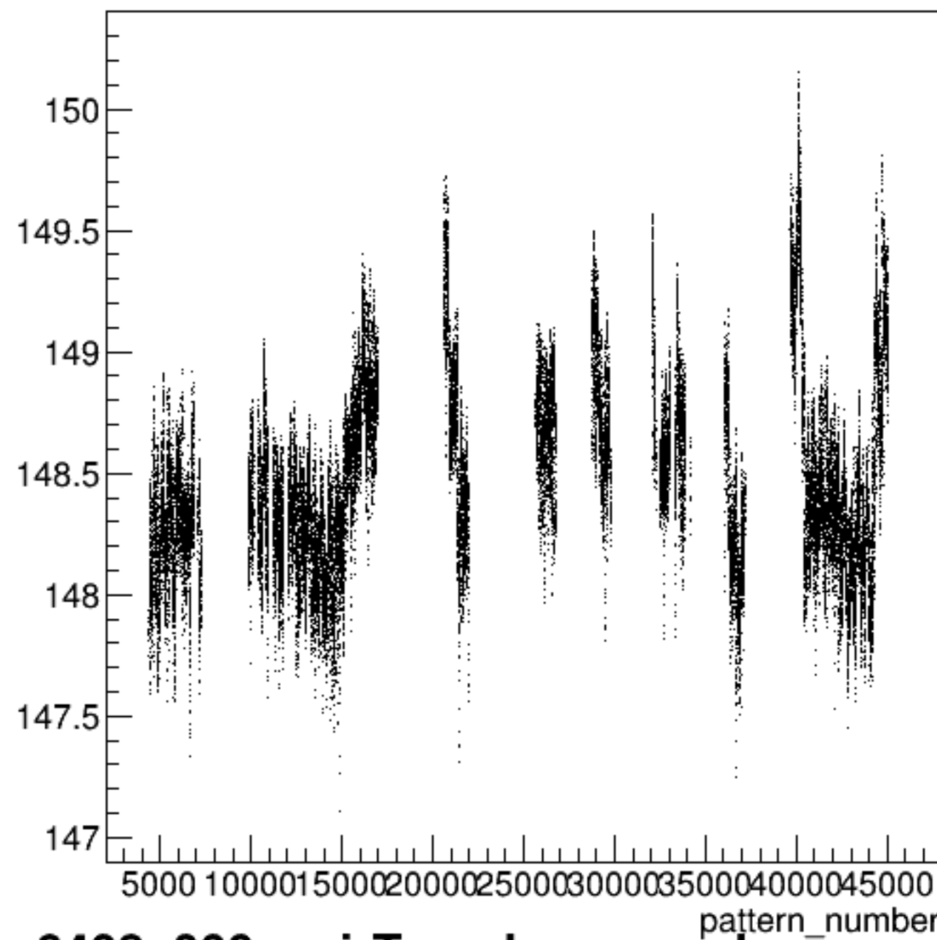
yield_bcm_an_ds:pattern_number {ErrorFlag==0}
