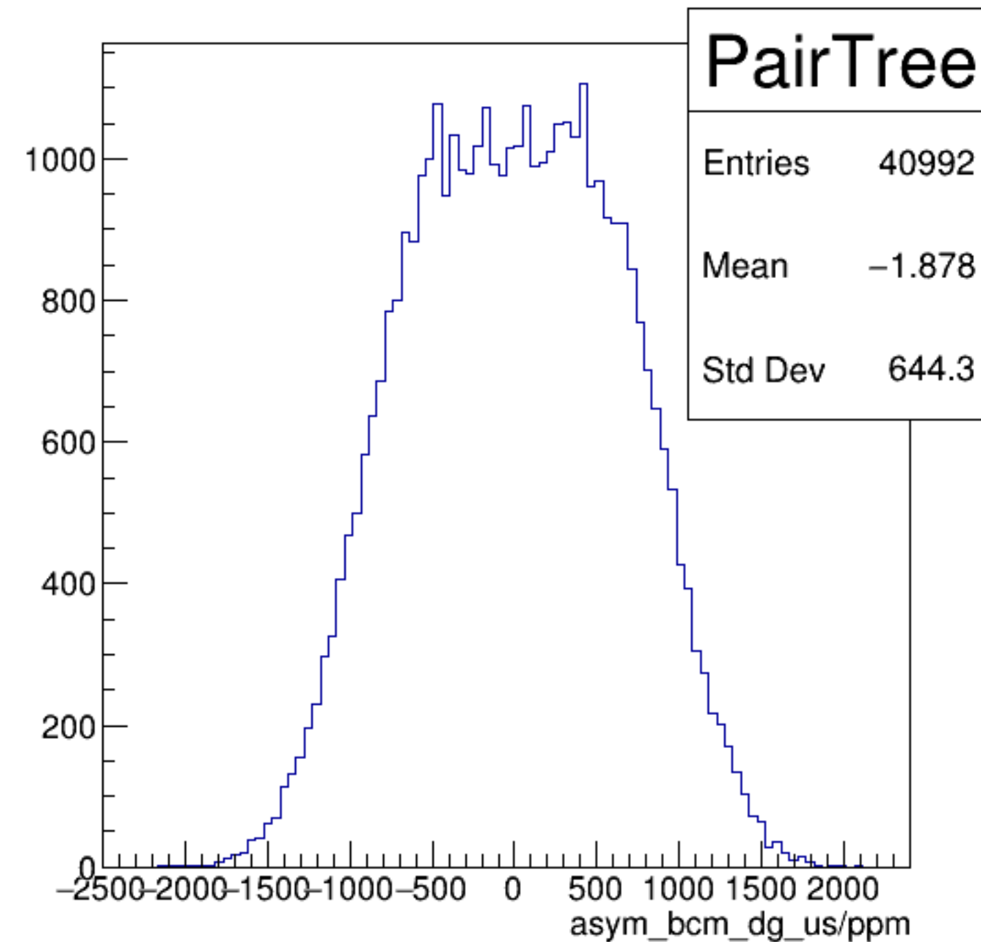
asym_bcm_dg_us/ppm {ErrorFlag==0}
