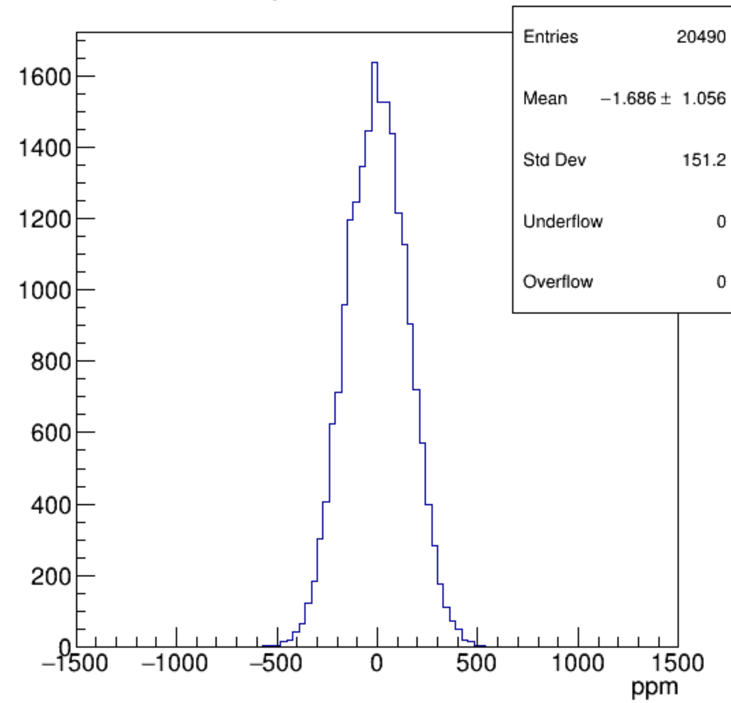
asym_bcm_an_us
