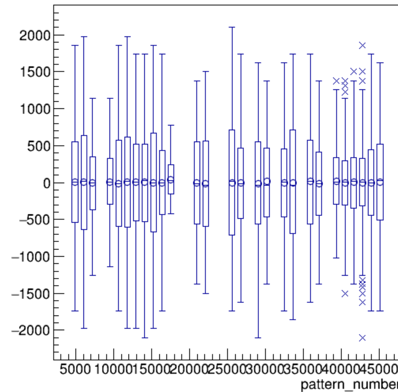
asym_bcm_dg_us/ppm:pattern_number {ErrorFlag==0}
