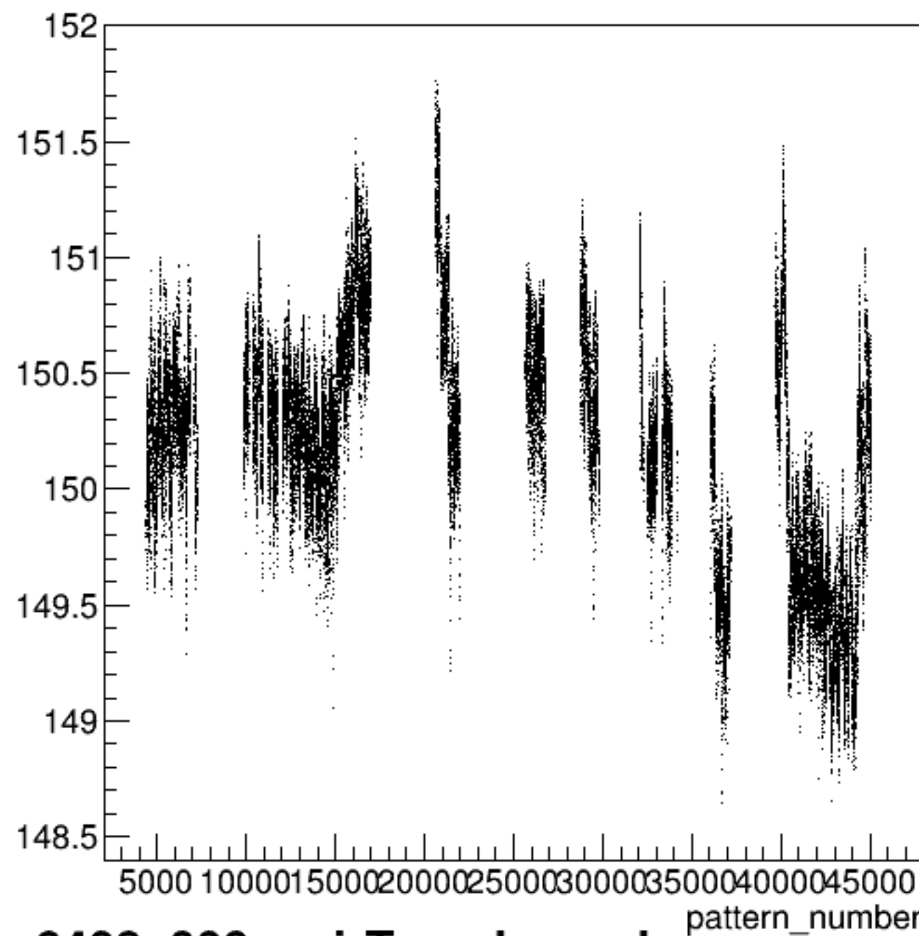
yield_bcm_dg_us:pattern_number {ErrorFlag==0}
