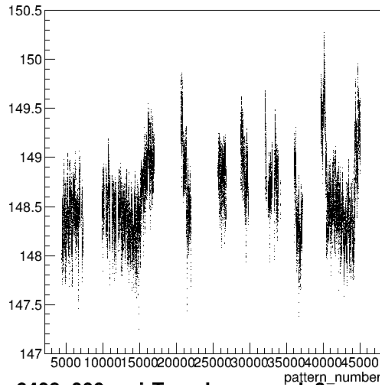
yield_bcm_an_ds3:pattern_number {ErrorFlag==0}
