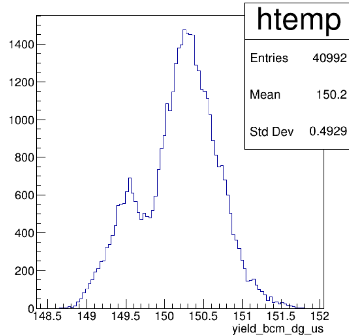
yield_bcm_dg_us {ErrorFlag==0}
