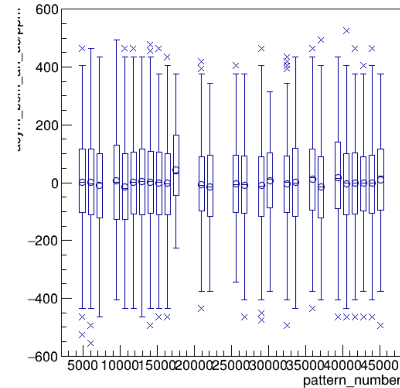
asym_bcm_an_us/ppm:pattern_number {ErrorFlag==0}
