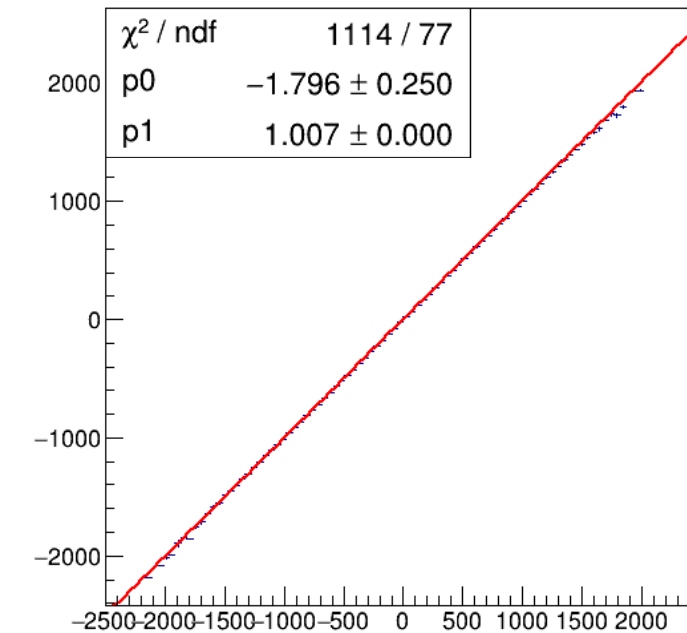
run6408_000_asym_bcm_dg_ds_vs_asym_bcm_an_us_pr.png
