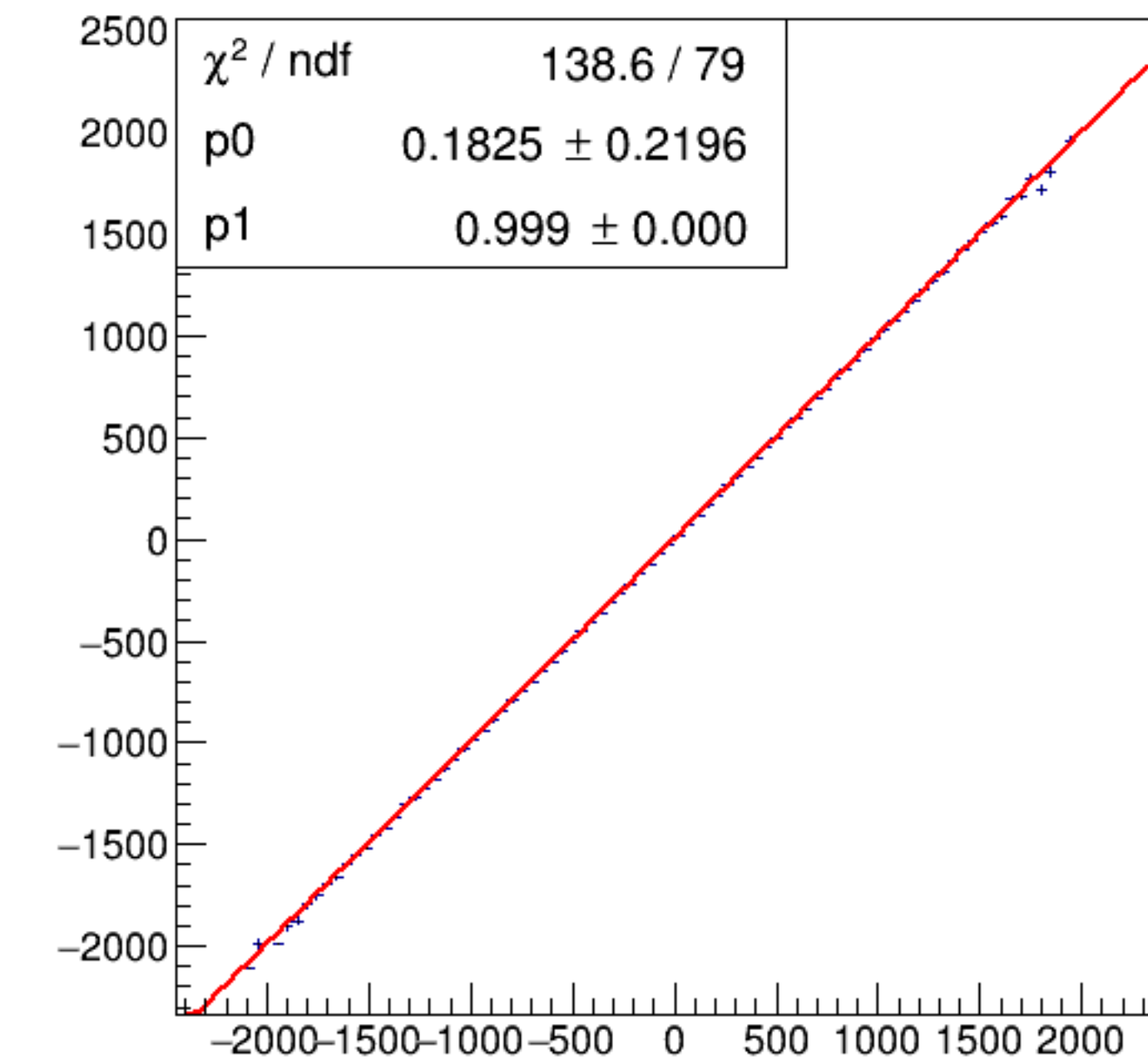
run6408_000_asym_bcm_an_us_vs_asym_bcm_an_ds_pr.png
