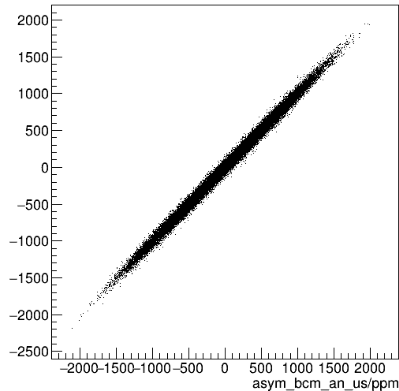
run6408_000_asym_bcm_dg_ds_vs_asym_bcm_an_us_pr.png
