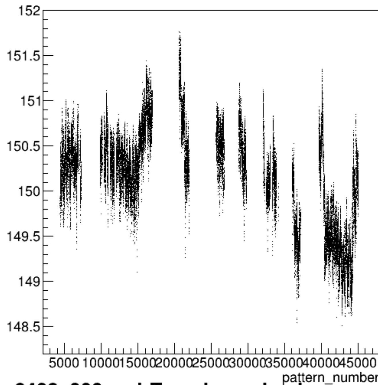
yield_bcm_dg_ds:pattern_number {ErrorFlag==0}
