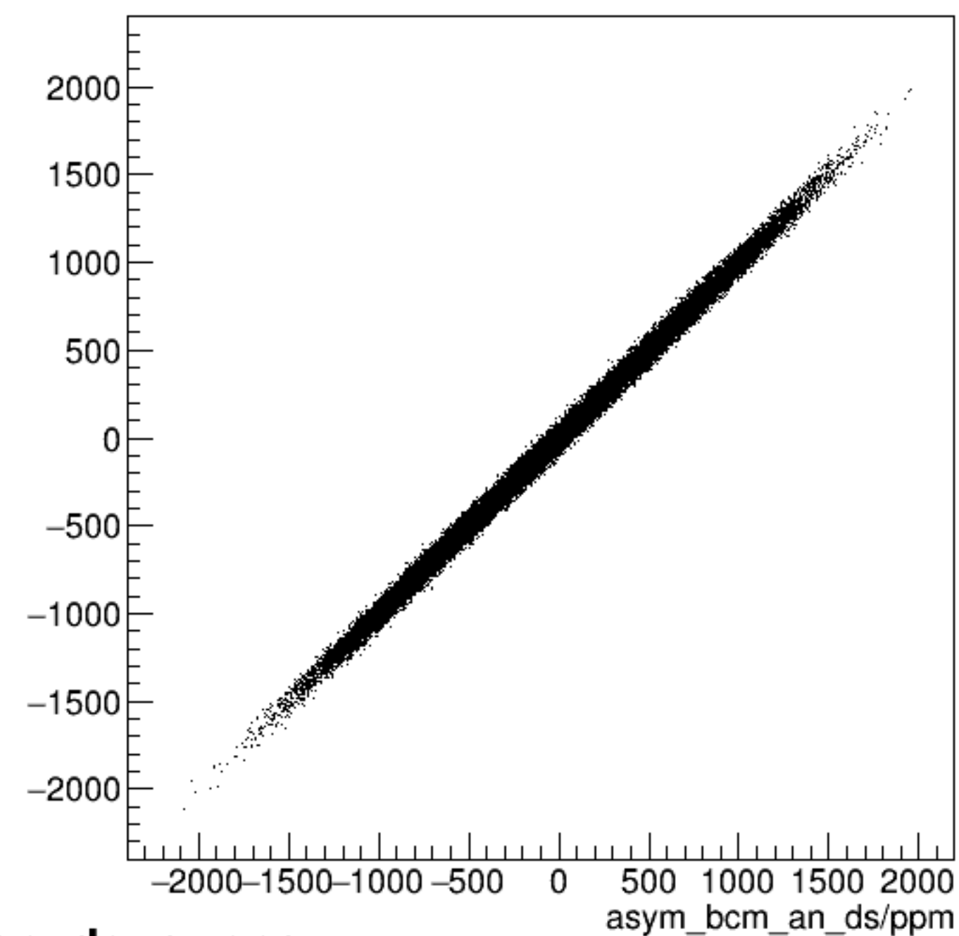
run6408_000_asym_bcm_an_us_vs_asym_bcm_an_ds_pr.png
