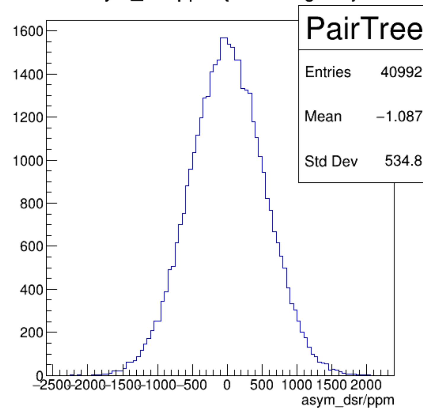
asym_dsr/ppm {ErrorFlag==0}
