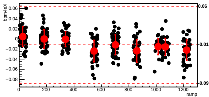
bmod_trim6,cyc=6179
