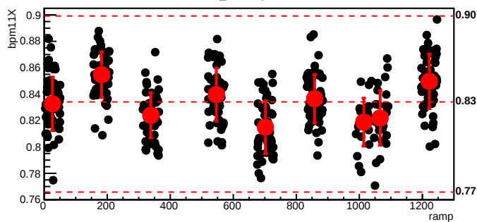
bmod_trim6,cyc=6179
