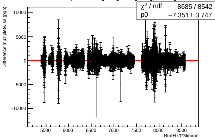
Difference multipletwise of eigen lagr vs. eigen reg, self weighted
