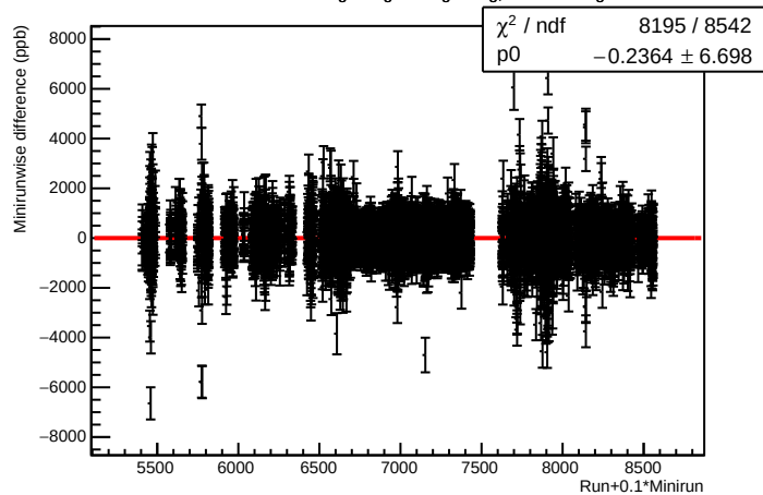
Minirunwise difference of eigen lagr vs. eigen reg, maindet weighted
