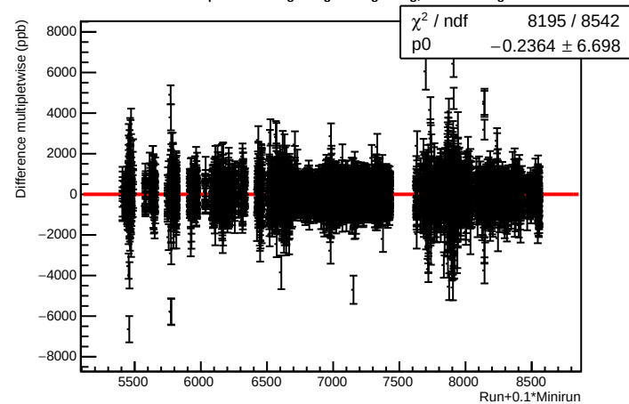
Difference multipletwise of eigen lagr vs. eigen reg, maindet weighted
