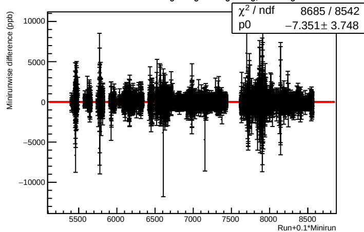
Minirunwise difference of eigen lagr vs. eigen reg, self weighted
