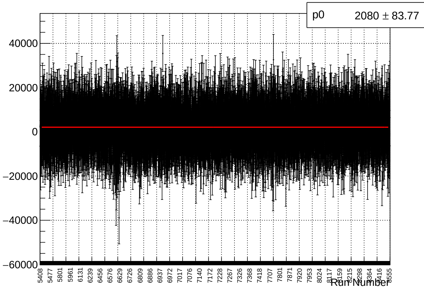
Signed eigen_lagr_asym_main_det_mean (ppb) vs Time
