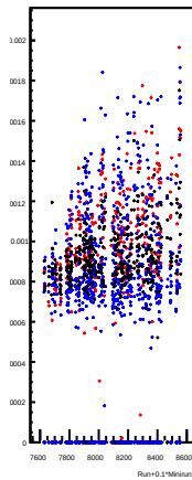
Col 5, eigen_reg_asyim_us_avg RMS
