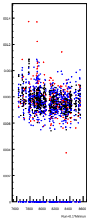
Col 4, eigen_reg_asyim_us_avg RMS
