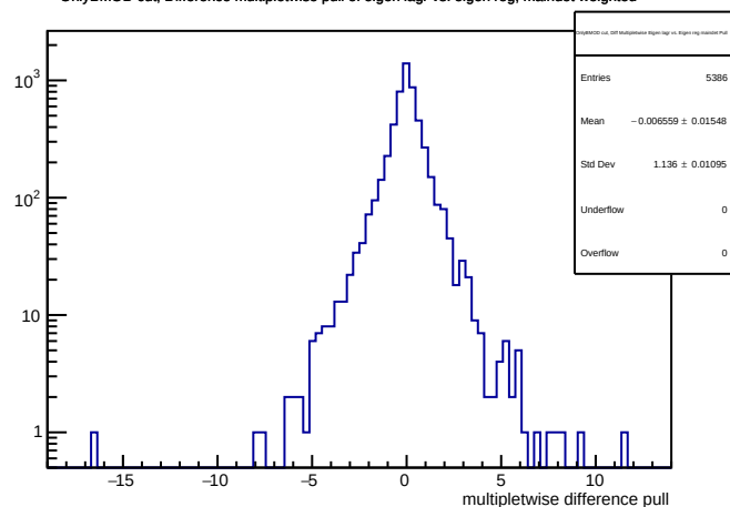
OnlyBMOD cut, Difference multipletwise pull of eigen lagr vs. eigen reg, maindet weighted
