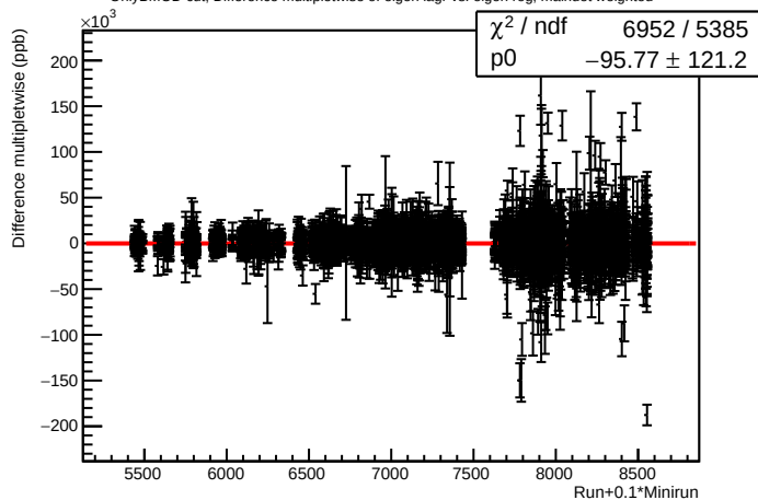
OnlyBMOD cut, Difference multipletwise of eigen lagr vs. eigen reg, maindet weighted
