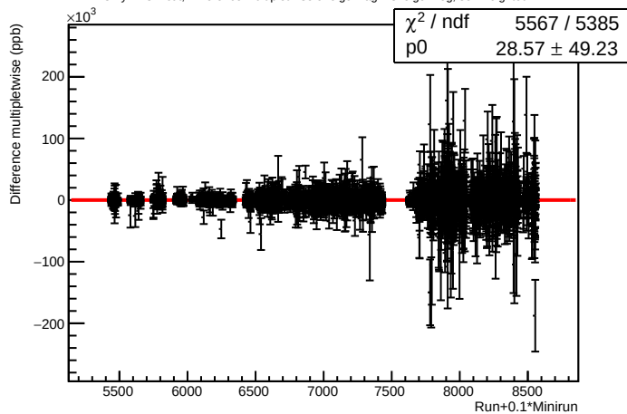
OnlyBMOD cut, Difference multipletwise of eigen lagr vs. eigen reg, self weighted
