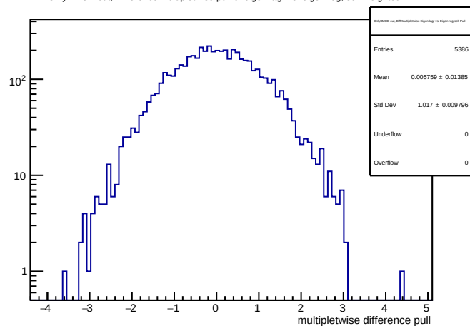
OnlyBMOD cut, Difference multipletwise pull of eigen lagr vs. eigen reg, self weighted
