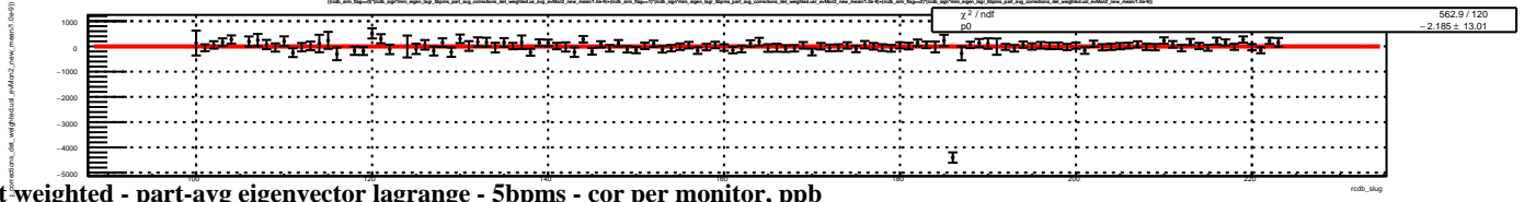
main det-weighted - part-avg eigenvector lagrange - 5bpms - cor per monitor, ppb
