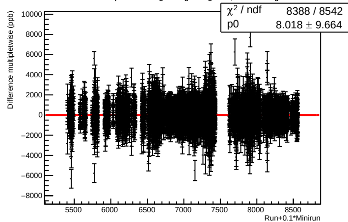
Difference multipletwise of regular reg vs. eigen dit, maindet weighted
