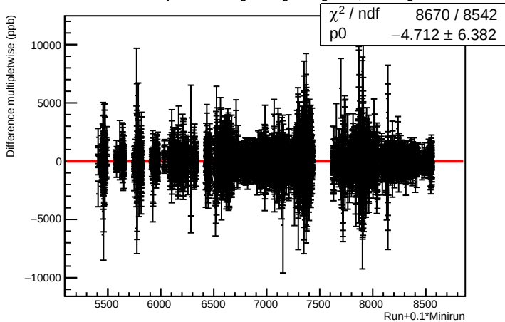
Difference multipletwise of regular reg vs. eigen dit, self weighted
