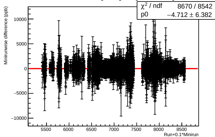
Minirunwise difference of regular reg vs. eigen dit, self weighted
