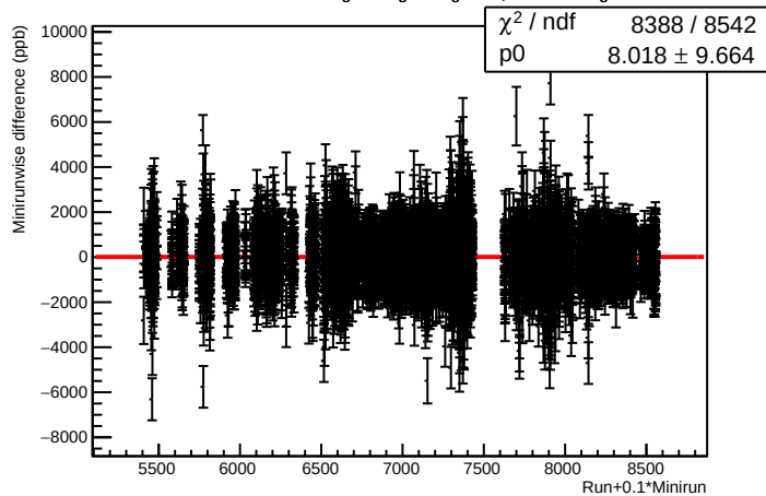
Minirunwise difference of regular reg vs. eigen dit, maindet weighted
