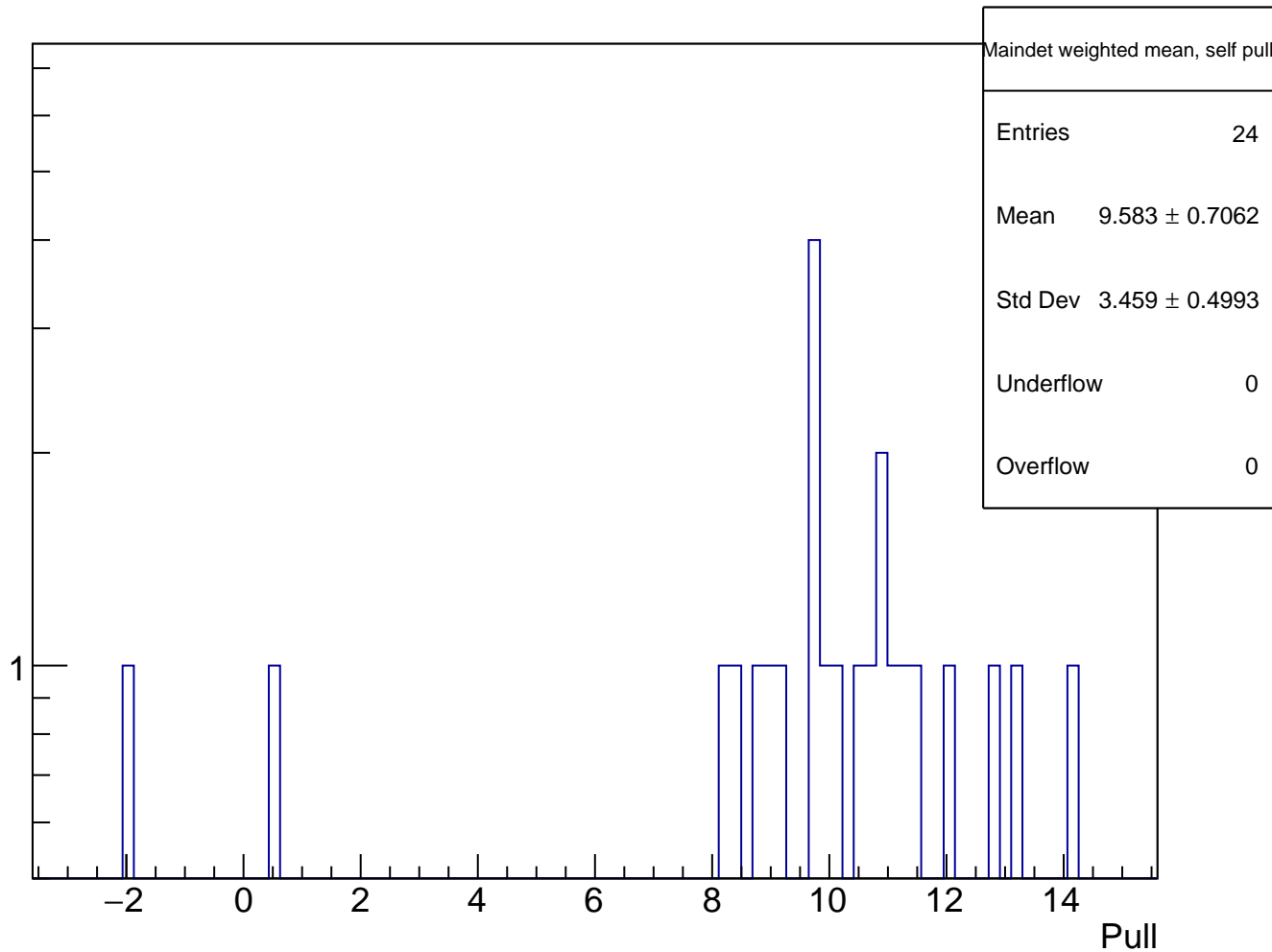
Maindet weighted mean, self pull - asym bcm_cav4cQ_bcm_an_ds_agg_dd
