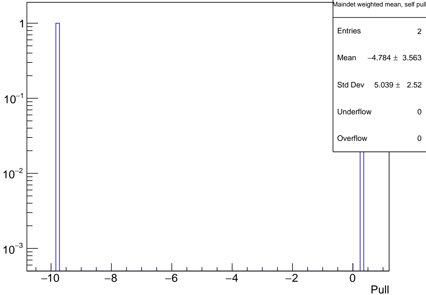
Maindet weighted mean, self pull - asym bcm_cav4cQ_bcm_an_us_agg_dd
