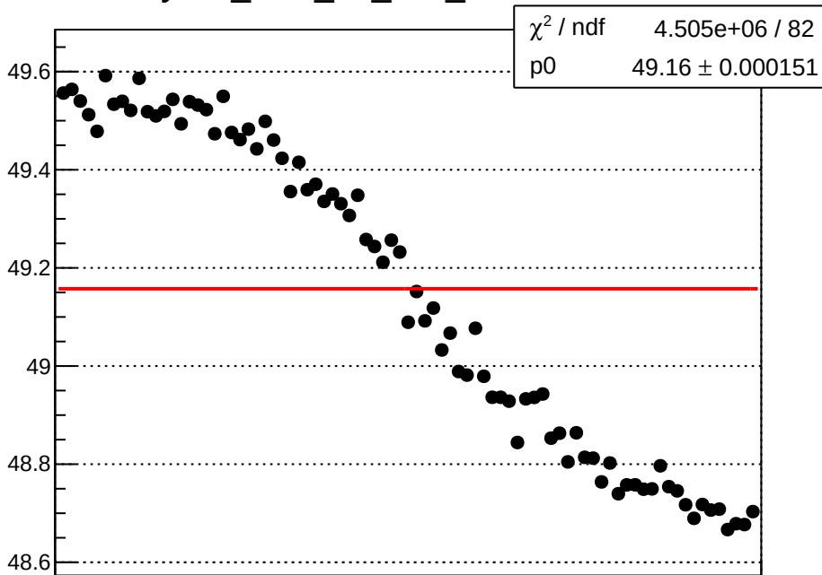
yield_bcm_an_ds3_mean vs run
