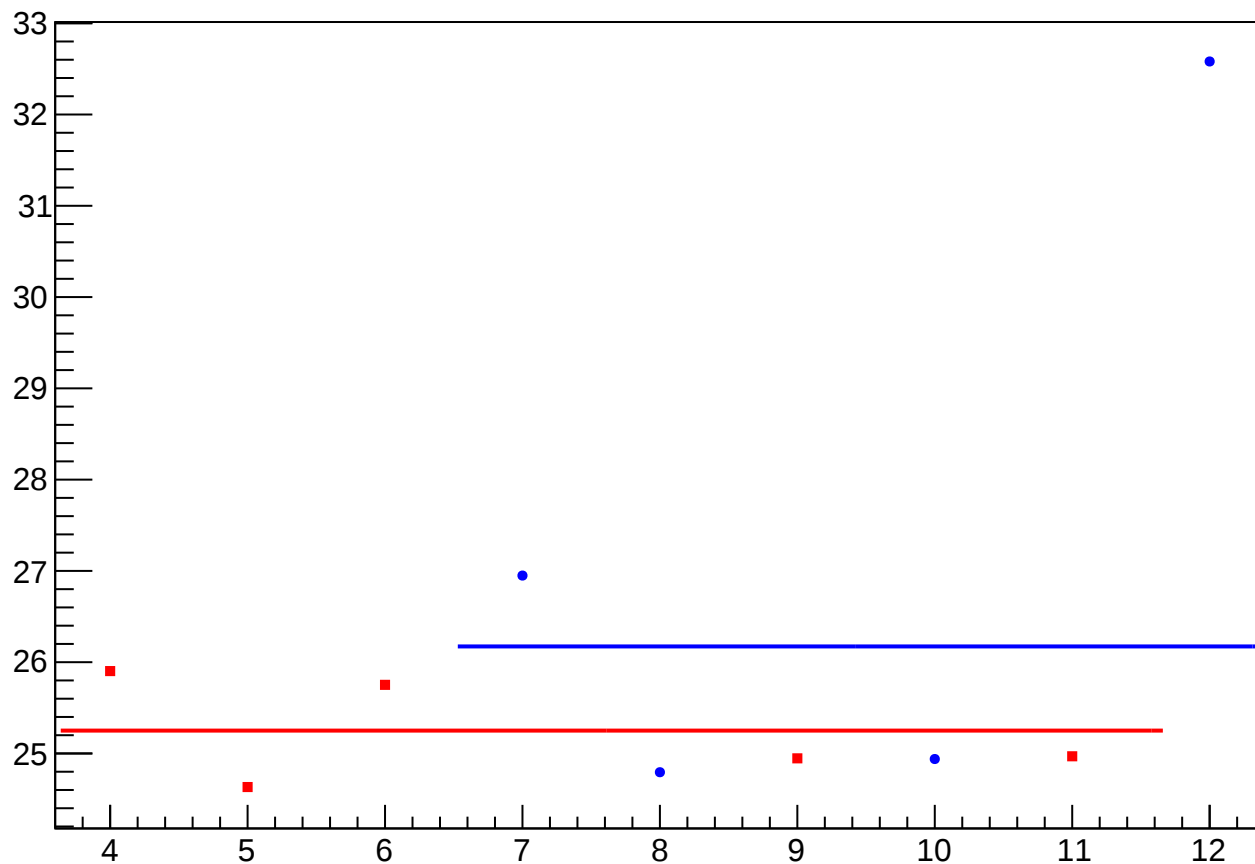
asym_bcm_dg_us_bcm_an_ds_agg_dd_rms vs slug
