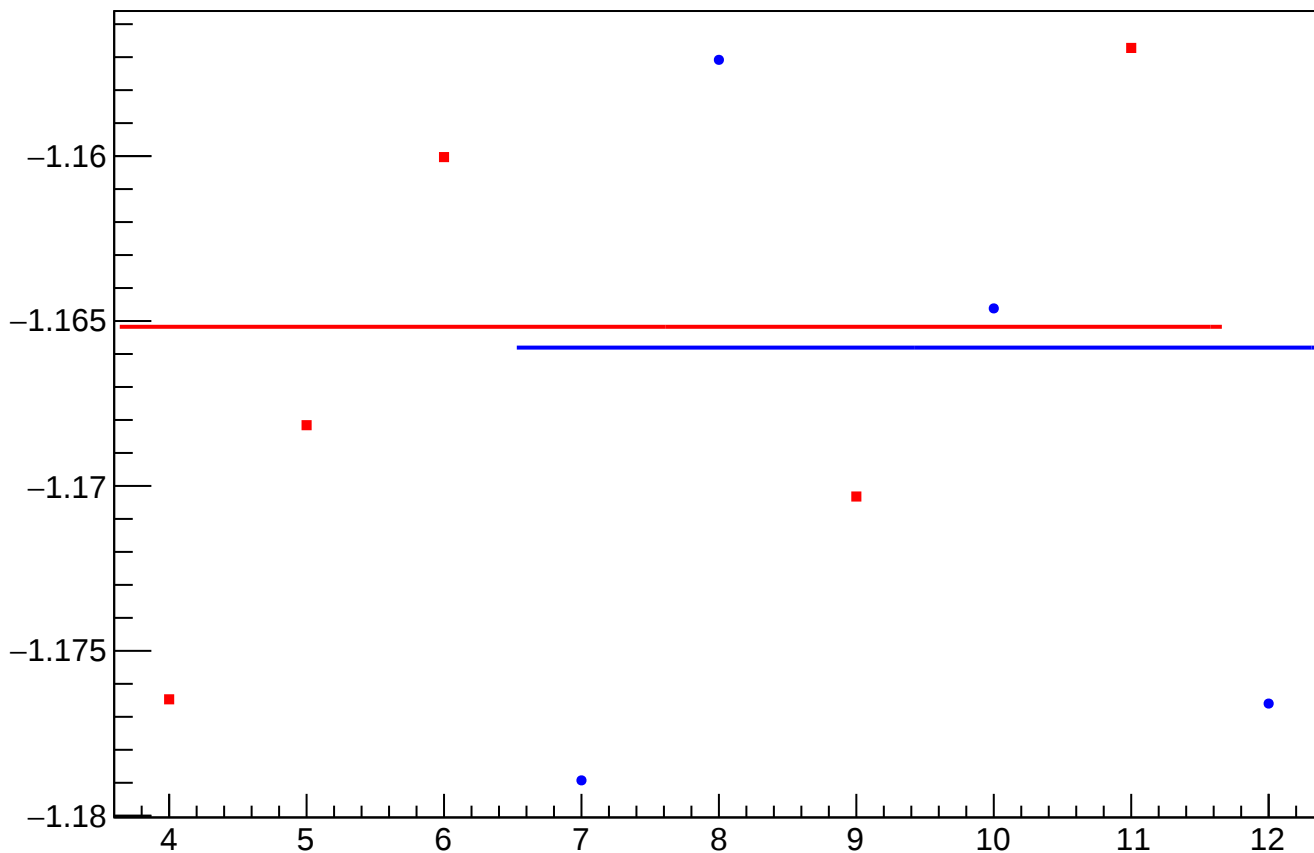
yield_bpm2i01X_mean vs slug
