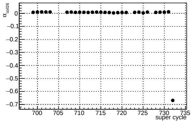
\alpha_{\text{coil26}} slug12
