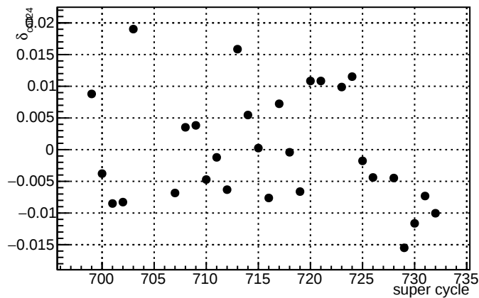
\delta_{\text{coil24}}
