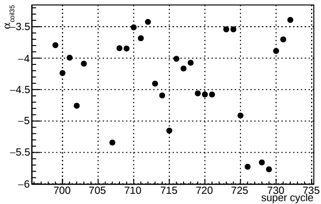
\alpha_{\text{coil35}} - \text{slug12}
