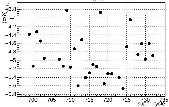
(\delta/\alpha)_{\text{coil15}}
