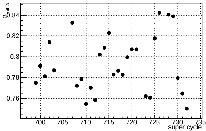
\alpha_{\text{coil13}} slug12
