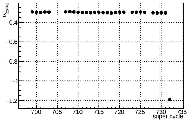
\alpha_{\text{coil46}} slug12
