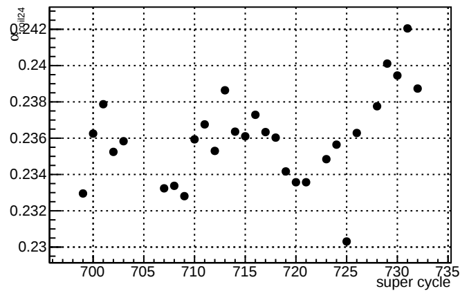
\alpha_{\text{coil24}} - \text{slug12}
