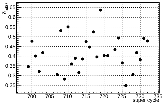
\delta_{\text{coil15}}
