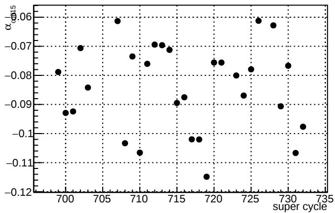
\alpha_{\text{coil15}} slug12
