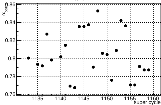
\alpha_{\text{coil13}} - \text{slug21}
