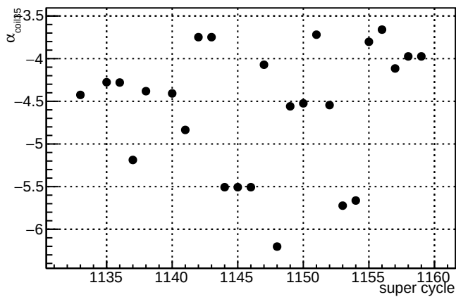
\alpha_{\text{coil35}} - \text{slug21}
