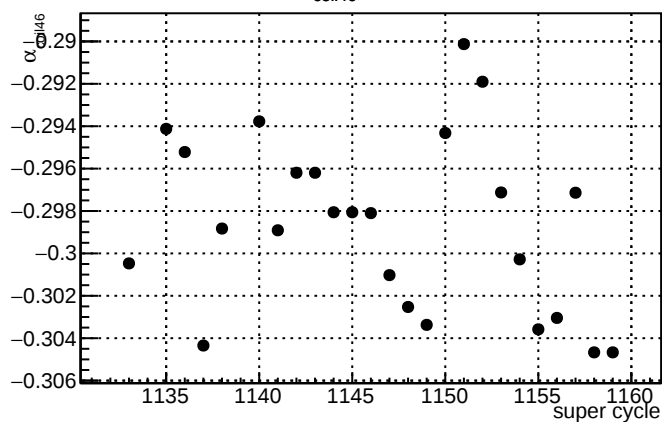
\alpha_{\text{coil46}} - \text{slug21}
