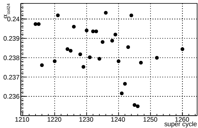
\alpha_{\text{coil24}} - \text{slug24}
