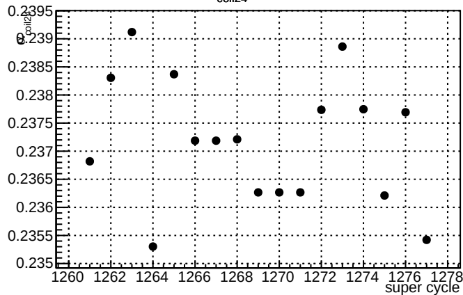
\alpha_{\text{coil24}} - \text{slug25}
