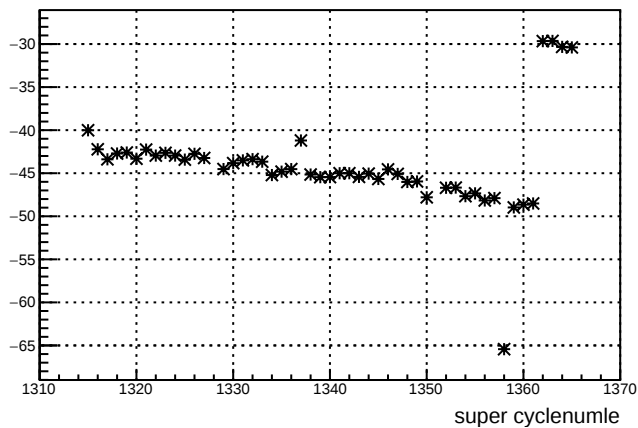
usr_11X12X : slug 27
