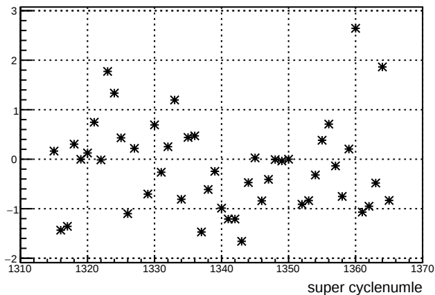
dd_ds_4ey : slug 27
