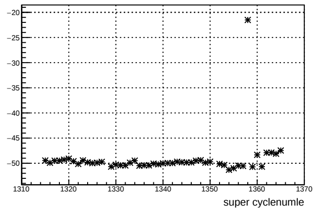
dd_ds_4ey : slug 27
