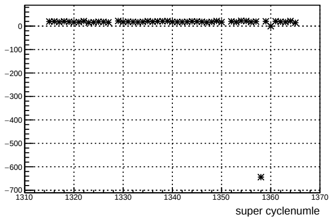
dd_ds_4ay : slug 27
