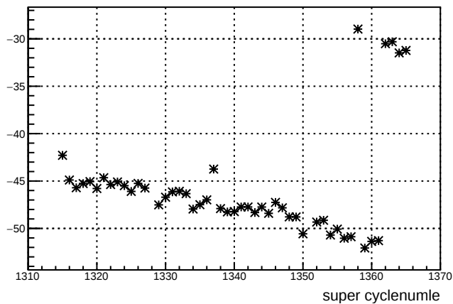
avg_ds_11X12X : slug 27
