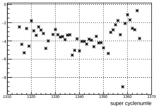
usr_11X12X : slug 27
