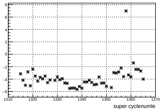
avg_ds_11X12X : slug 27
