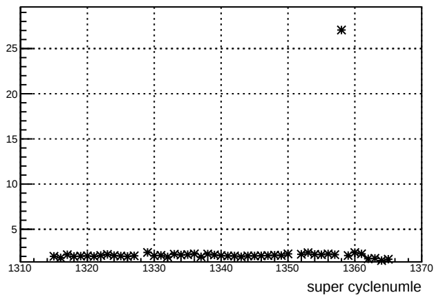
dd_ds_11X12X : slug 27
