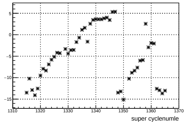
avg_us_4ey : slug 27
