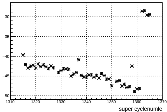
avg_us_11X12X : slug 27
