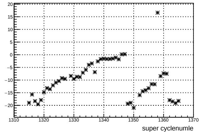
avg_ds_4ey : slug 27
