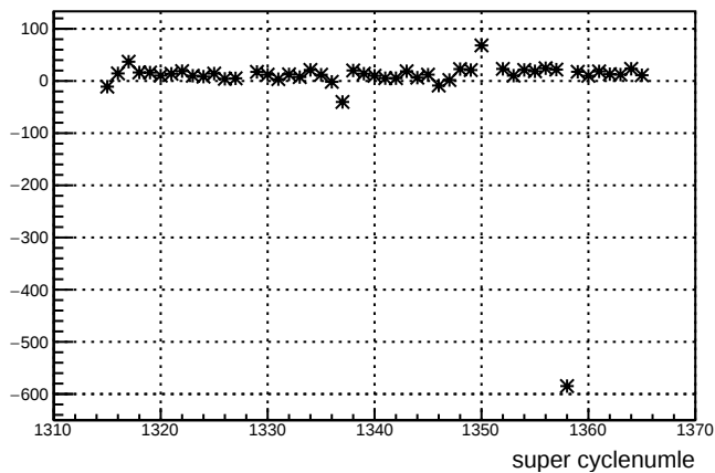
avg_ds_4ay : slug 27
