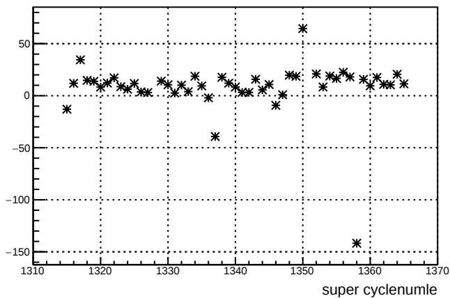
avg_us_4ay : slug 27
