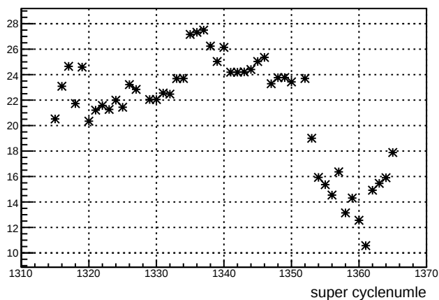
avg_us_4ey : slug 27
