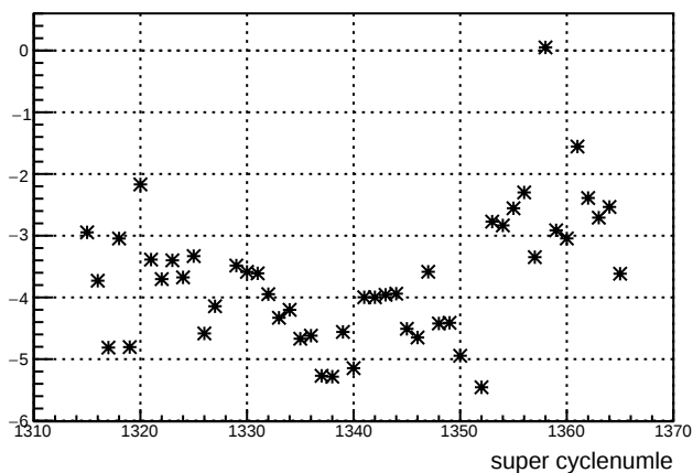
avg_us_11X12X : slug 27
