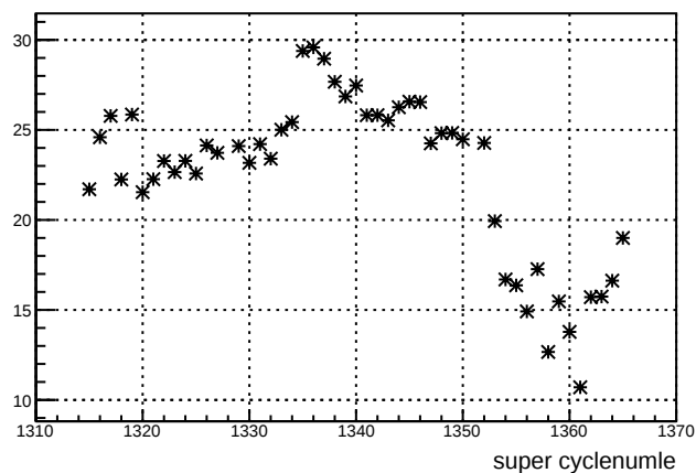
avg_ds_4ey : slug 27
