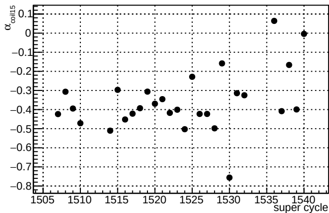
\alpha_{\text{coil15}} - \text{slug30}
