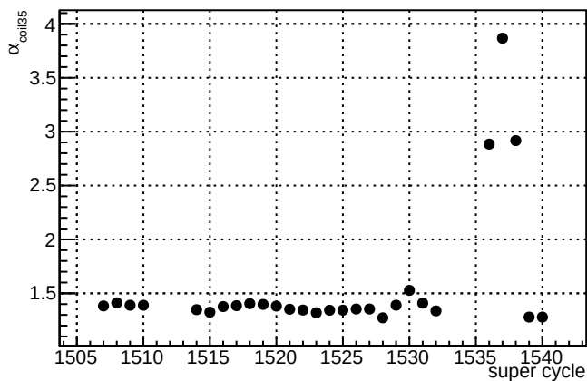
\alpha_{\text{coil35}} - \text{slug30}
