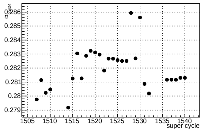
\alpha_{\text{coil24}} - \text{slug30}
